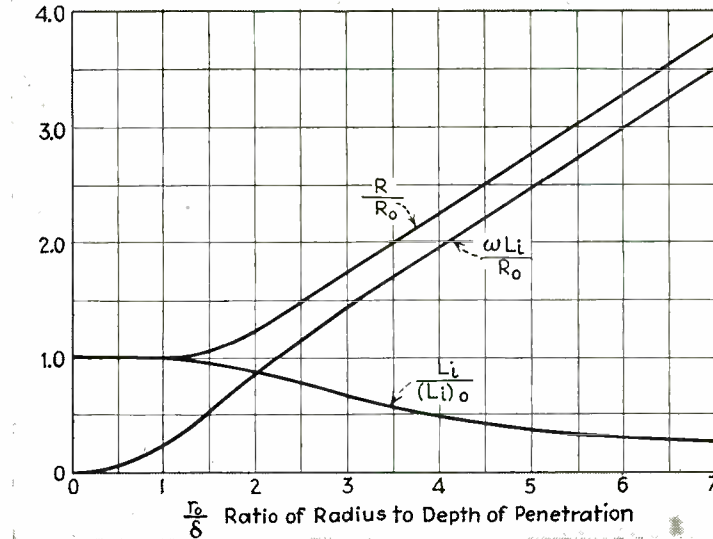
Fig. 2—Solid round wire. Skin effect quantities compared to d-c values. R_o = d-c resistance of round wire; L_i = internal inductance; R = true resistance of round wire; (L_i)_o = internal inductance at very low frequencies
