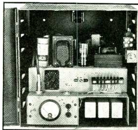
Fig. 7—Holmes a-c amplifier, band-pass filter and power supply unit. (Photo-tube detector "head", not illustrated, is mounted few feet away.) Plug at lower left may be removed and inserted in jack few inches to right to test performance of system without a-f filter. One of three relays visible at lower right may be tripped from remote office to extinguish lightsource and check system performance
