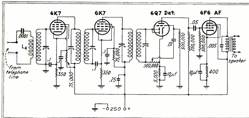
Fig. 2—Carrier-current receiver
