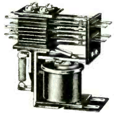
TYPE "F" RELAY Small, compact Relay for 1, 2, 3 or 4 Poles: Single Throw or Double Throw. Dimensions: 2 1/2" High, 2 1/2" Long, 1 1/2" Wide.
