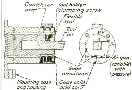
Location of the electrical aids with respect to the tool bits as they cut into the metal of the workpiece
