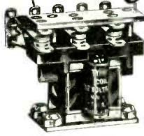
TYPE "J" RELAY Small, compact, with extra power for small size. 2 or 3 pole. Contacts have self-cleaning "wiping" action. Designed to meet the rigid temperature, humidity and vibration specifications established for military and naval aircraft.
