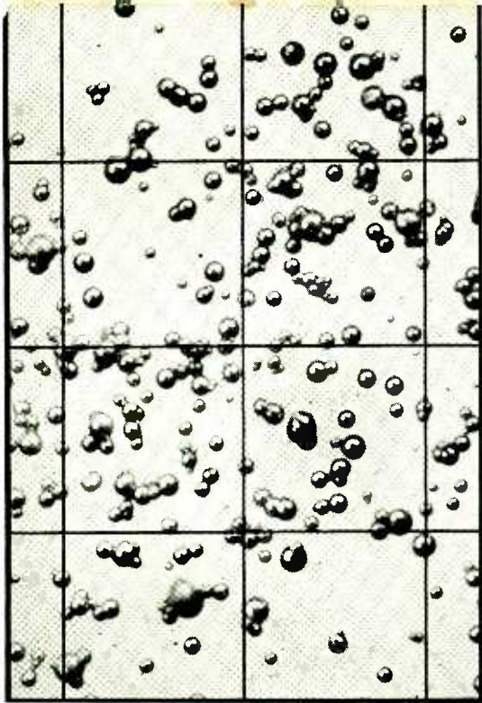
powder used for communication circuits. Magnification 515X
