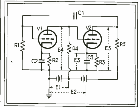
Fig. 1—Essential circuit of the 10-Mc oscilloscope which uses a high vacuum tube as sweep frequency generator in place of the usual gas tube
