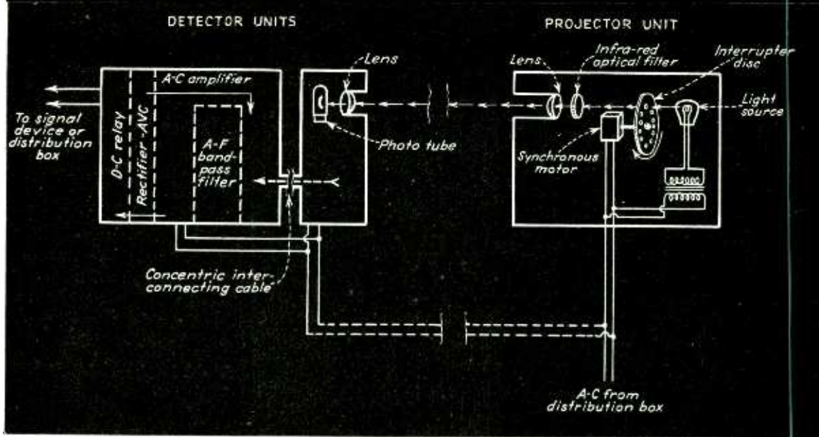
Fig. 5—Block diagram of typical modulated-beam photoelectric alarm system. Beam-throw distances of 1000 feet or more are proving practical with such systems, outdoors as well as indoors
