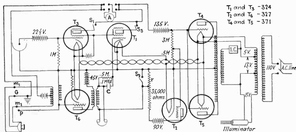
Fig. 4—Use of microphone to start timing mechanism for races. A phototube marks the instant the end line is crossed
