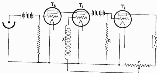
Fig. 2—A phototube may be used to supply the impulse that starts the timer
