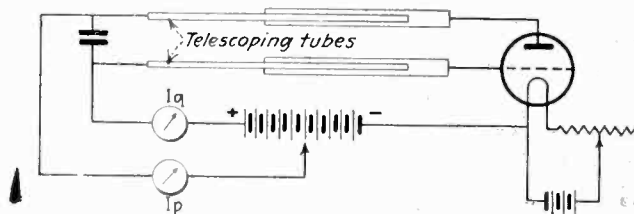
Fig. 2—Gill and Morrell's oscillating circuit. The frequency could be varied by the telescoping tubes
