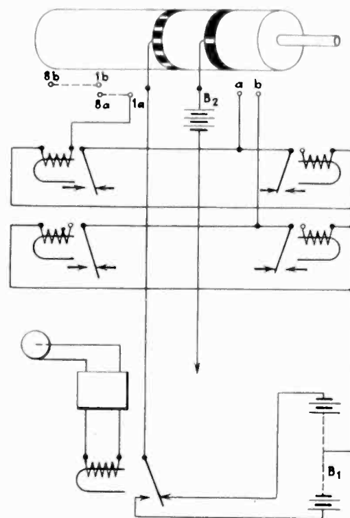
Phototube apparatus for punching design into Jacquard cards for weaving
