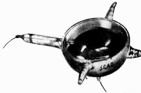
Hemispherical photoelectric cell of L. Dunoyer
