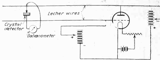
Fig. 1—Ultra-high frequency oscillator of Barkhausen and Kurz, in which the voltages determined the frequency. Wave length was measured by moving the crystal detector along the Lecher wires
