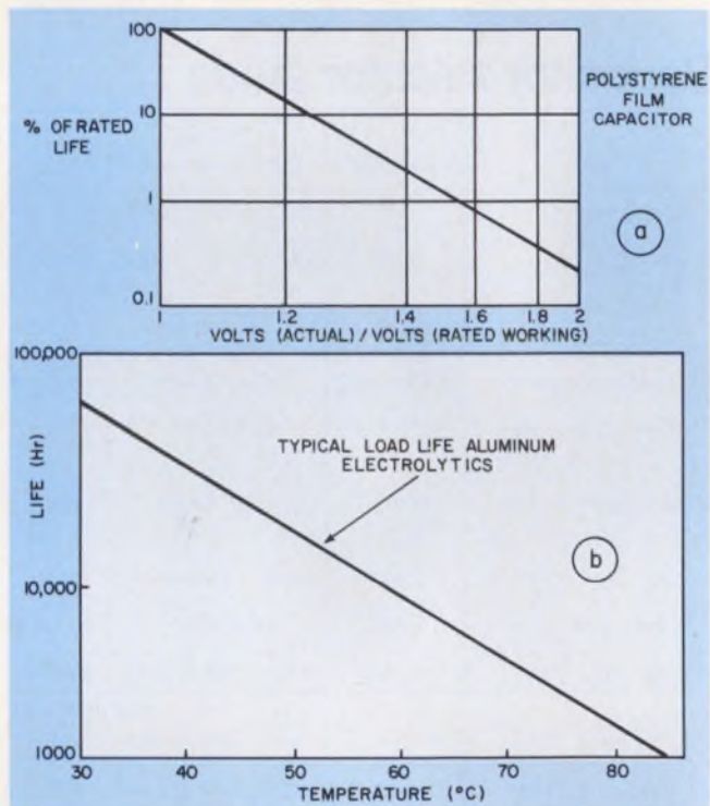
4. Capacitor life drops rapidly with both overvoltage (a) and temperature increase (b).
