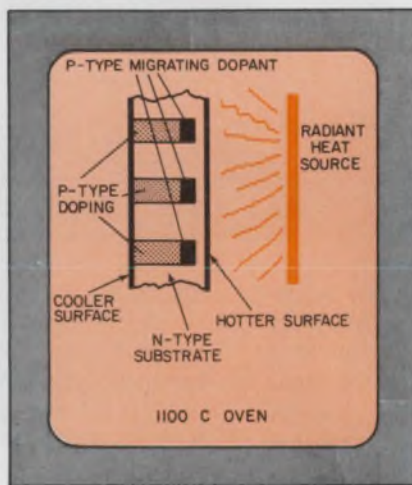
Since one side of the slice is hotter, dopant is drawn through faster, which should cut semi costs.
