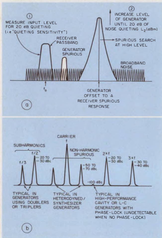
5. A generator's spurious components directly affect the measurement of receiver spurious attenuation (a). Any one of a variety of unwanted generator outputs can complicate the measurement (b).
