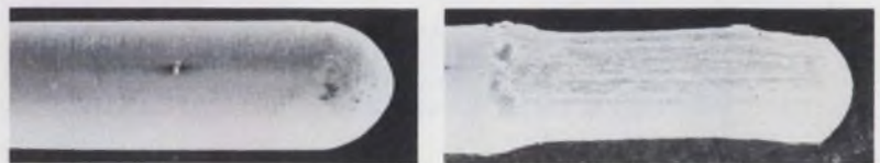
Dramatic difference in wear between contacts utilizing the unique AMP Bonded Lubrication Process and ordinary contacts is shown by these electron images.
