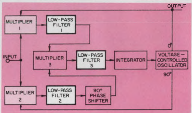
2. Theoretically, three low-pass filters are needed in an FLL that uses digital multipliers at its input.
