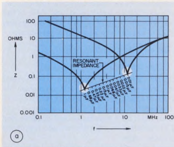
2. The impedance of a capacitor shows the resonance dip of a series-tuned circuit. Typical curves for polycarbonate (a) and polyethylene-film (b) capacitors display the dip.
