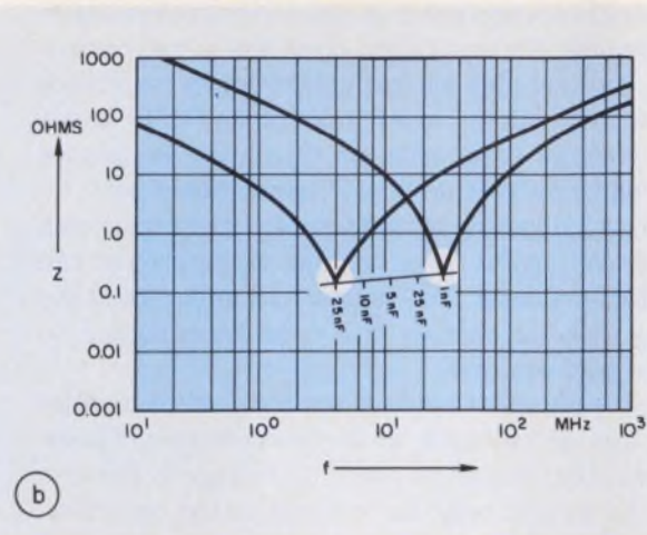
At frequencies past the dip, the capacitor has the reactance of an inductance, which increases with frequency and can disrupt circuit performance.
