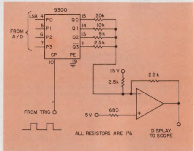
12. A two's complement, four-bit d/a converter provides \pm 5 -V analog excursions for the scope display. The screen amplitude doesn't depend on the a/d under test.
