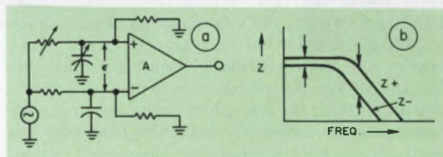
5. Input imbalance results from unequal electrode impedances or unequal capacitances to ground (a). The impedances are frequency-dependent, of course (b).
