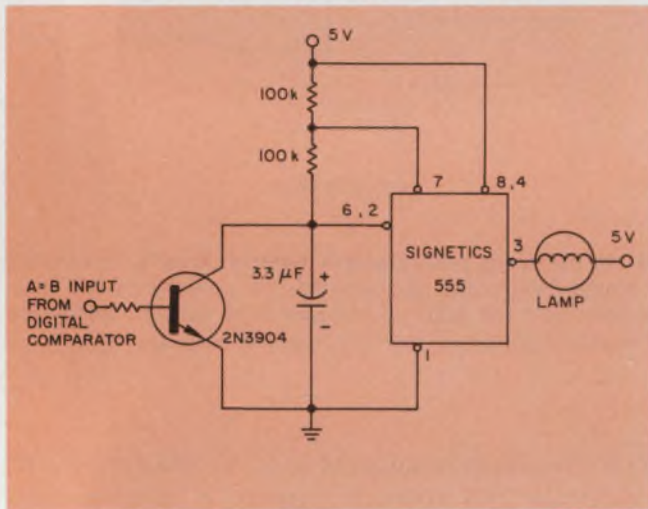
11. Missing codes are indicated when the 2N3904 is cut off and the 555 timer, acting as a multivibrator, blinks the lamp at about three flashes per second.
