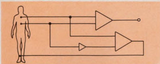
10. To cut common-mode noise, you can detect the unwanted signal, then vary a reference signal—usually derived from the right leg—at the same rate as the noise. The differential amplifier thus “sees” no common mode at its front end.
