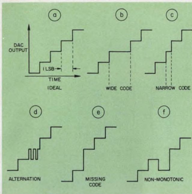
5. Various displays depict uniform excursions of an ideal a/d (a), wide and narrow codes (b and c), alternations (d), missing codes (e) and nonmonotonicity (f).
