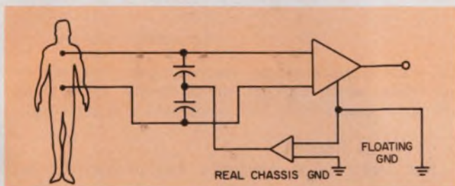
11. Still another way to discard a common-mode signal: Drive the junction of two capacitors with a signal 180-degrees out of phase with the noise.
