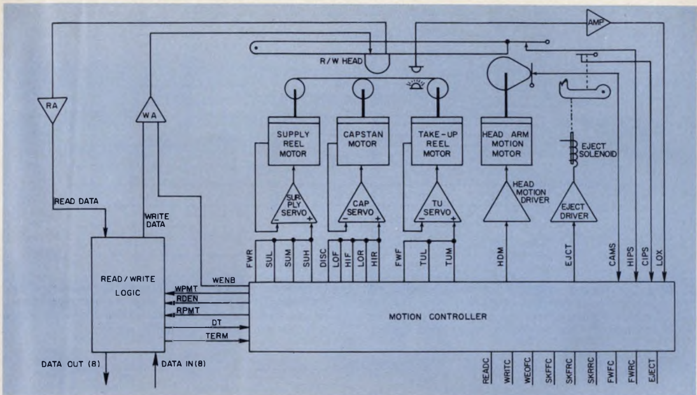
1. A cassette-tape drive system uses a programmable controller consisting of read-only memory and an MSI-
