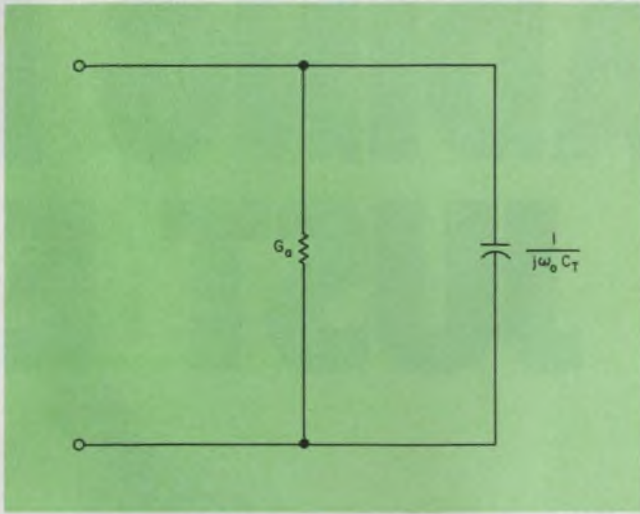
4. A surface-wave transducer can be represented by this equivalent circuit.
