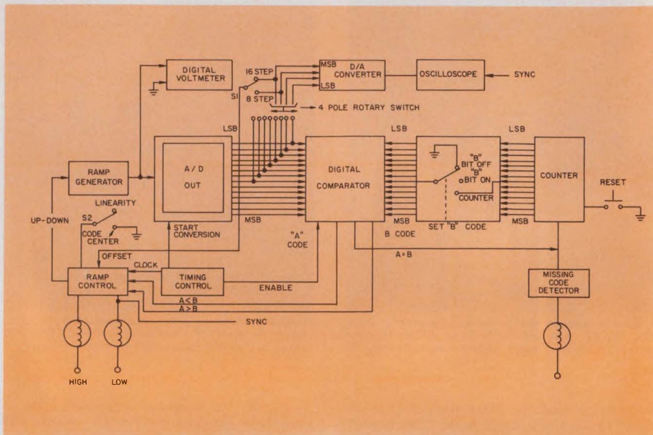
7. The complete a/d converter tester, with all additions and modifications, can determine converter errors in several ways. Code centers are measured with the digital
