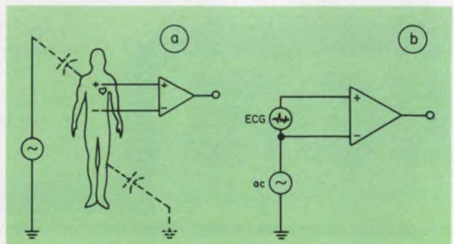
3. A biomedical signal, such as ECG, is differential (a), while the unwanted 60 Hz appears as common mode (b).
