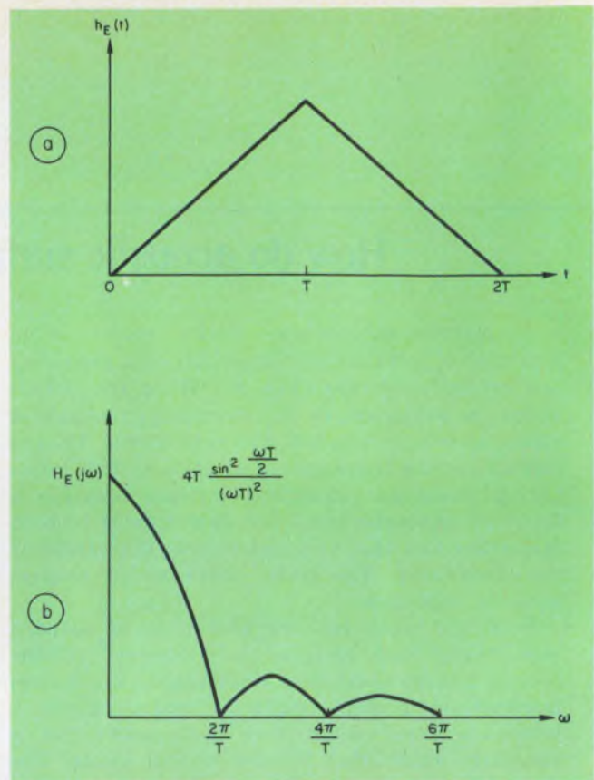
2. The over-all delay line has a triangular impulse response (a). The corresponding spectrum exhibits the characteristic of a matched filter with a 1/T bit rate.
