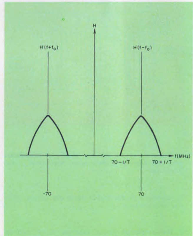
3. The first null-to-null bandwidth affects the length of the quartz and number of lines.
