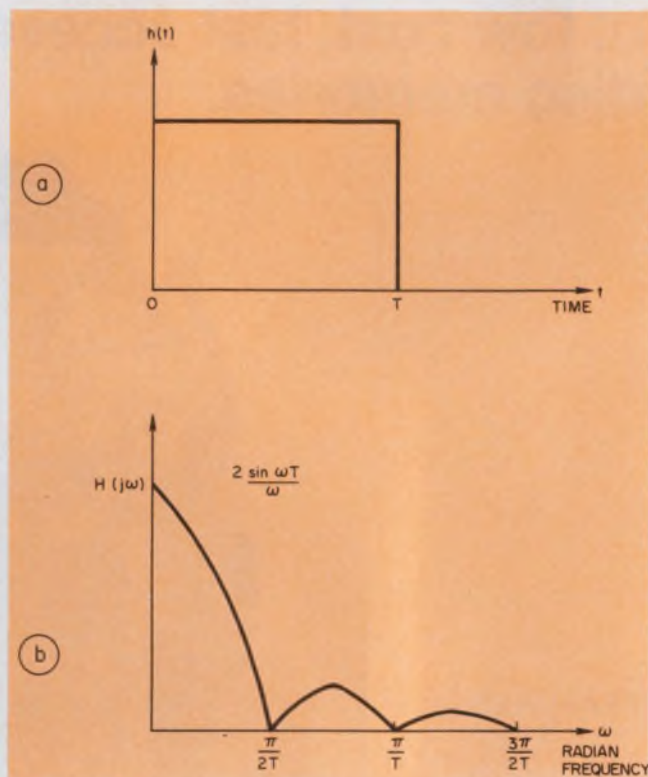
1. Assume each transducer has an impulse response (a). As a result, the corresponding spectrum has a (\sin x)/x type of variation (b).
