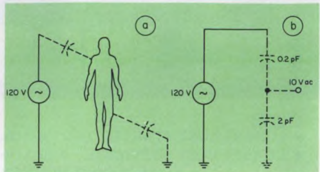
1. Capacitive coupling to surrounding power sources and grounds (a) causes the human body to appear electrically as a 60-Hz noise source (b).
