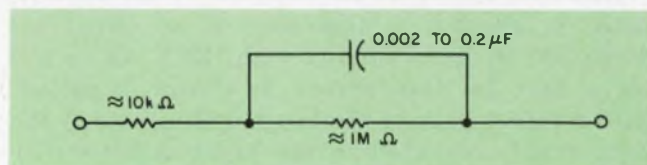
6. An equivalent circuit of the skin's contact impedance accounts for tissue and fluid resistance and capacitance.
