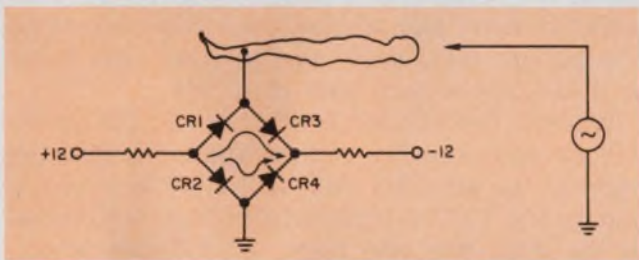
12. With a diode bridge, you can safely ground a patient to eliminate common-mode voltages. The bridge prevents a direct path to ground if the patient inadvertently touches a power supply.
