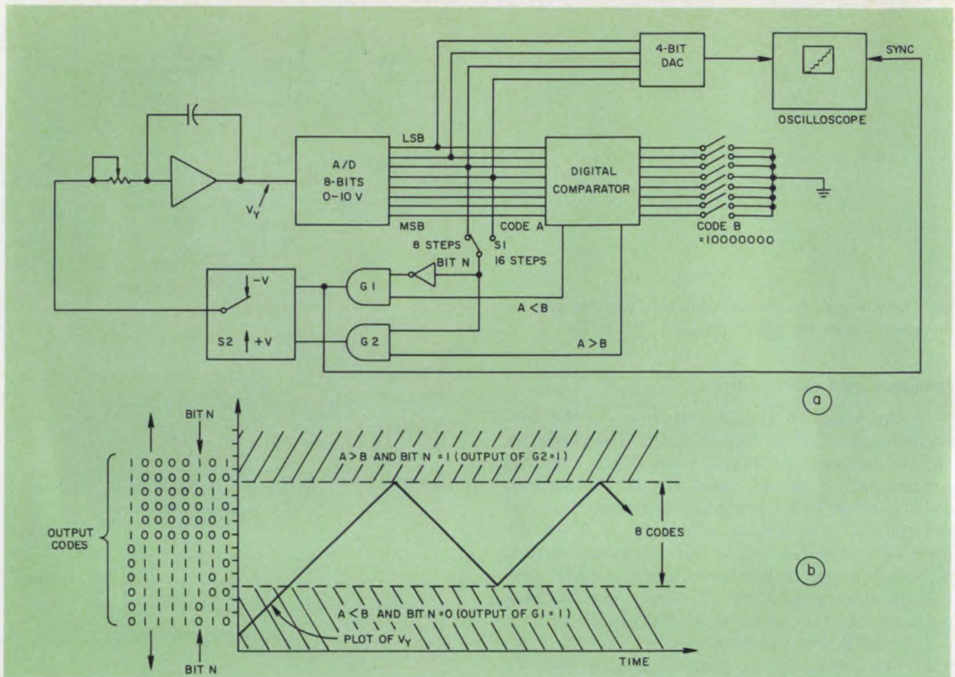
4. Local linearity can be displayed by modification of the feedback and comparator sections (a). With S_1 set to
