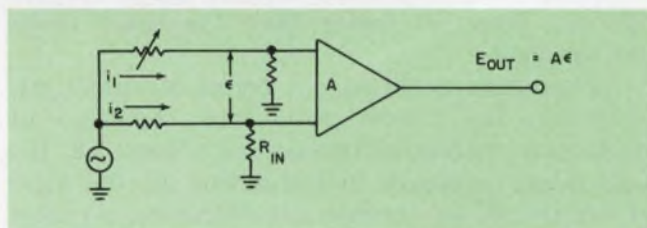
4. Unbalanced impedances in the two input legs of the amplifier cause unequal currents to flow into each leg. As a result, a portion of the common-mode noise is converted to a differential signal, which is then amplified and delivered at the output.
