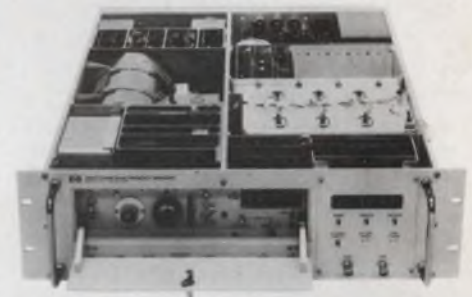
Remove the lid and you'll see the sturdy construction that enabled the 5062C Cesium Standard to pass the grueling 400-lb hammer blow test.
