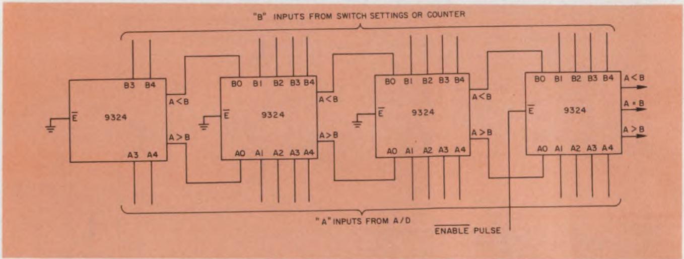
10. Four 5-bit comparators are connected to form the 14-bit digital circuit that compares the converter's out-
