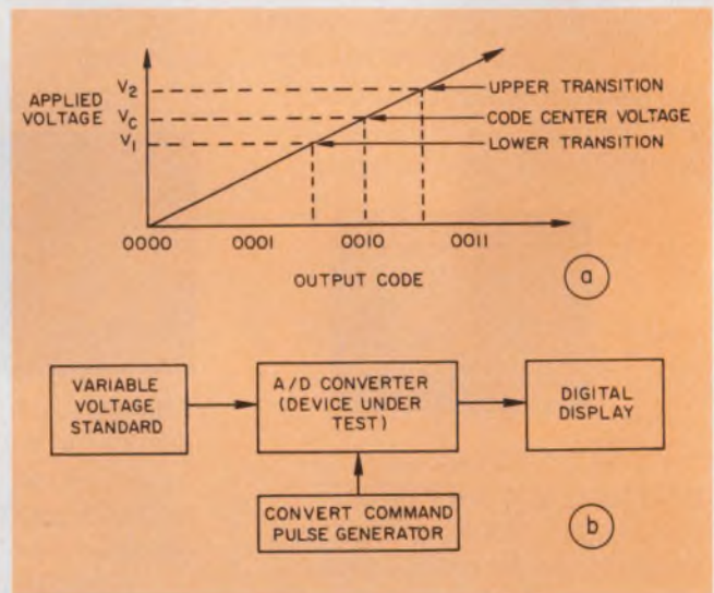
1. To check an a/d-converter's static transfer function—output codes vs input levels (a)—the user varies the input voltage and looks at the displayed code (b). Such a test provides limited performance data, however.
