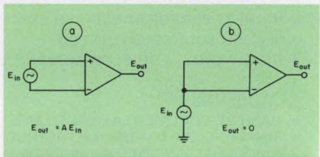
2. To extract minute biomedical signals and simultaneously discard the 60-Hz noise, the signal is first applied to a differential amplifier (a). An ideal differential amplifier shows no output when the same signal, called the common mode, is applied to both input terminals (b).
