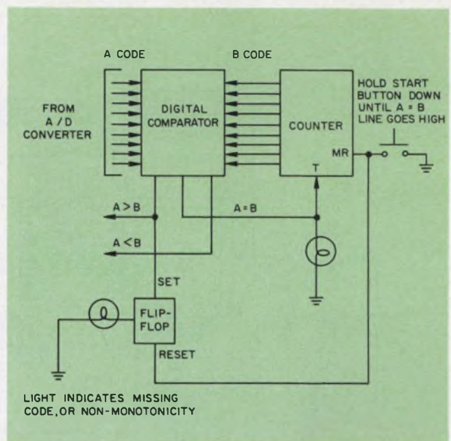
6. Missing codes are automatically searched out with a counter in place of the manual switches. Nonmonotonicity is also determined and indicated.
