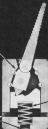
T8000 SERIES PCB TOGGLE SWITCH
