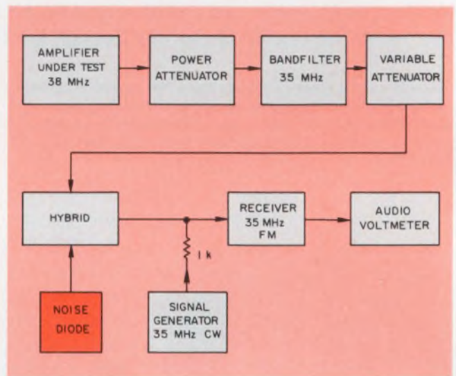
1. To characterize transmitter noise, a receiver can be used in a transfer setup to indirectly compare the transmitter's output with that of a noise diode.
