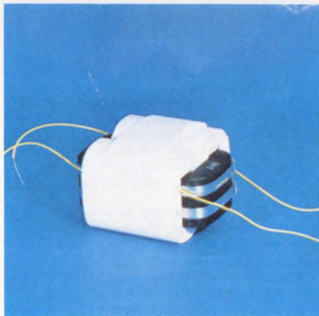
Output pulses with amplitudes of 3000 V and widths of between 10 and 100 \mu s are possible with this 500-W pulse transformer from Velonex.
