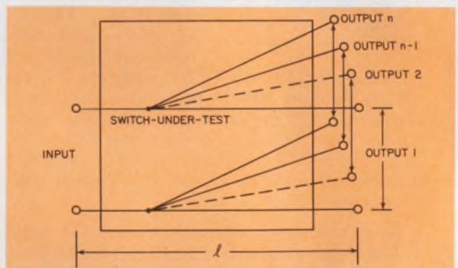
2. Insertion phase is the phase difference (horizontal axis) from the input to outputs 1 through n. The measurement assumes zero electrical length between the ports. Phase differential gives insertion phase between outputs.
