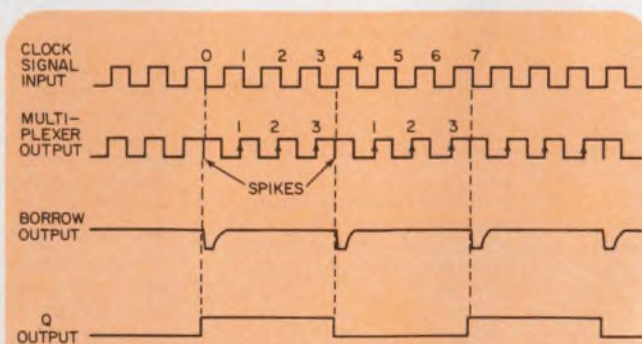
2. Timing diagram of a divide-by-7 sequence shows how the counter input is reduced by one count for every half cycle for odd values of n . This is because the phase of the input signal is reversed every half cycle. The counter registers only on rising edges.
