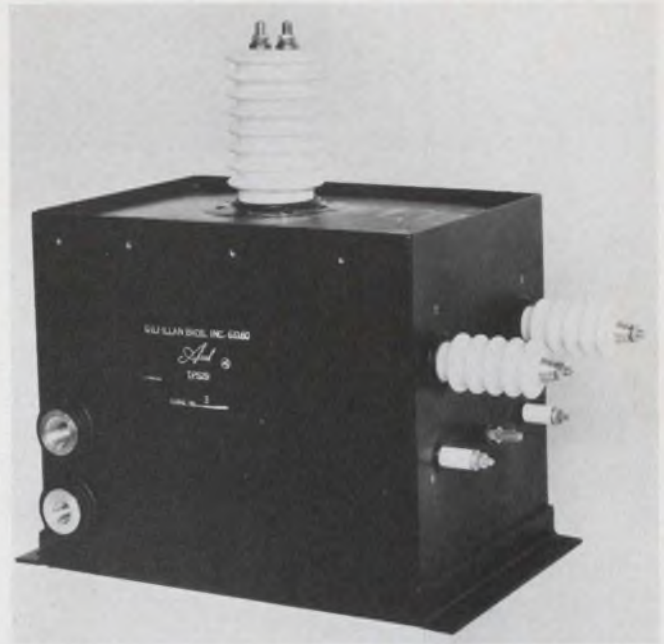
Large pulse transformers for matching the voltage and impedance of pulse-forming networks to microwave tubes, such as this one from Axel, often contain a filament transformer too.
