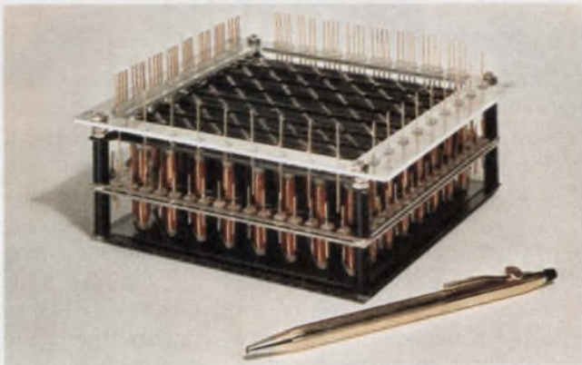
A workhorse for circuit switching , the reed memory matrix, consumes little power, yet handles signals from dc to video frequencies. This Mini Memory Matrix from C. P. Clare switches eight rows by eight columns with four contacts per crosspoint. The electronic control can be a mini or microprocessor.
