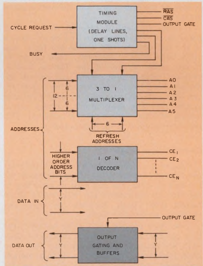
3. Interface circuitry for a memory system assumes the use of Mostek's 4-k dynamic RAM, the MK4096.
