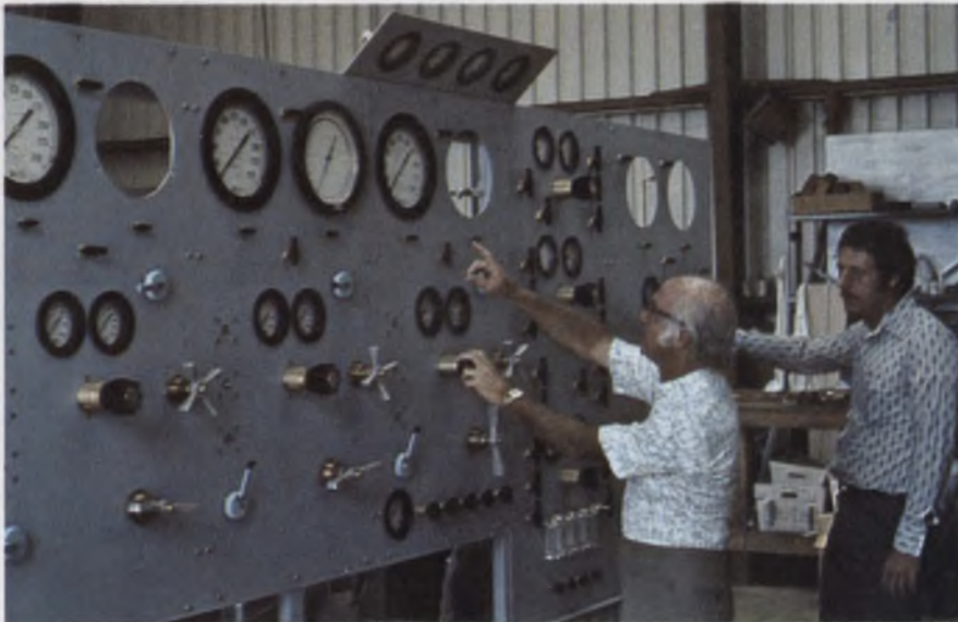
Control console, built by Perry, is used on the offshore platform or on board ship over a submerged well to monitor the diver saturation complex for diving bells and for the hyperbaric chamber on board ship.
