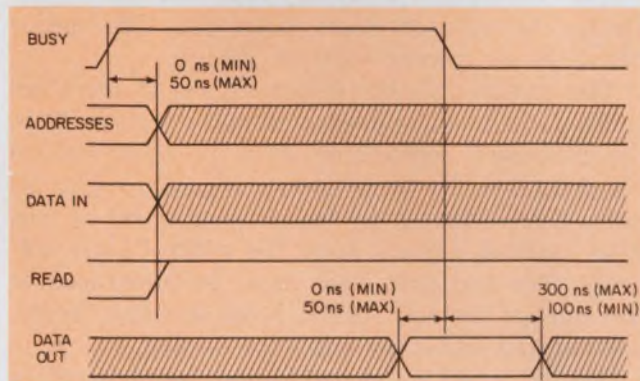
2. These control and data signals are sent back to the processor by the memory system.
