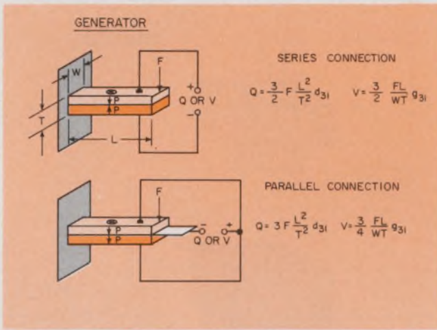
9. Series or parallel connections of transducer materials provide high outputs for small displacements.
