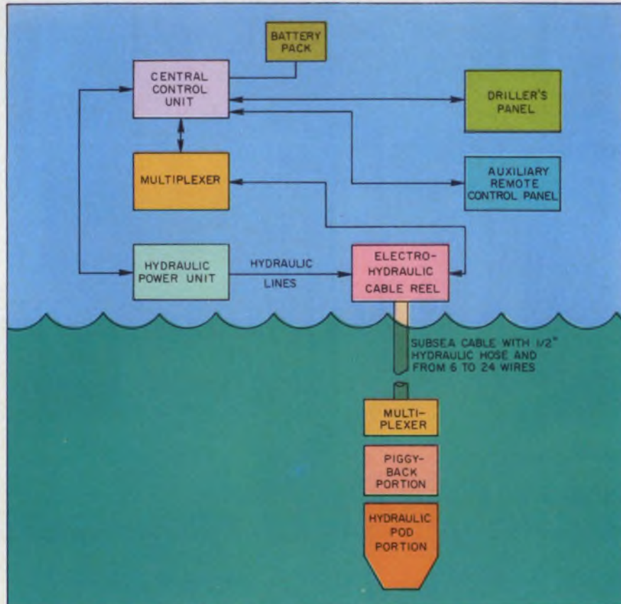
Koomey multiplex electro-hydraulic control system, by Stewart & Stevenson, is designed for deep producing wells. The multiplex cable sends signals to the underwater multiplexer, which instructs the hydraulic pod.
