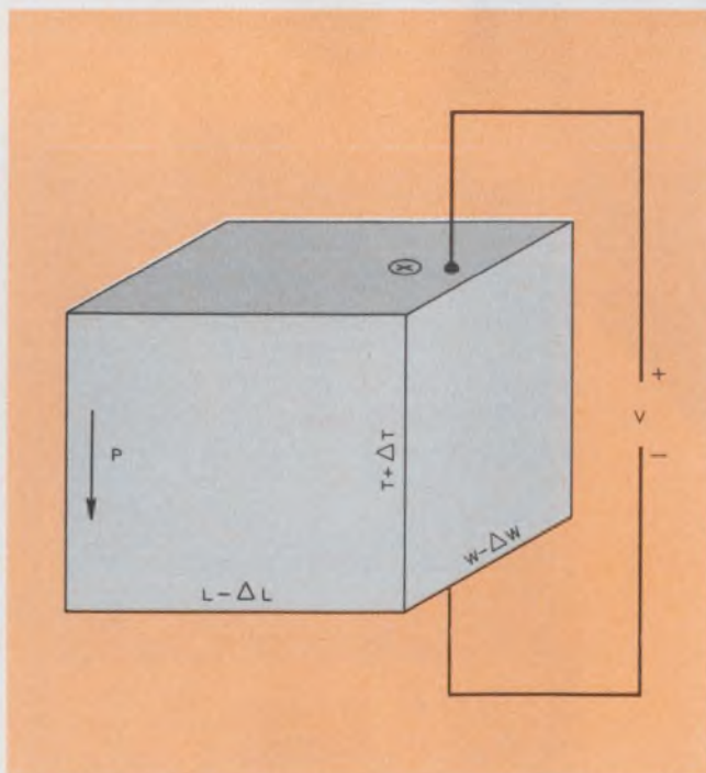
2. The electric fields required to pole the ceramic material are often as high as 100 V/mil.
