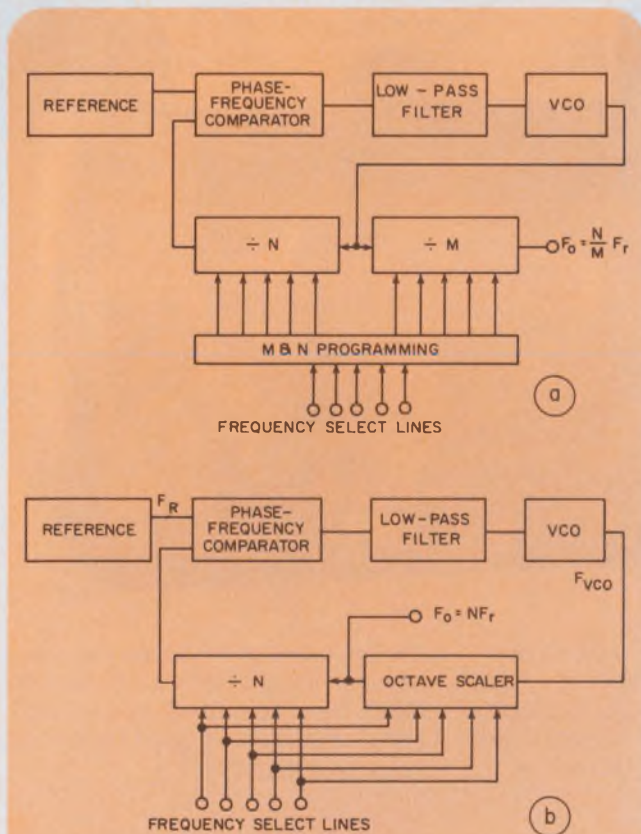
1. Conventional frequency multipliers (a) require selection of M and N. An improved version (b) requires selection of only N, and it reduces the VCO tuning range.
