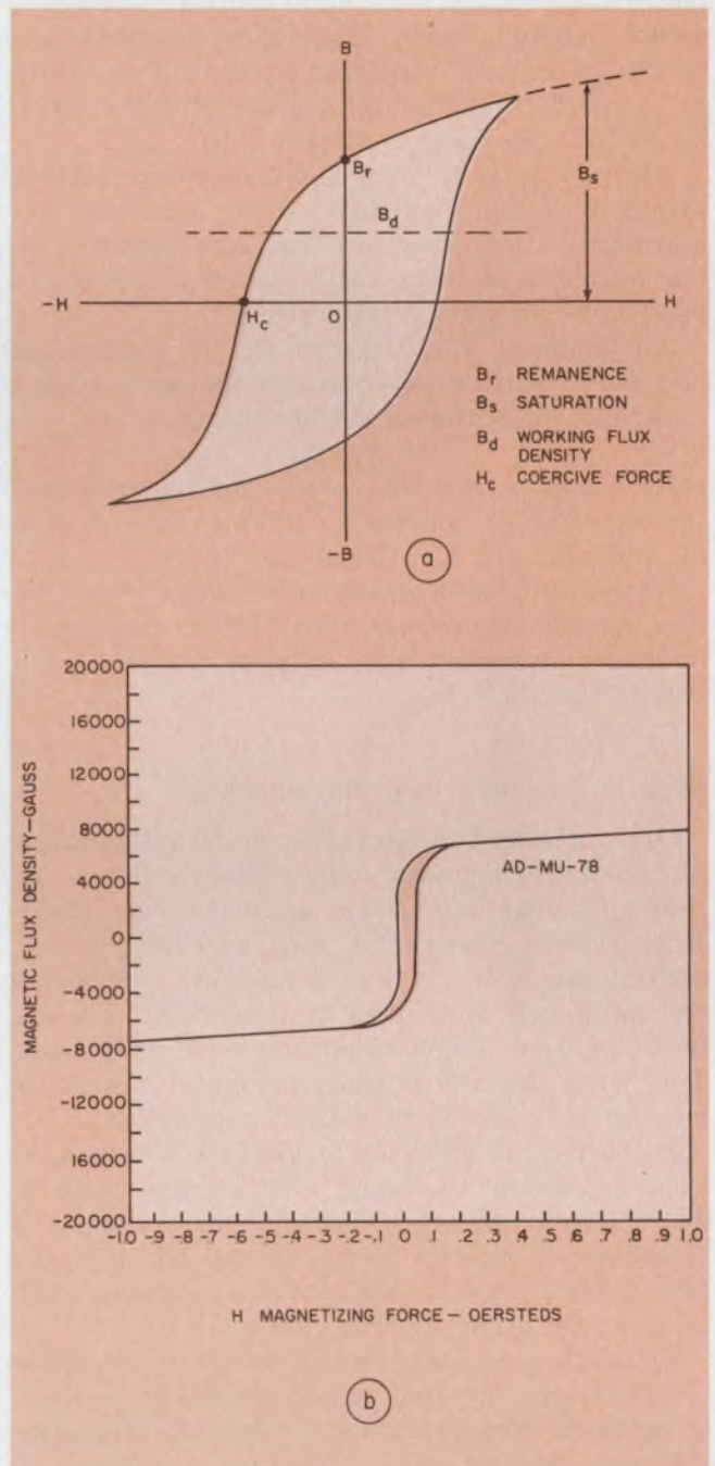
2. Permeability—the slope of a BH curve (a)—is not constant, contrary to the assumption in most mathematical analyses of magnetic systems. The BH curve of AD-MU-78, a high-permeability-alloy, is very steep, and it has an almost rectangular saturation point.
