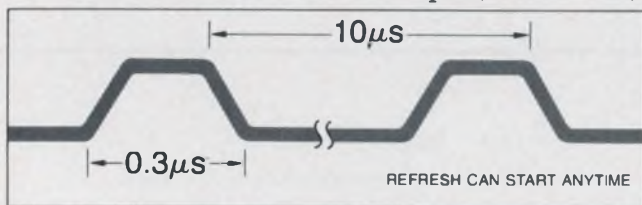
100 KHz TO 1 MHz INVISIBLE REFRESH SIGNAL
