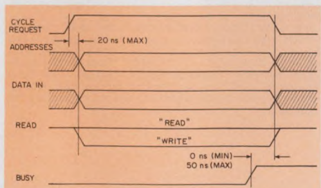
1. An asynchronous design begins with specification of the system interface signals to the memory system.
