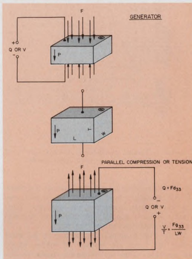
7. Direct generator applications make use of a charge output from the transducer under mechanical stress.
