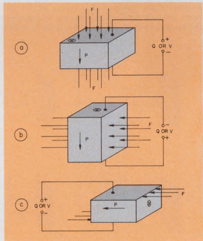
4. A polarized piece of ceramic has different characteristics when it is stressed in different directions.
