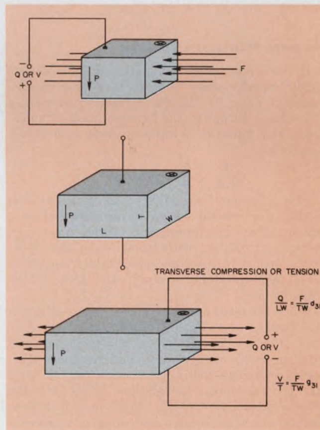
8. Forces applied perpendicular to the poling axis also produce usable electrical outputs.
