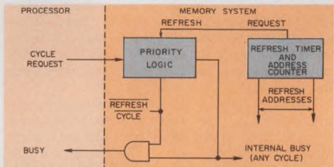
4. The controller section of an asynchronous design can include refresh-cycle interrupt logic needed for dynamic semiconductor memories.
