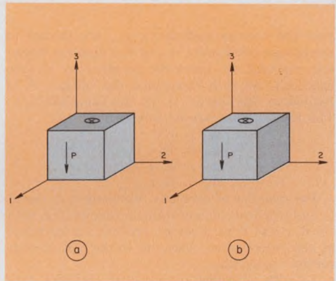
3. A unit cube of the ceramic material is set up as a three-dimensional solid for easy analysis.
