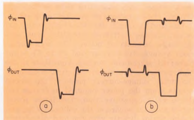
3. Typical clock noise problems consist of ringing (a) and crosstalk (b).
