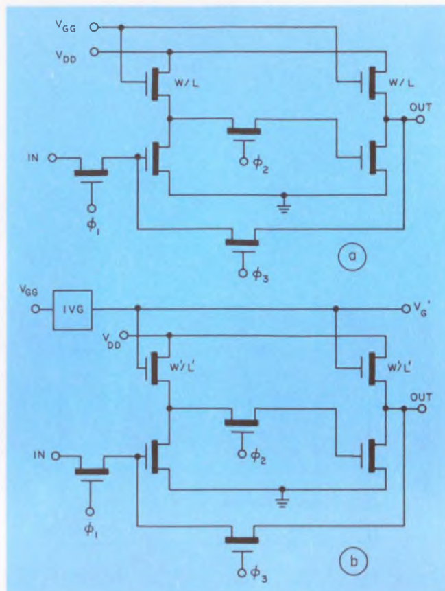
4. Power for a static shift register can be reduced, from that for a conventional design (a), with an IVG, or intermediate voltage generator (b).
