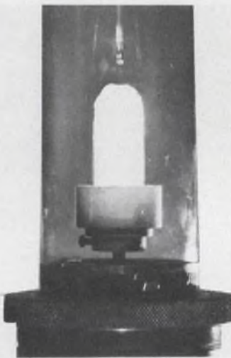
The top of the slug is melted by focused light. A seed crystal is then positioned above the molten cap (left), dipped into the cap (right) and then pulled slowly up to form a single crystal.
