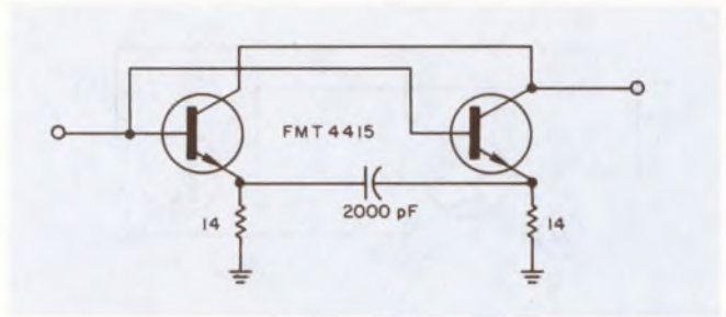
6. When two or more transistors are placed in parallel for a medium-power design, two equal emitter resistors are included for dc balance.
