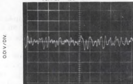
(b) - RESPONSE TO A 500\mu\text{C} STEP WITH CORRECT LOOP GAIN.
