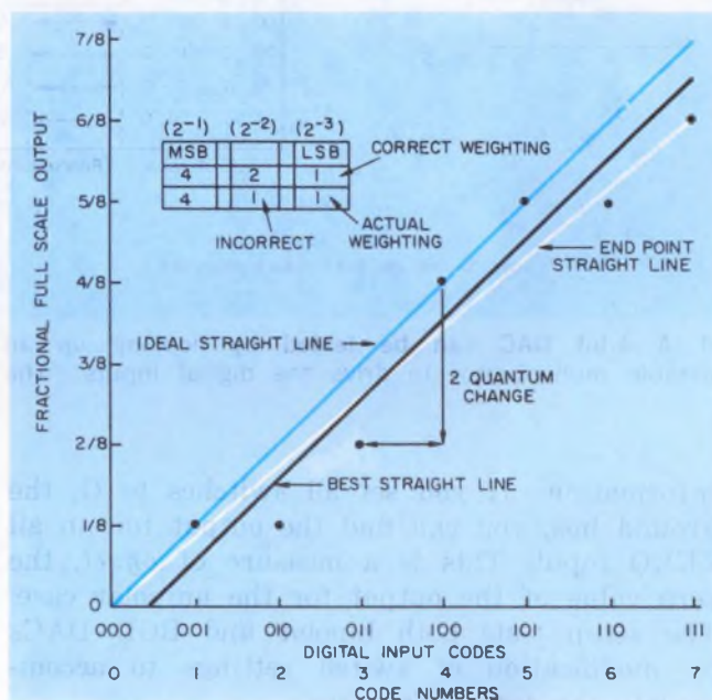
3. Deviations from the ideal linearity curve for a typical DAC can still stay within \pm 0.5 LSB if the best-straight-line is drawn through the points. The end-point-straight-line joins the zero and full scale values and thus passes through zero and the actual full scale.
