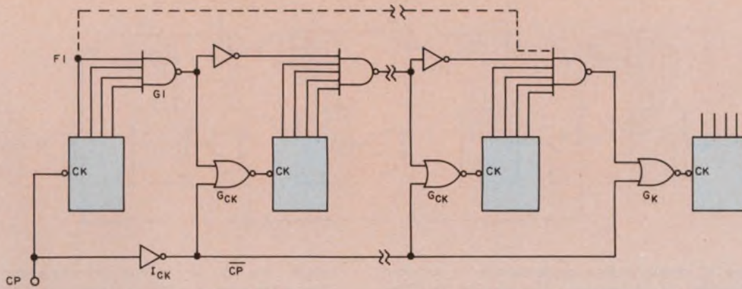
5. Greater clock speeds can be used if the clock-line is also enabled. Both the gate-inverter delay and the 1-to-0 transition delay of F_1 —at each clock pin—are elimi-
