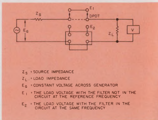
2. Accurate attenuation measurements below 1 MHz can be made using the method outlined in MIL-F-18327C.
