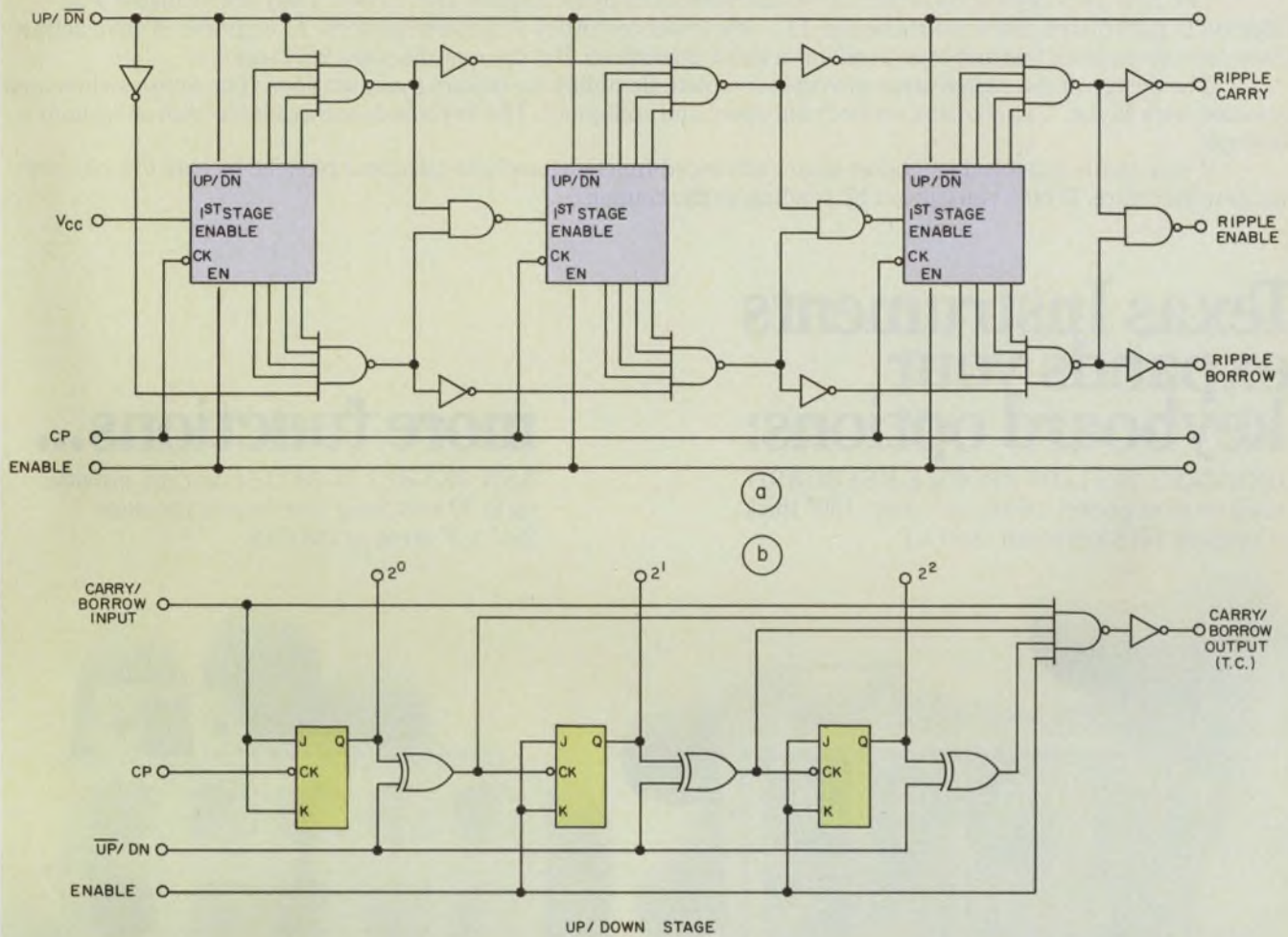
12. Circuits for the enabling of up/down counters are similar to those used with "up" counters. The main difference is that a second enable chain is used for the
