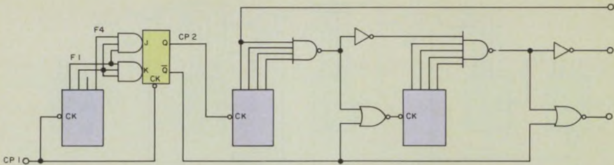
10. Secondary clock pulses should be tailored to the speed requirements of succeeding sections. The secondary clock pulse, taken from a ripple section, is modified in period and width.
