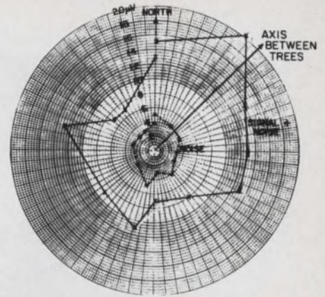
This directional pattern from two trees was obtained by controlling the phase of the energy fed them. Two Hemac couplers were used here.
