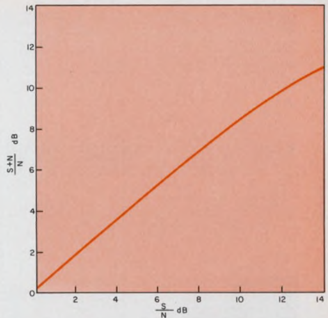
8. (S + N)/N to equivalent S/N ratio can be converted with this graph. Above about 10 dB, little error results if one is assumed equal to the other.
