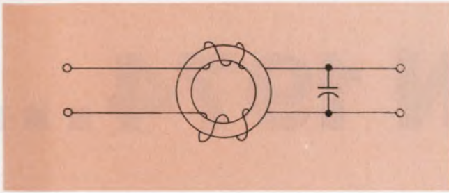
3. Common-mode interference can be reduced with a simple, "common-core" line-to-line filter.
