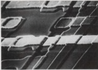
This is the surface of Hitachi's silicon-gate MOS chip for an 8-digit calculator with memory.
