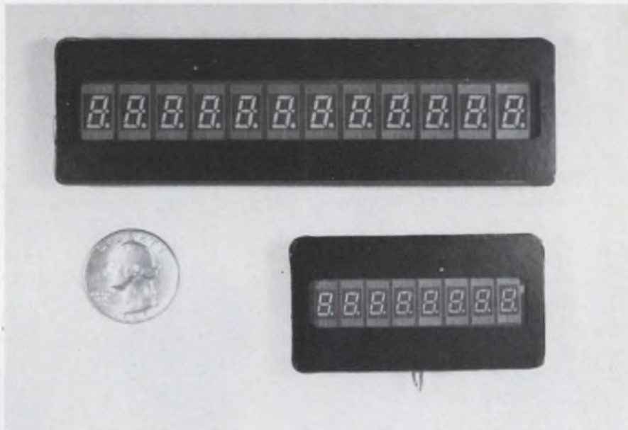
Multidigit fluorescent readouts from Ise Electronics lend themselves to easy multiplexing and provide a soft green glow.
