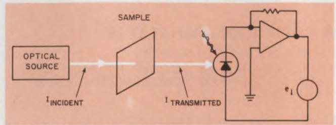
1. A conventional system can be used to make relative optical-transmission measurements without correction for component instability or drift. Typically a laser is used as the optical source and a photodiode with a FET-input operational amplifier as the detector system.
