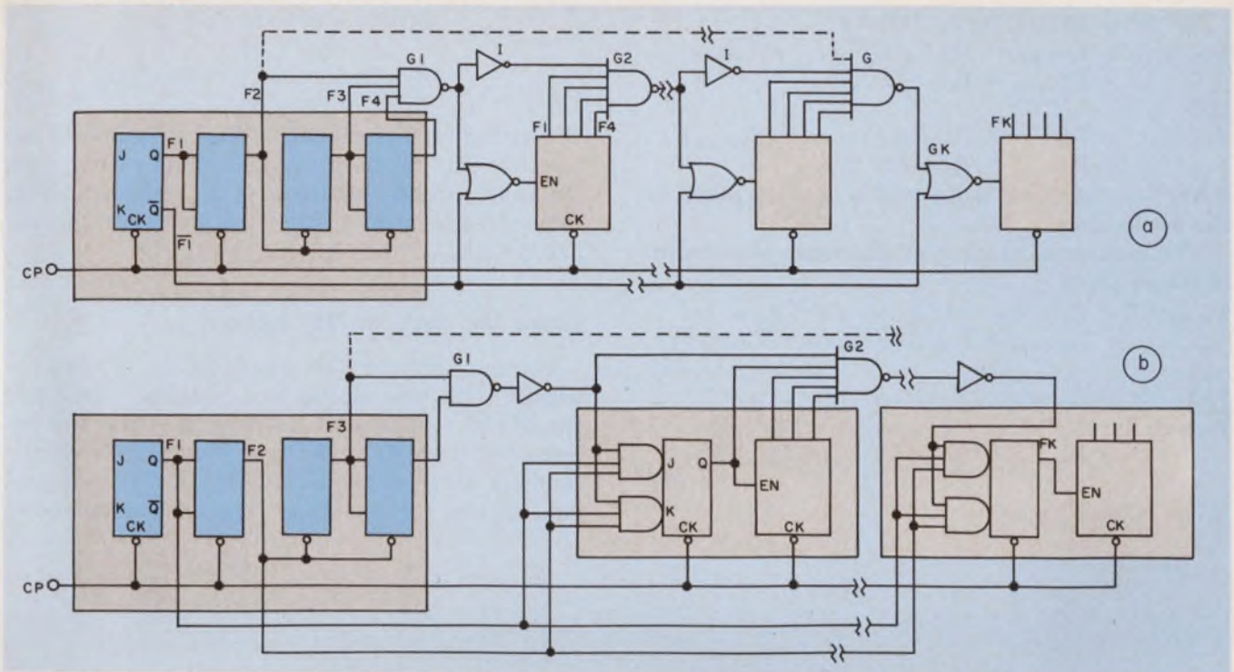
1. Counter size with parallel enabling is double or almost quadruple that for serial enabling. Parallel injection of F_1 eliminates the ripple delay of the first stage's 0-to-1 transition (a); parallel injection of F_1 and F_2 de-
