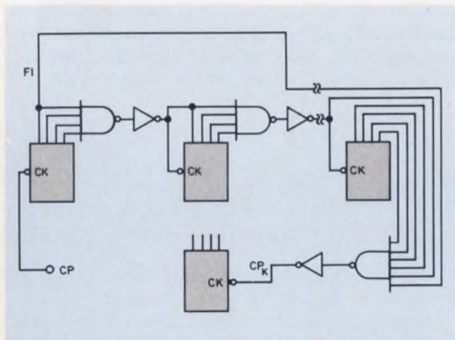
4. Clock-timing restrictions are removed with this configuration of MSI ripple-counters. The signal from F_1 —the first flip-flop stage of the first section—becomes the virtual or secondary clock for the counter. The addition of F_1 to each counter section eliminates the 1-to-0 ripple delay of the gates.
