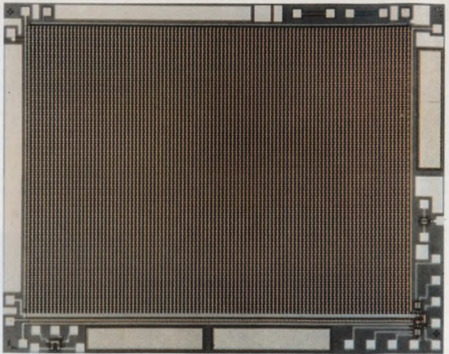
This 100 × 100-element self-scanned charge-coupled array, by Fairchild, has an image aspect ratio of 4 × 3. The charge coupling uses buried channels.
