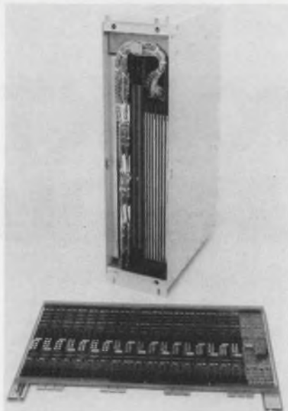
A 65-kilobyte core memory from Toko offers maximum access time of 180 ns and max cycle of 250 ns.
