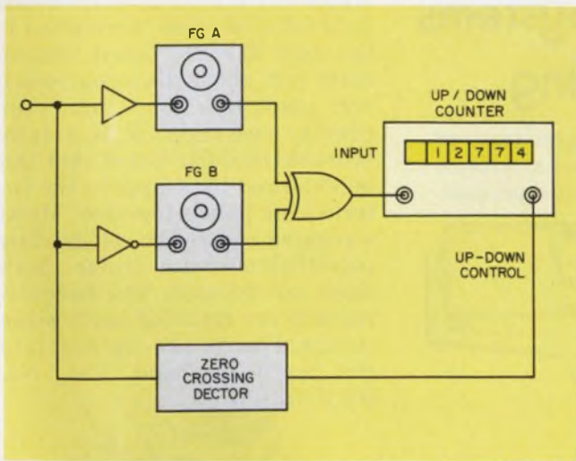
4. An up-down counter gives a direct integration of a bipolar voltage when controlled by a polarity-sensitive signal derived from the input.
