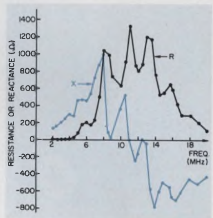
Tree-antenna resistance and reactance are shown here for an oak tree with a Hemac 2.3 m above moist ground in a forest.
