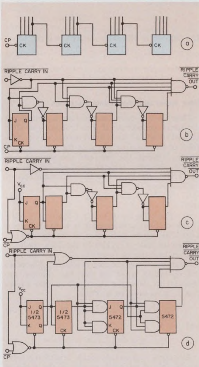
7. Synchronous sections boost speed. The ripple connection (a) is the simplest for multisection counters. Each stage (flip-flop) must be enabled at the same time since they are all toggled by the clock (b). Enabling the clock simplifies the circuitry (c) and (d). Similar circuits are available as MSI sections.
