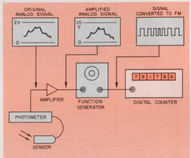
1. In a scheme to integrate the light falling on a photo-sensor, the sensor's output signal, after conditioning, is used to control the frequency of a function generator. A digital events counter then accumulates—or integrates—the frequency over the period of interest.
