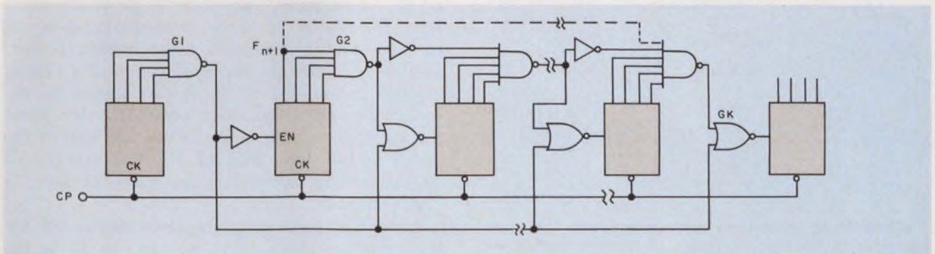
2. Apply parallel enabling from all flip-flops in a single section and you are using the terminal count—as generated by the multi-input AND gate. The same 74L30
