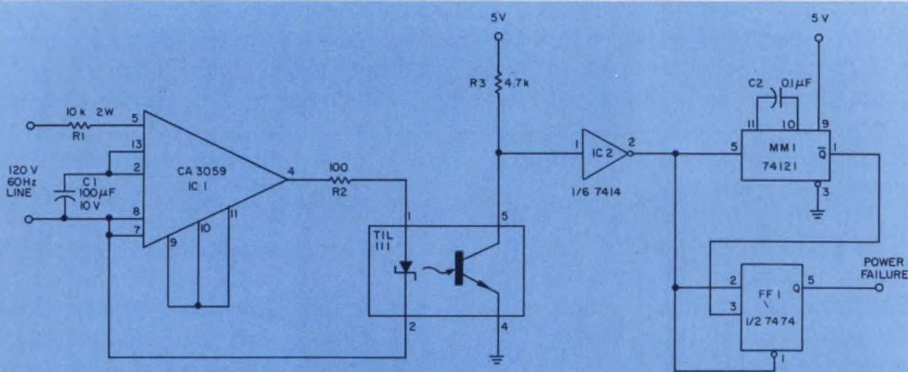
Zero-voltage switch minimizes reaction time of a power-failure detector. MM 1 times out and sets FF 1
