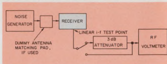
6. When an i-f prelimiter test point is available, this setup can measure receiver noise figure.
