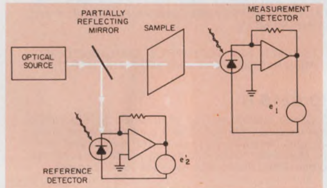
2. A reference detector, which delivers a signal proportional to the incident-intensity level, has been added to the straightforward system of Fig. 1. The new signal can generate a source-variation correction term.
