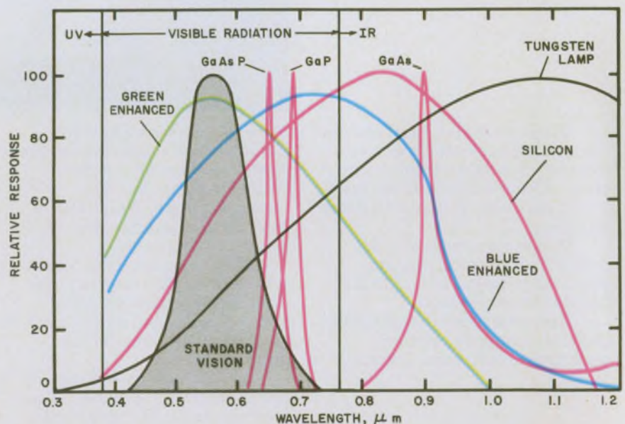
1. The spectral response of silicon has been modified by several manufacturers to improve shorter-wavelength sensitivity. One of Vactec's cells has the blue-enhanced curve while one of Sensor Technology's has the green.
