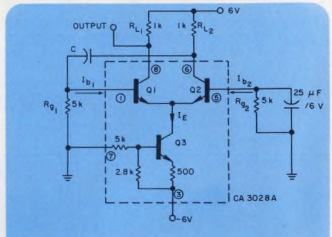
Capacitor C provides positive feedback for this astable multivibrator. Positive starts are assured since Q_1 and Q_2 do not saturate during their conductive periods.
