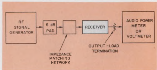
1. Receiver quieting can be measured from a simple setup. However the technique can't distinguish between i-f and audio response.
