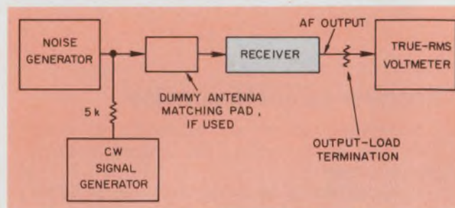
7. When only the audio output is accessible, this setup can measure receiver noise figure. The measurement is made on the linear portion of the quieting curve. Even an FM receiver has a small range of linear relation.
