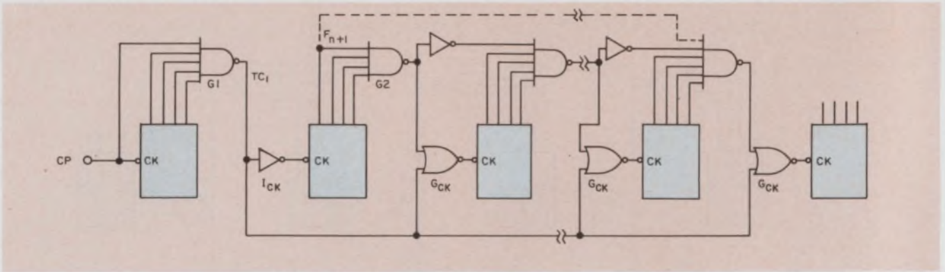
6. Maximum IC ripple-section performance is obtained by a combination of techniques. The parallel injection of the terminal count, as in Fig. 2, maximizes the counter
