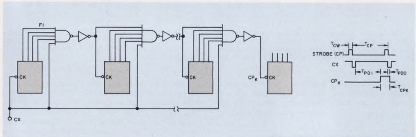
3. Serial-enabling scheme allows use of MSI ripple-counter packages that do not afford access to the J-K inputs of individual flip-flops. The clock pins are used
