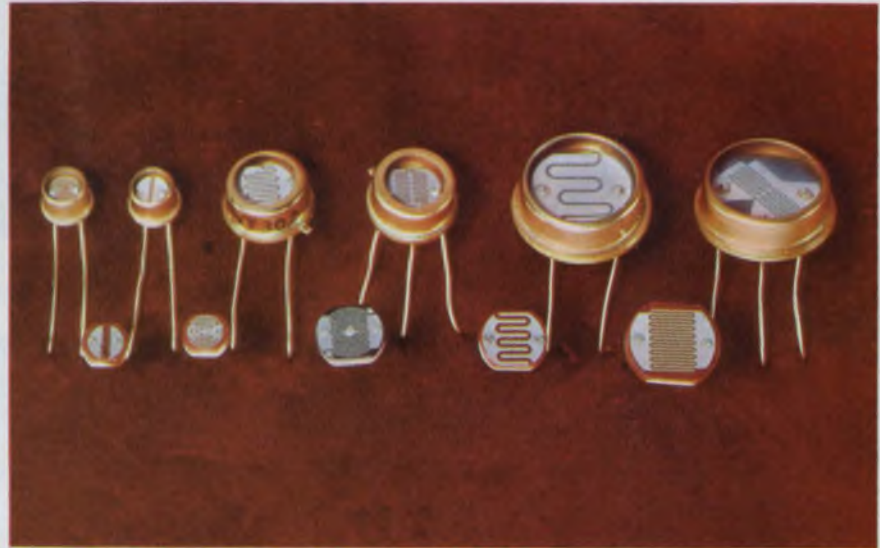
Cadmium sulfide and cadmium selenide photoconductive cells provide the highest sensitivity per unit cost of any photosensor. Some types of these cells, like these by Vactec, are more sensitive than photomultiplier tubes.
