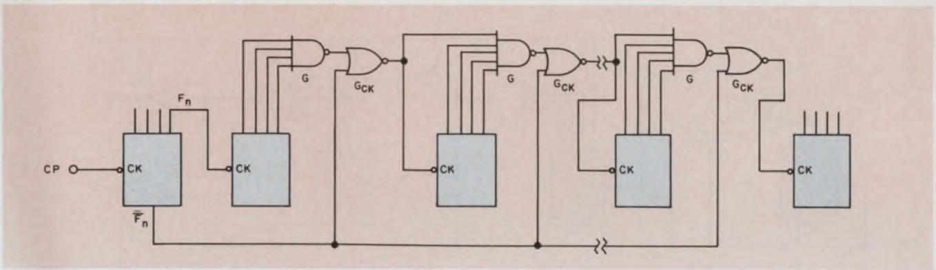
8. Synchronous sections can be used in a serial-enabled counter configuration (a). The first gate-inverter pair—required for ripple sections—can be eliminated. The last
