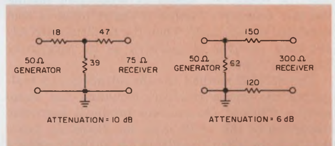
4. Simple impedance matching pads can be built to provide a wide range of attenuation values.
