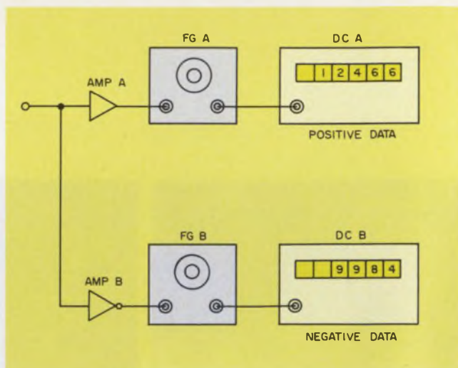
3. To integrate bipolar signals, two duplicate channels can be used. The counts of each channel are then added algebraically to get the final result.
