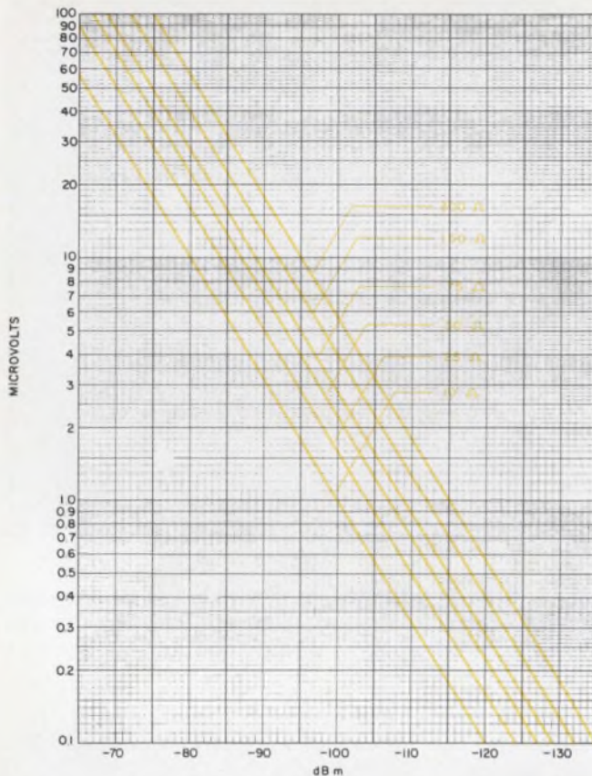
9. Conversion of dBm to \mu\text{V} for a given receiver impedance can be performed with this graph.
