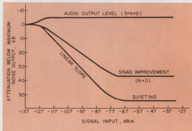
2. Typical SINAD and quieting curves exhibit a leveling off in output noise. The linear region in the quieting curve, beyond the start of limiting, permits a simplification of the noise-figure measurement.
