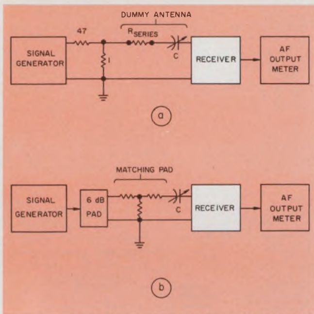
5. An unknown receiver input resistance can be found by measurement (a). The value found can then be used to build a matching pad that ensures maximum power transfer between generator and receiver (b).
