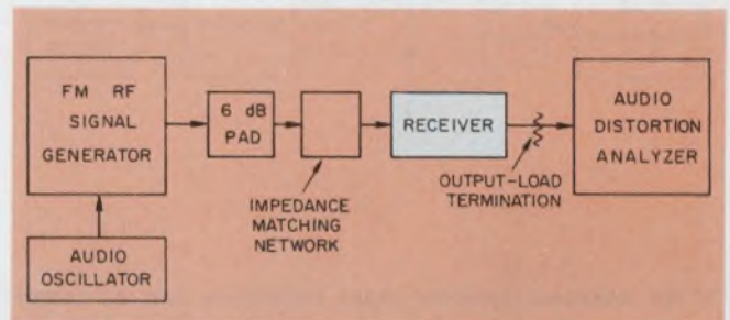
3. The SINAD measuring setup, similar to that for quieting, uses a modulated rf signal and distortion analyzer to notch out the recovered audio tone.
