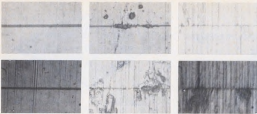
Photomicrographs of the surfaces of single-crystal (left), polycrystalline (center) and permalloy tape heads before (top) and after 500 hours of running time with Crolyn tape.
