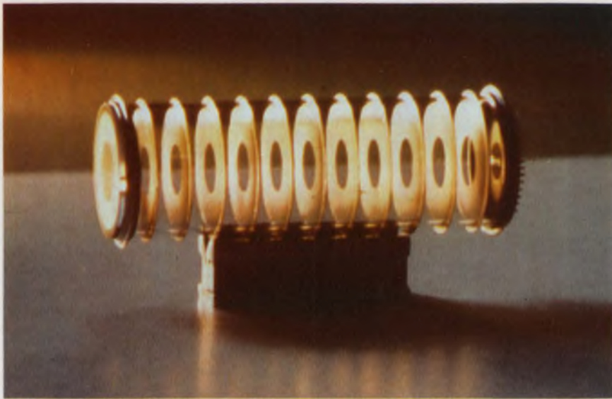
A new supersensitive solid-state photomultiplier, by Electronic Vision Corp. focuses electrons from a photocathode onto a silicon array. Each of the electrons striking the silicon is multiplied by several thousand.
