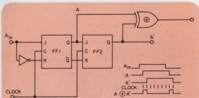
2. The EXCLUSIVE-OR of signals A and A' determines the transition points of the transducer signal A IN .
