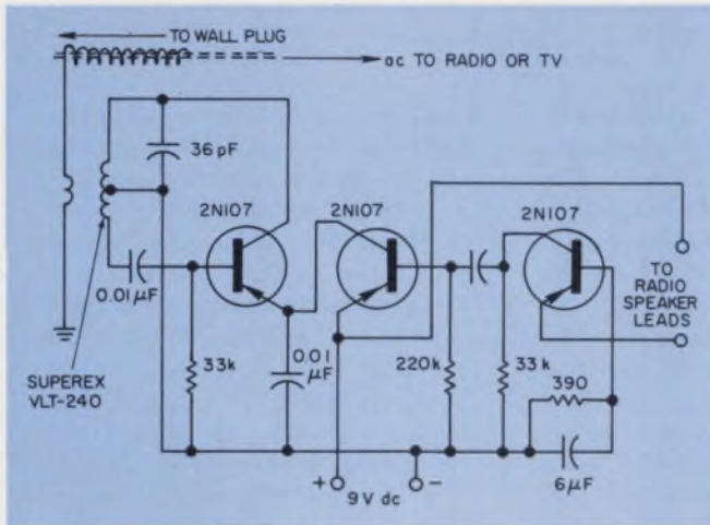
By using the speaker as a microphone and the ac power line as an antenna, an AM radio can be converted into a bug that picks up room conversation.
