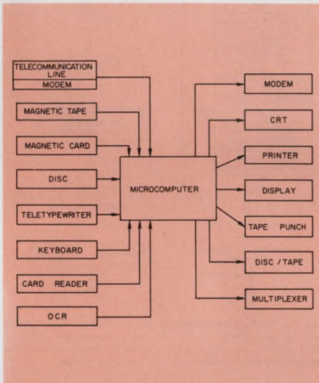
2. Any computer peripheral can work with microprocessors. Interface requirements are determined by word length and any additional hardware needed.
