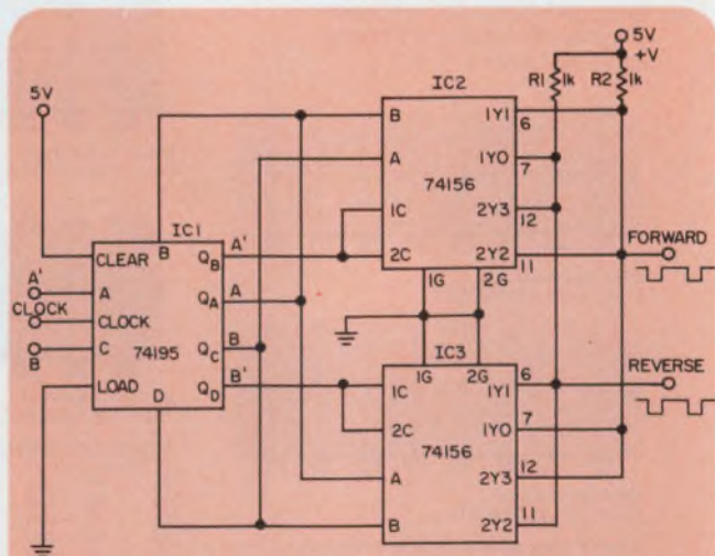
3. Pulse trains appear at the output of IC 2 or IC 3 , in the quadrature decoder, depending on whether the transducer motion is in the forward or reverse direction. The number of pulses generated is proportional to the transducer displacement. The clock rate should be set for at least eight times the pulse frequency of the input.
