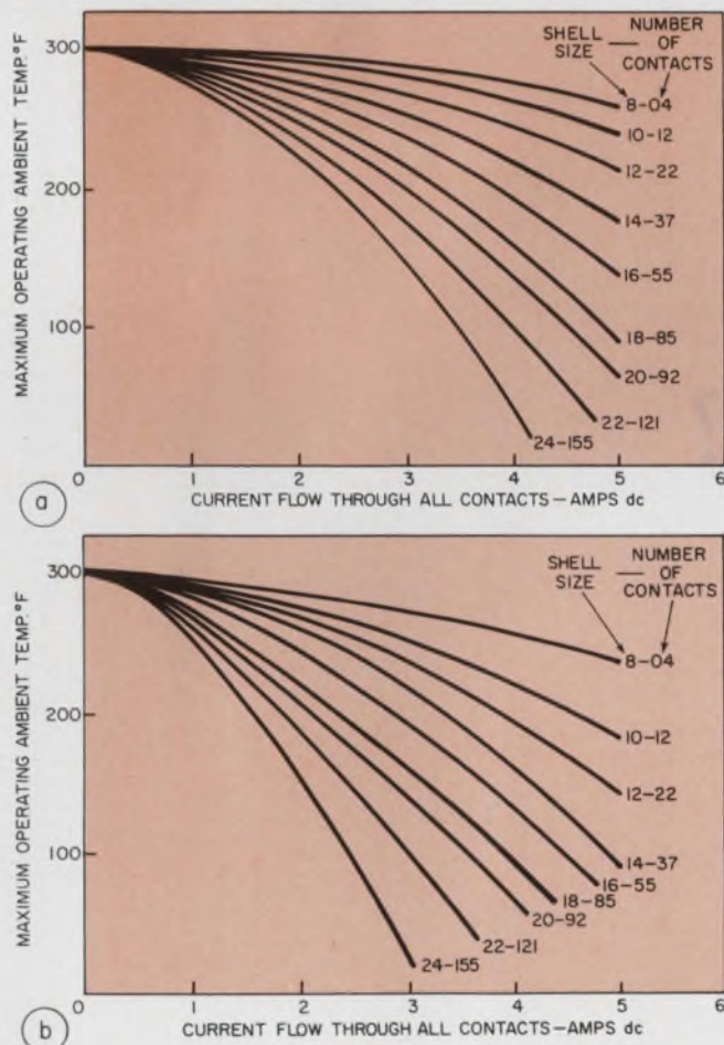
2. Maximum operating ambient temperature at sea level (a) and 110,000 foot altitude (b) with the connector cooled by natural convection.
