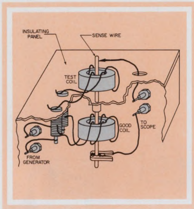
4. The simple test fixture needs almost no components to do its job.
