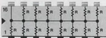
898-1 (15 resistors) Price (1,000-4,999) $ .85
