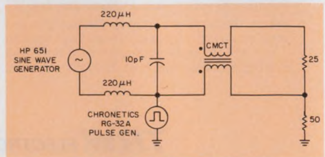
2. 10-MHz differential signal is unattenuated, but the common-mode pulse is rejected.
