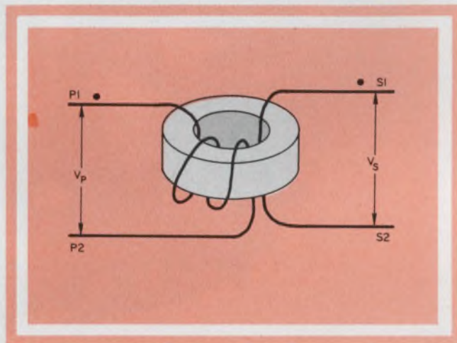
1. Basic toroidal coil obeys the simple transformer law.
