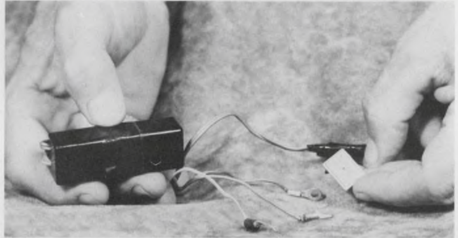
Three-wire bug can be placed in a telephone base and transmit both room and telephone conversations up to 800 feet under good conditions. It measures 2-1/2 by 1/2 by 1/2 inches and can be installed in five minutes.
