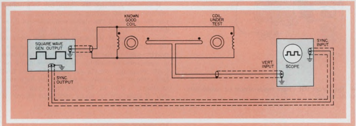
2. Coils are tested with a very simple circuit, a scope and a square-wave generator.
