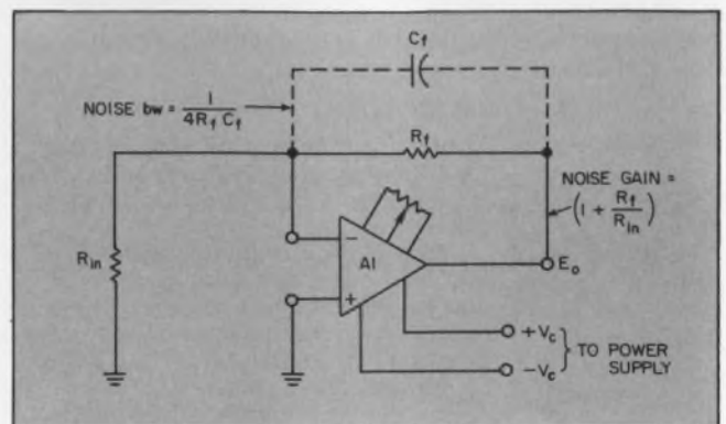
1. Op amp powered by dc/dc converter passes negligible converter switching spikes because of narrow bandwidth and slow response.
