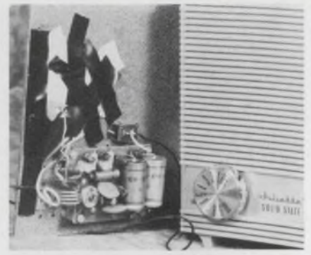
The quality of this radio will be so poor you'll soon stop using it, even though it's a gift. Good! That's when the hidden transmitter (left) can operate, loud and clear.
