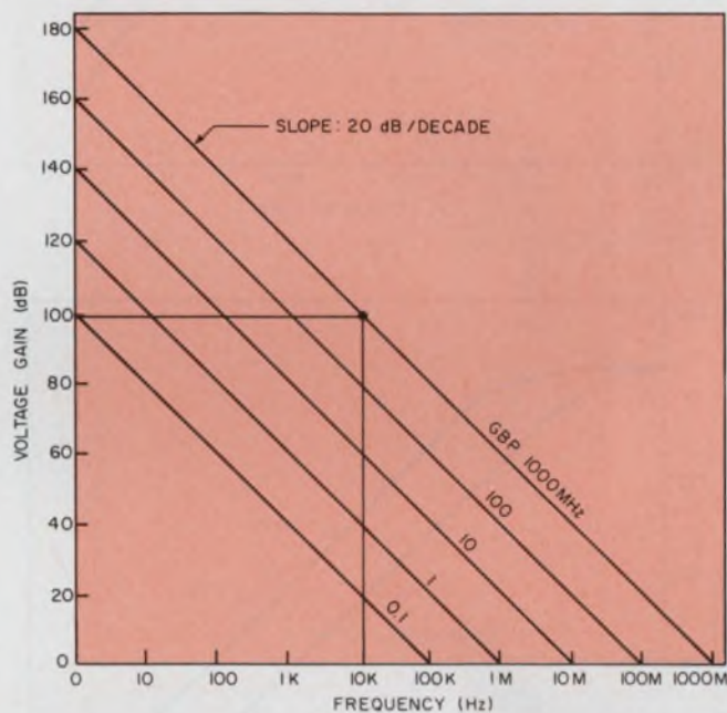
2. Nomogram for estimating required gain-bandwidth product (GBP). Select the highest operating frequency and draw a line equal to the operating gain plus the desired loop gain, both expressed in dB. The intersection of this line with one of the constant GBP curves yields the required amplifier GBP.
