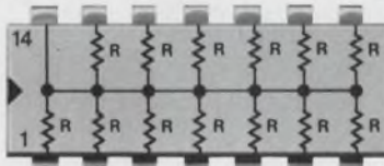
899-1 (13 resistors) Price (1,000-4,999) $ .81
