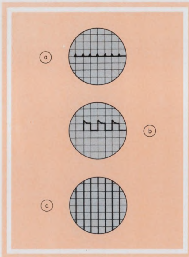
5. Typical test patterns on the scope show the results if two identical coils are tested (a). If two coils differ by a small number of turns, a square-wave pattern results (b). If the two coils are connected wrong or wound in opposite directions, a vertical grid appears (c).
