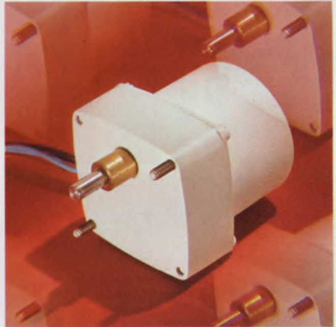
Heavy-duty timing motors , such as this 600 rpm 86600-series unit from North American Philips, can handle rugged load conditions more safely than light-duty timing motors, even though the light-duty motors may be able to develop the required torque.
