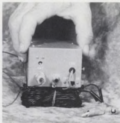
High-powered telephone wiretap transmitter, built by Gene Levette in Canada, has a 2-W power output and a two-mile range. Filters eliminate suspicious noise.
