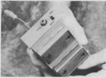
Bumper beeper is built with two 14-pound magnets, which stick to the gas tank of a car to be tailed. A direction finder can pick up the beeper's 100-cycle signals.
