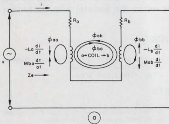
(a) Impedance of series circuit with mutual inductance subtracting.
