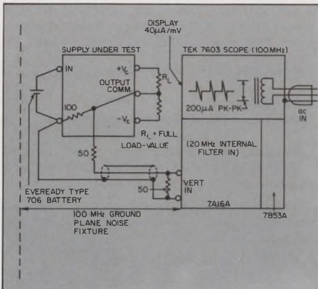
4. "Common-mode" current noise between a converter's output and input common terminals should also be measured. This unwanted noise can saturate a differential-input op-amp being powered by the converter.
