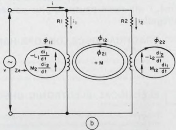
(b) Impedance of parallel branches with mutual inductance adding 2 (assuming constant circuit parameters).
