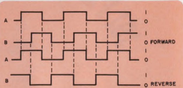
1. Forward or reverse movements of an incremental encoder cause waveform B either to lag or lead waveform A.
