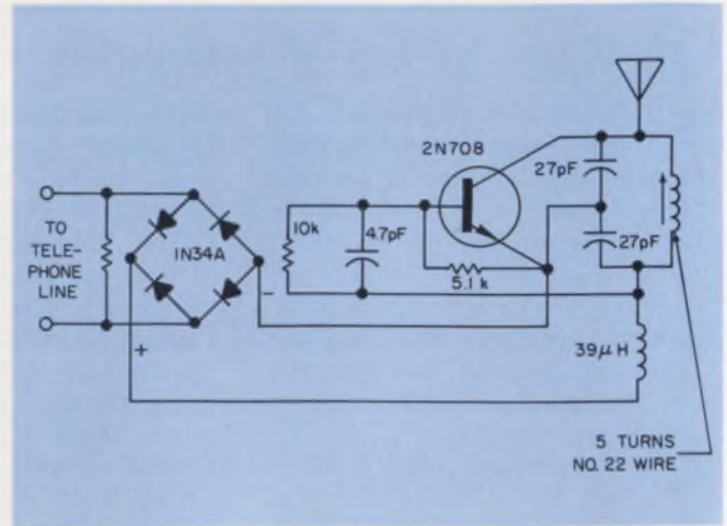
A series-connected bug draws its power from the telephone line and transmits both sides of the conversation. The bug can be installed anywhere on the line.
