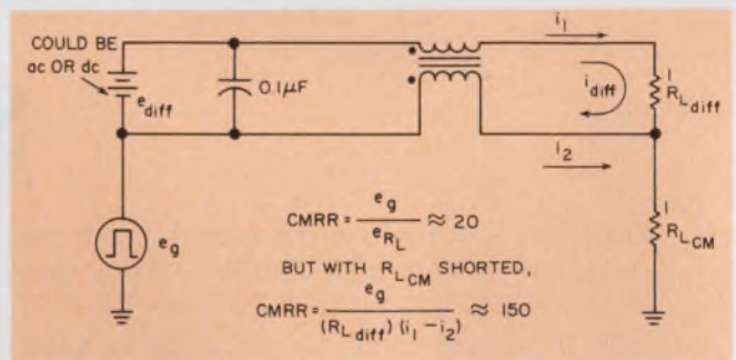
1. The CMCT "rejects" an unwanted common-mode pulse, e_c , but passes the desired dc differential current.
