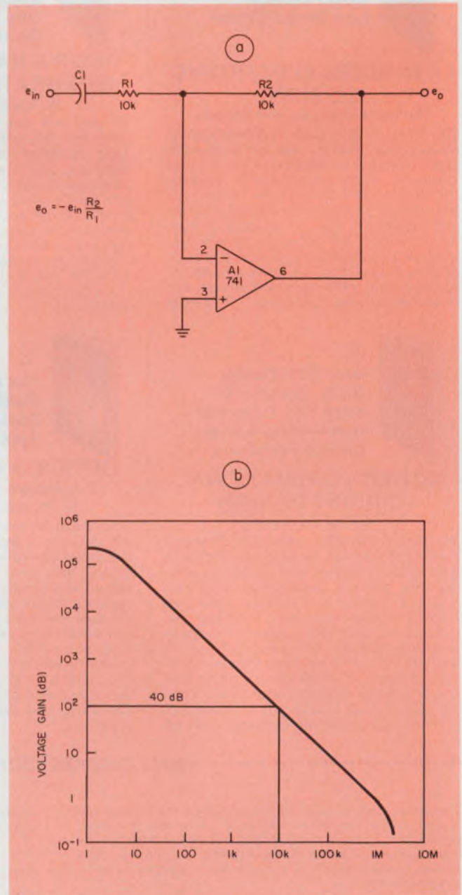
1. At unity gain the simple op-amp inverter (a) can provide a 500-kHz bandwidth. The maximum upper corner frequency of the circuit for a selected value of gain equals the open-loop gain of the amplifier itself (b), as shown by the horizontal line for a noise gain of 40 dB. Vertical lines indicate the maximum circuit gain at any given frequency.
