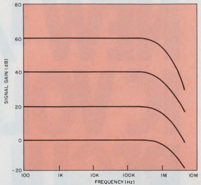
8. Use of optimum compensation for the 709 permits operation with almost constant bandwidth—a characteristic of circuits having adequate loop gain.
