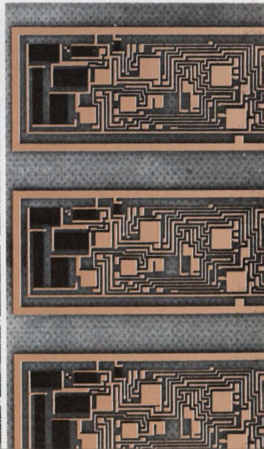
Hybrid microelectronics
