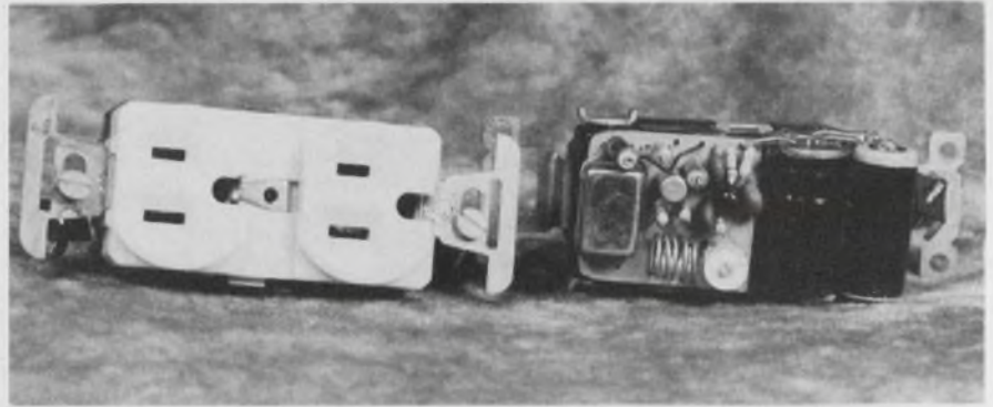
The bug in the plug pulls juice from the wall plug it's slipped into, and it will transmit indefinitely all room conversations to a receiver 800 feet away. The unit can still be used as an electric plug while transmitting.
