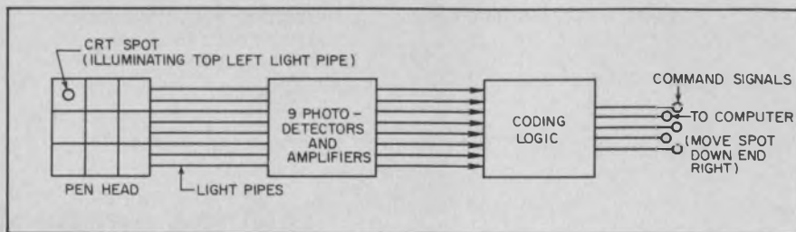
Light pen can be built for about $75.
