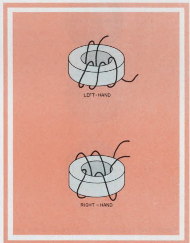
3. A toroidal coil can be wound in either of two directions and still deliver correct voltages.
