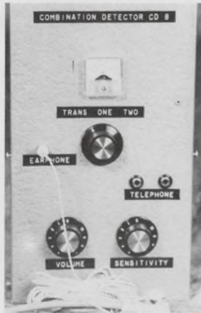
Debugging device is an untuned rf receiver that picks up signals between 1.75 and 900 MHz. When the receiver squeals, it has picked up a hidden, active transmitter.
