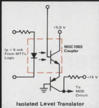
Isolated Level Translator
