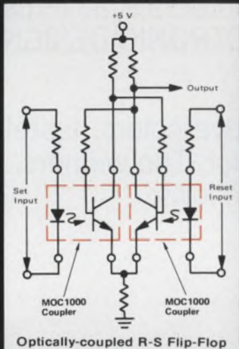
Optically-coupled R-S Flip-Flop
