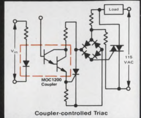
Coupler-controlled Triac
