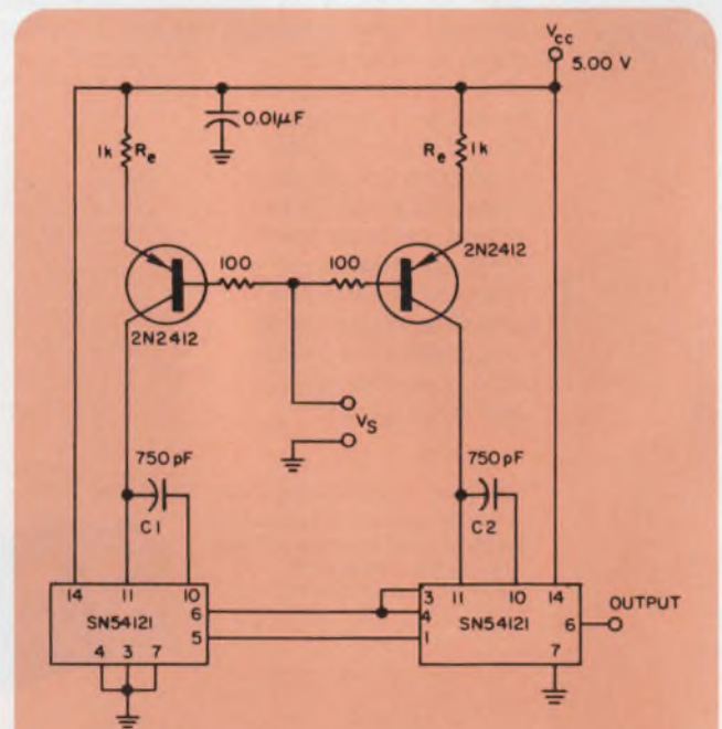
2. Voltage-to-frequency converter uses SN54121 one-shots controlled by 2N2412 transistors connected as current sources.
