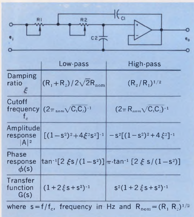
1. A noninverting configuration with variable resistances can be used as a tuneable active filter (top). In high-pass or low-pass applications, f_c and \xi are independently adjustable (bottom).
