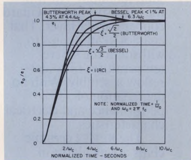
4. The output response time and overshoot are indicated for a low-pass, second-order step input.
