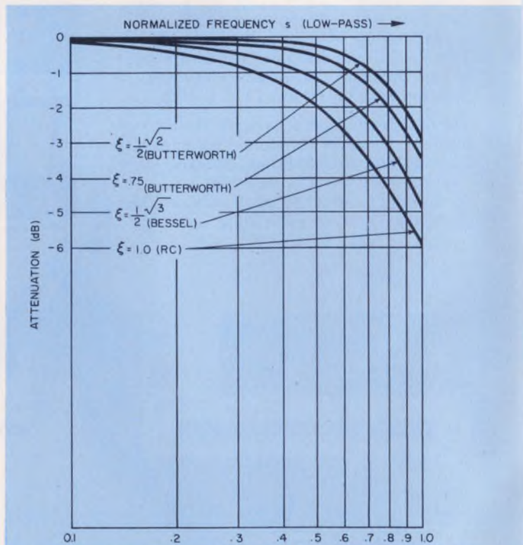
2. For high-pass as well as low-pass applications, the normalized curves cover the range of damping ratios
