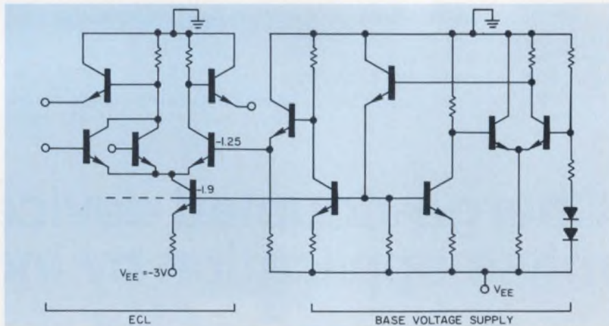
Hitachi's modified ECL circuit has a differential base-voltage circuit that supplies current-source transistors. A self-aligned etching technique produces high-speed switching transistors with small base areas. The special base-drive circuit insures reliable operation and relatively low power dissipation.
