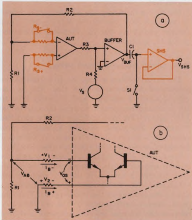
2. Adding source resistors and memory to the basic circuit of Fig. 1 permits measurement of the input offset current, I_{OS} . (a). The meaning of the offset current is explained by considering the two input bias currents (b).
