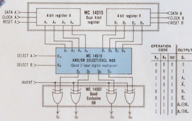
Select-Compare Data Register Total Quiescent Power Dissipation 25 \mu W @ 5 V ( V_{DD} )
