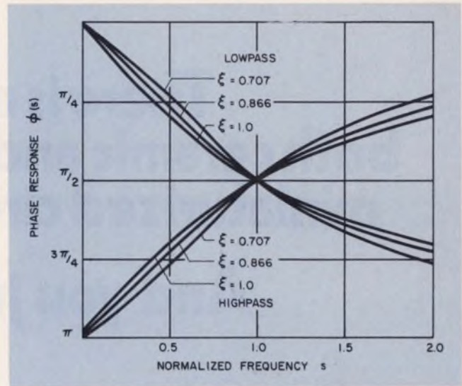
3. The output-to-input phase response is determined once the cutoff frequency and damping ratio are selected. For both high-pass and low-pass filters, the insertion phase shift at f=f_c is \pi/2 .
