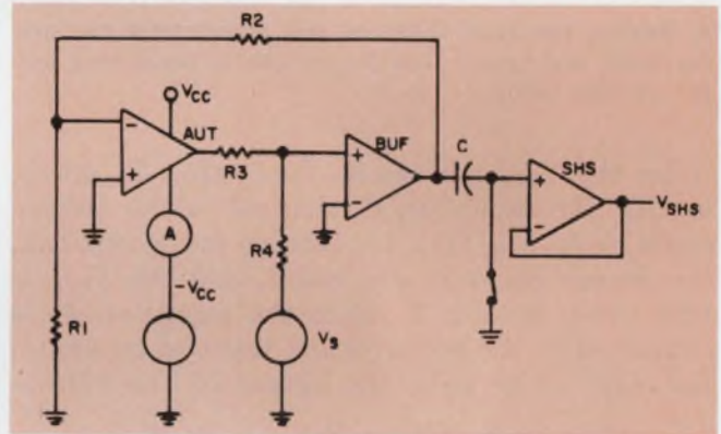
4. Supply current, I_S , and large-signal voltage gain, A_V , are measured with the basic test circuit and a sample-hold-and-subtract (SHS) circuit.
