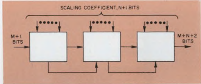
3. Any number of multipliers can be connected in tandem to accommodate a scaling coefficient of any length (N = 8 per multiplier).
