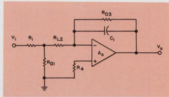
5. The reset-mode equivalent circuit applies during discharge of C_1 . The input voltage is attenuated by R_{01} , where R_{01} \ll R_i , and isolated by R_{1,2} . Unity gain compensation eliminates instability.
