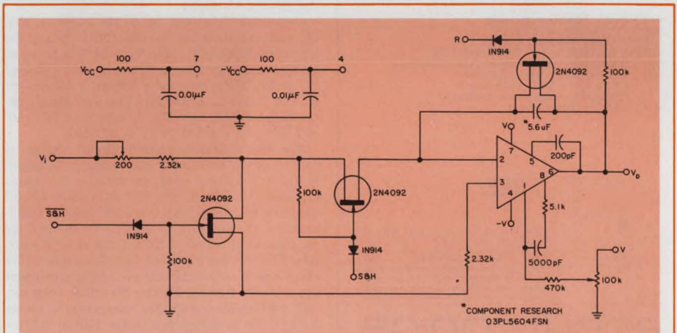
7. The final sample-and-hold circuit design includes all of the components selected, biasing for the FET switches, the compensation network and
