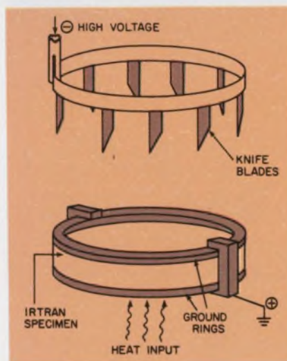
2. The best electrostatic cooling of the Irtran window was obtained with the setup shown above.
