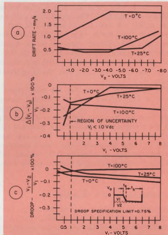
8. Measured data of the sample-and-hold design show the drift rate (a) plotted for one-second averages. Drift rates are significantly smaller for t_b \ll 1s . The accuracy with which a given input is reproduced at the output is shown in b. Plotted in c, the percent change in the output voltage.
