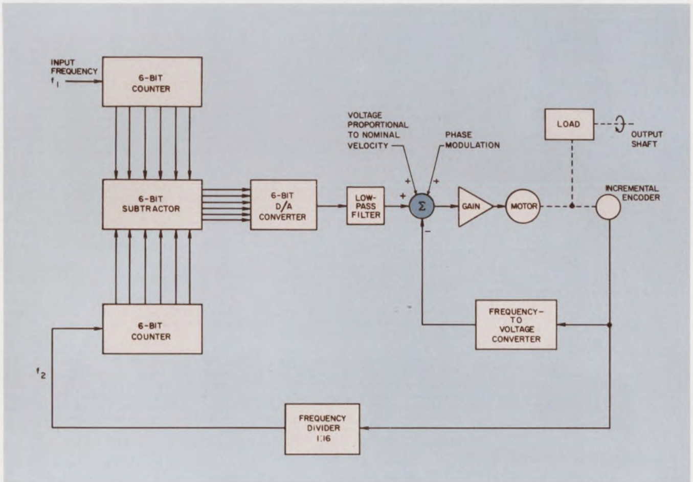
6. An application of a six-bit digital phase-locked loop is this precision velocity servo. This design minimizes the
