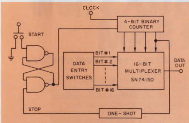
2. A multiplexer is used as the basic storage element in this 16-bit word generator. The outputs of the data entry switches are always available at the inputs to the multiplexer. Once the start button is depressed, the counter controls the sequencing of the multiplexer.
