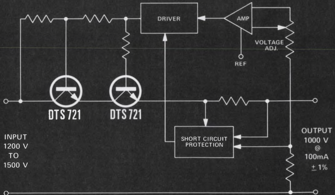
DC Regulator Circuit
