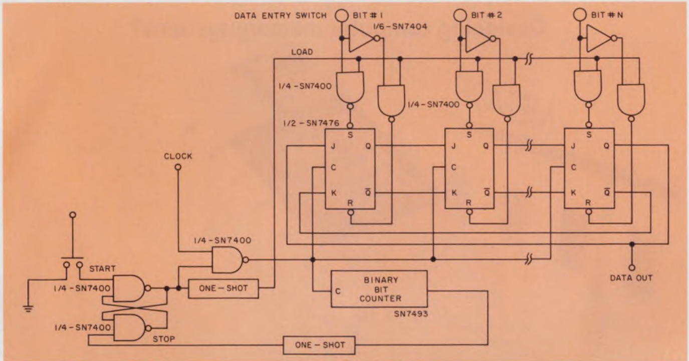
1. The simplest form of programmable word generator uses flip-flops to form a presettable shift register. This word generator is easy to build and is extremely useful
