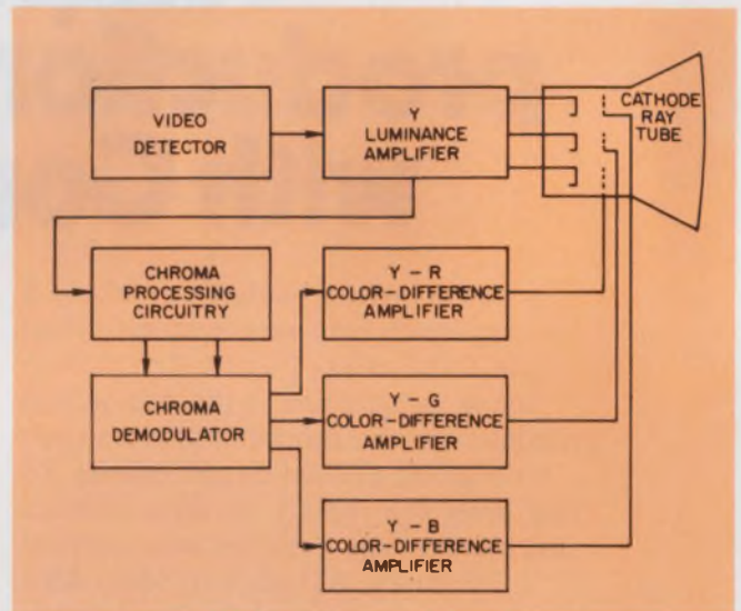
1. The color-difference circuit needs a powerful luminance amplifier that requires not only a high-power transistor but a large heat sink as well. It has the advantage of providing identical luminance transient responses for all three colors, thus eliminating a source of color fringing.
