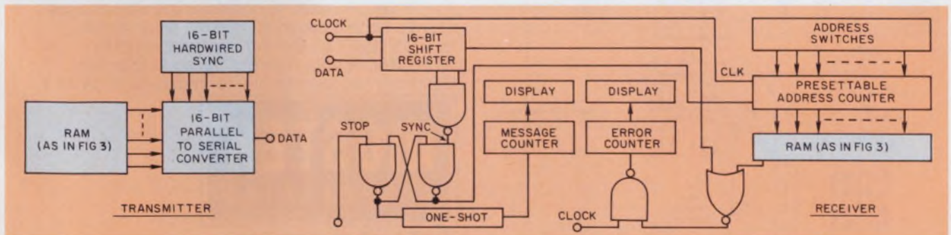
4. Two simple programmable word generators form a bit-error detector. The transmitter produces the test signal that is applied to the system under test. The sys-
