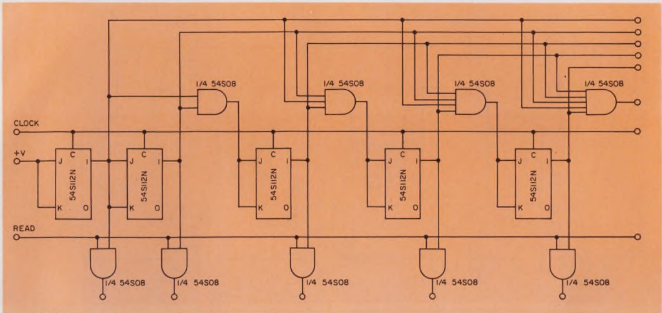
1. The complex gating network limits the speed of the synchronous counter. Before a flip-flop can be toggled,
