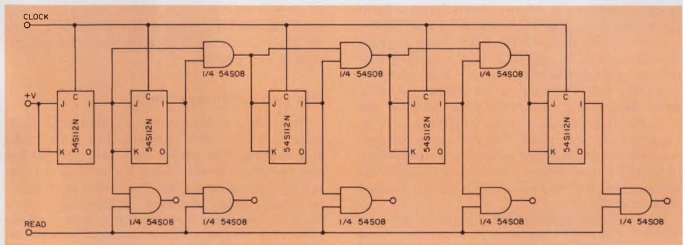
2. The features of both the synchronous and ripple counters are combined in a counter whose speed is limited
