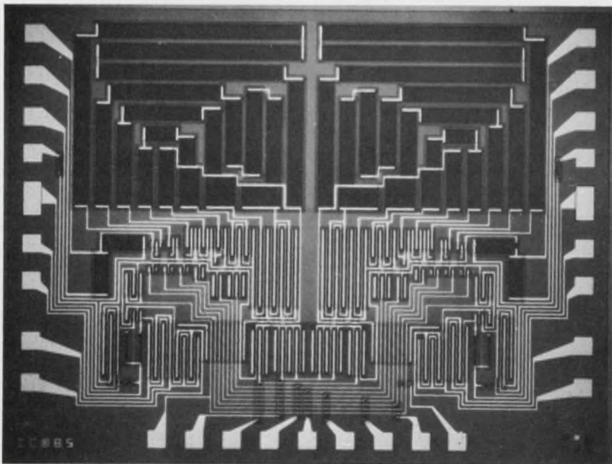
This digital-to-analog converter for Hughes' DC-10 jet entertainment system uses an implanted resistor ladder (top) for reliable performance and low cost.
