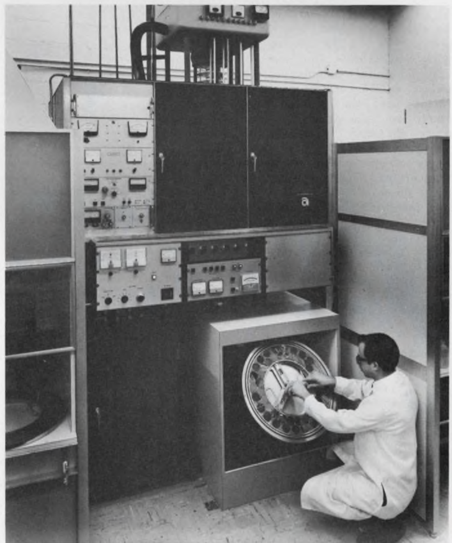
In one of Hughes Aircraft's newest ion-implantation systems for MOSFET ICs, a technician loads silicon wafers in the vacuum implantation chamber.
