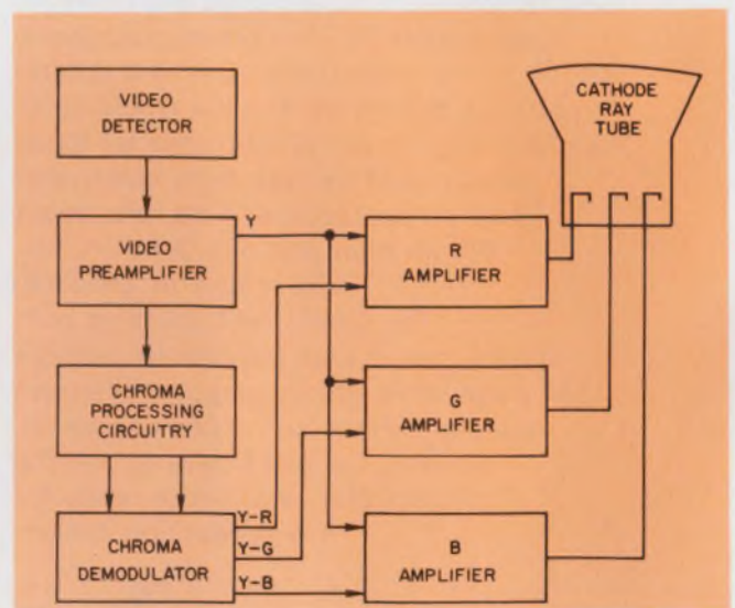
2. The red-green-blue circuit uses a separate amplifier for each cathode. Both luminance and color-difference signals are applied to these amplifiers. Therefore, individual amplifier gain adjustments will affect both chroma and luminance information, preserving their proper relationship at the CRT.
