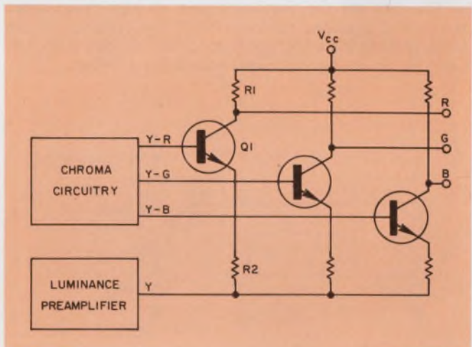
3. Each transistor acts as a common-emitter amplifier to the color-difference signal and as a common-base amplifier to the luminance signal. The gain of the former is -R_1/R_2 , while that of the latter is +R_1/R_2 .
