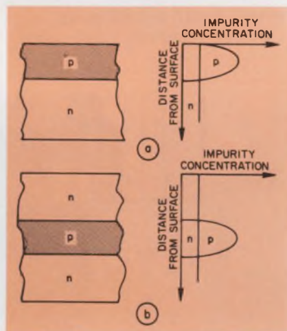
1. Layers of impurity concentrations can be implanted at the surface of a substrate (a) or buried inside (b).
