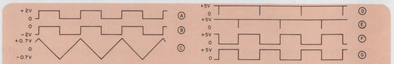
2. Available outputs include a fully adjustable triangular waveform, negative-going synchronization
