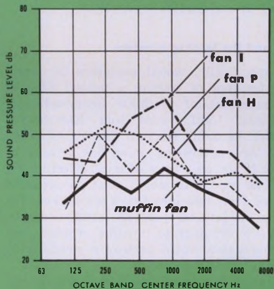
Results of acoustical analysis conducted under like conditions at 60 Hz and free air delivery Microphone 3 feet from specimens.
