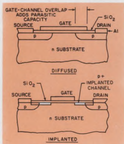
2. The parasitic capacities in diffused MOSFETs are eliminated by Hughes' ion-implanted structure.
