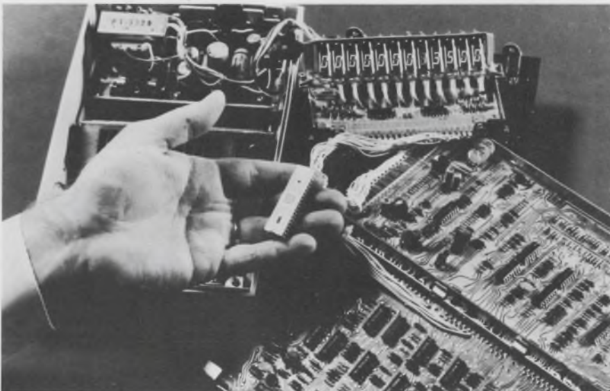
The single MOS-LSI chip (held in the hand) contains the complete logic for an electronic calculator. It replaces 22 MSI circuits and many discrete components contained on two circuit boards.
