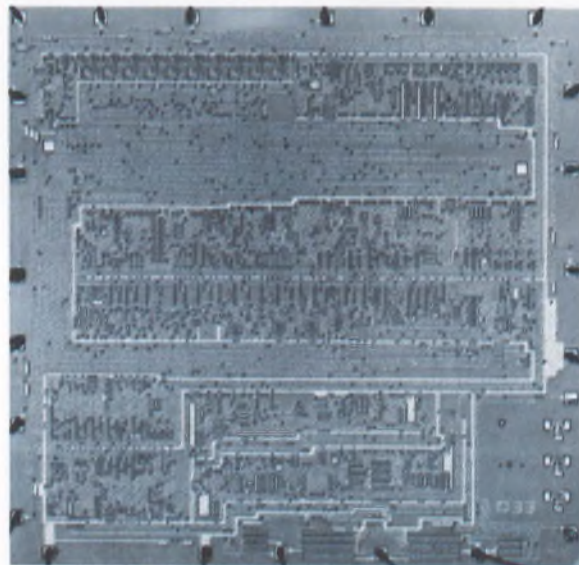
Custom MOS/LSI in Boeing 747 electronics.
