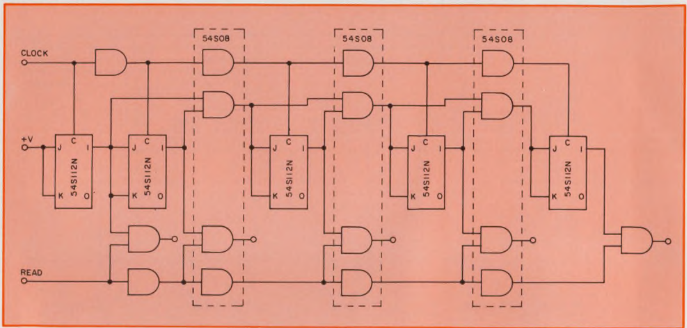
3. A simple modification of the synchronous/ripple counter of Fig. 2 can increase its speed beyond that of the synchronous counter. By applying both the clock and
