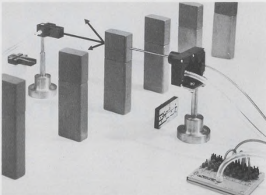
2. The fluidic ear , with a cutaway view of the transmitting and receiving elements. The receiver is reported to operate anywhere within five feet of the 50-kHz source.
