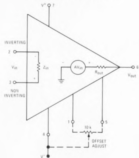
EQUIVALENT CIRCUIT
