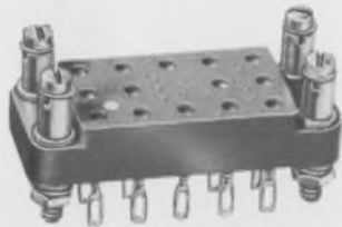
145-8-10/14 CONTACTS/FIXED
