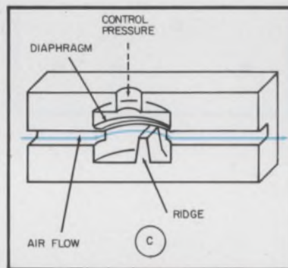
1. Three approaches to fluidic logic are shown above. The wall-attachment principle (a), the impact modulator (b) and the diaphragm-valve design (c).
