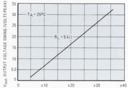
PEAK OUTPUT VOLTAGE SWING versus POWER SUPPLY VOLTAGE
