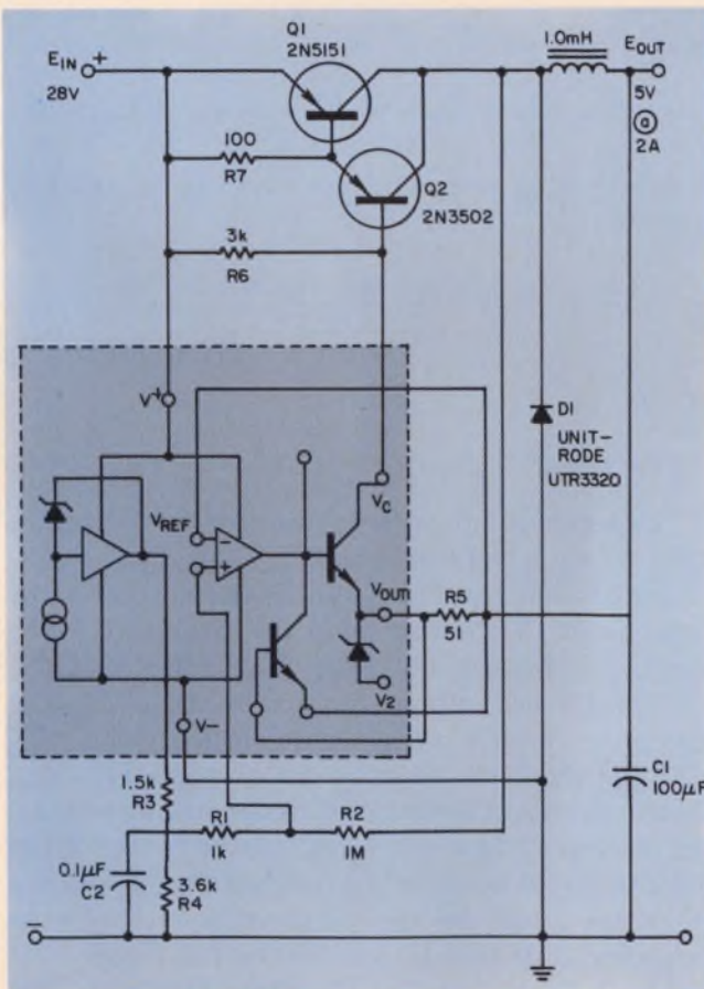
5. A positive switching-mode regulator using a linear IC voltage regulator as control circuitry achieves 73% efficiency with a 5-V, 2-A output and an input of 28 V. The series inductance L_s is 40 turns of #20 enameled copper wire wound on a Ferroxcube P36/22-3B7 core with 0.009-inch air gap (or equivalent).
