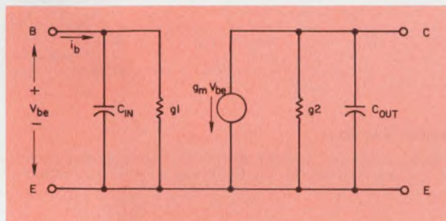
4. This simplified hybrid-pi model of a microwave transistor is more complicated than it looks. The capacitances include both interelectrode and packaging effects.
