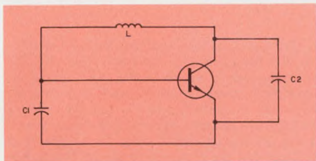
3. The Colpitts oscillator is an excellent choice for microwave operation. The capacitances shown in this simplified model can be provided by the transistor's parasitics. The inductor can be realized with a transmission-line section.
