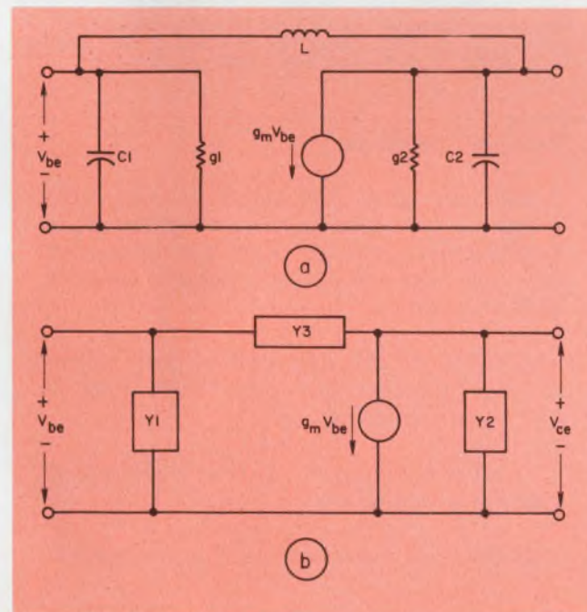
5. Combining the transistor model of Fig. 4 with the Colpitts circuit of Fig. 3 yields circuit (a) where C_1 and C_2 actually represent C_{IN} and C_{OUT} of Fig. 4. By adding the parallel admittances, a simplified circuit (b) is obtained. In (b), Y_1 = g_1 + j\omega C_1 ; Y_2 = g_2 + j\omega C_2 ; and Y_3 = -j/\omega L .
