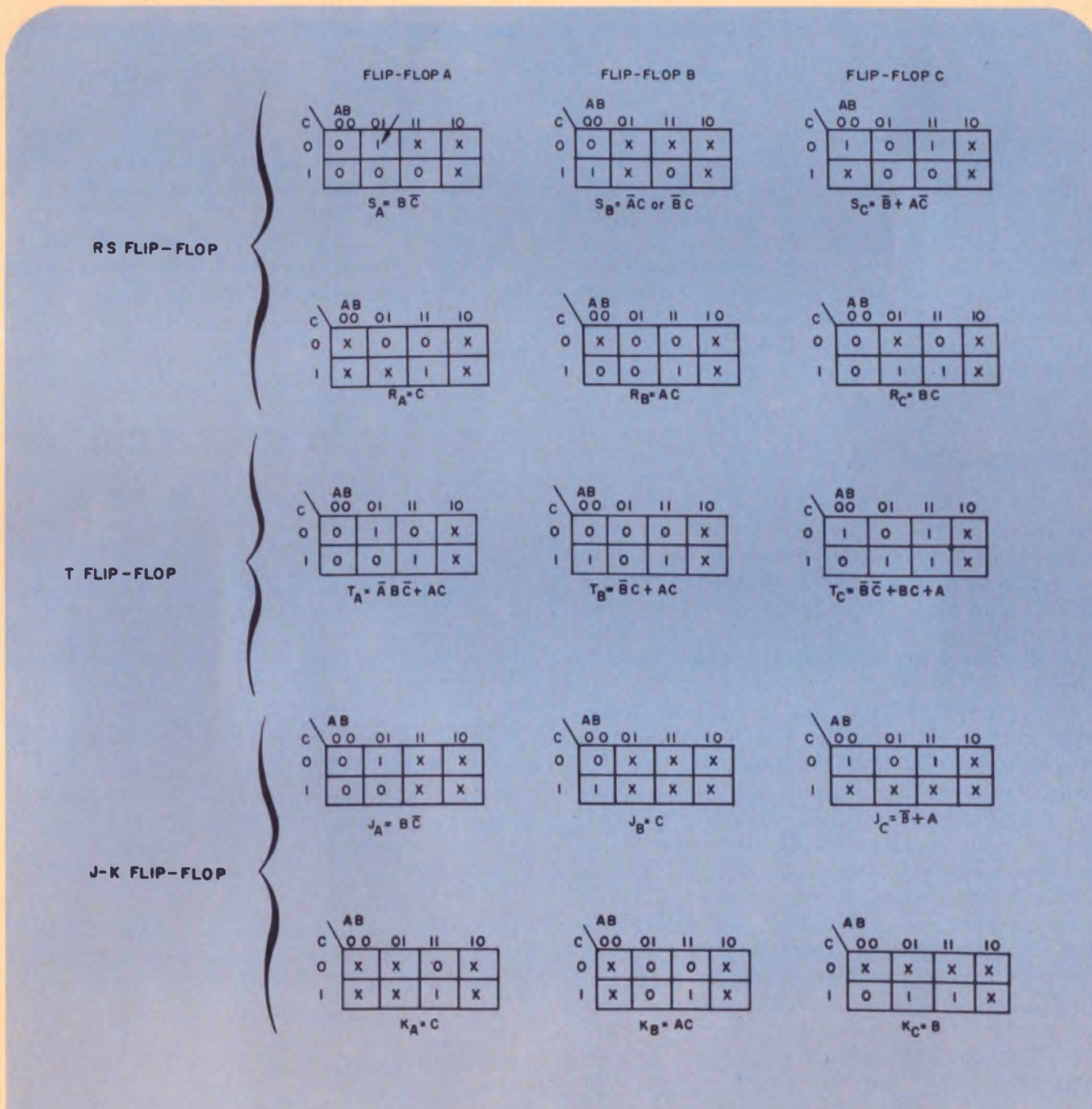
5. The three flip-flop sequential counter flow table (Fig. 3) translates into this multiple set of maps.
