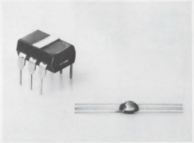
Magnetically sensitive transistor called Mag-nistor detects 0.5 mV/gauss, p. 94.
