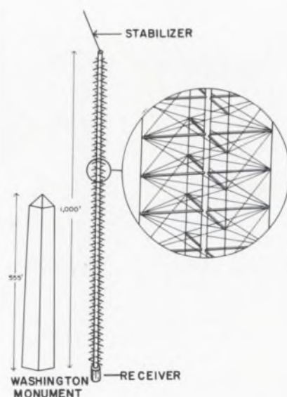
A 1000-foot antenna is proposed for low-frequency mapping of sky.
