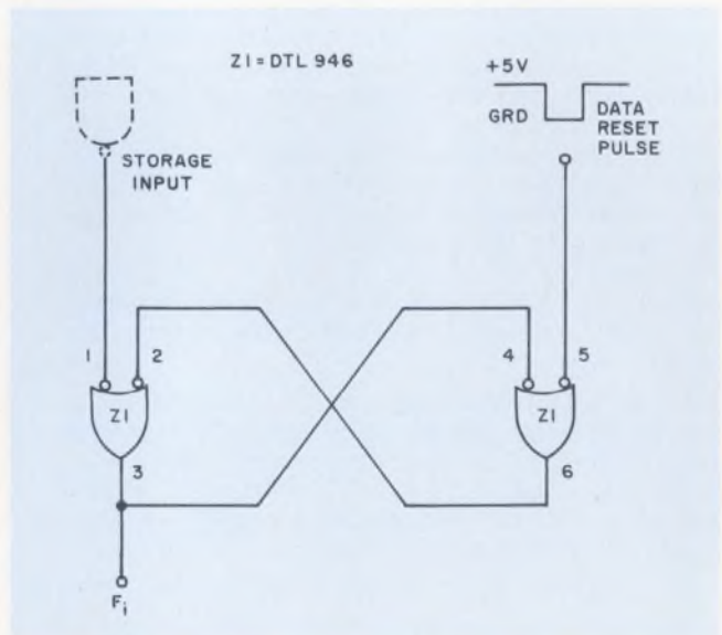
14. Another storage register uses only one DTL 946 package. It is used in the serial-to-parallel converter of Fig. 17.
