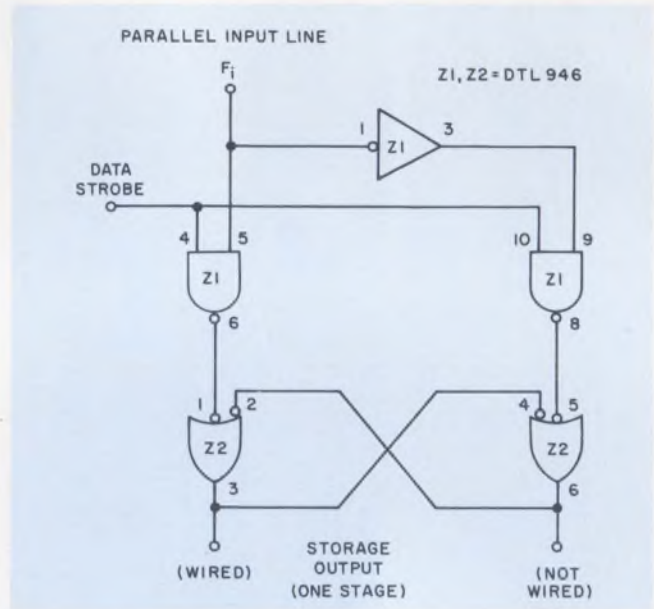
13. Two DTL 946 packages make one stage of an n-bit storage register. This is the register used in the parallel-to-serial converter of Fig. 15.
