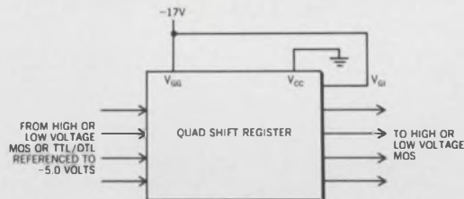
MOS Operation
