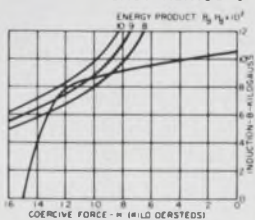
TYPICAL DEMAGNETIZATION CURVE OF CAST ALNICO 9
