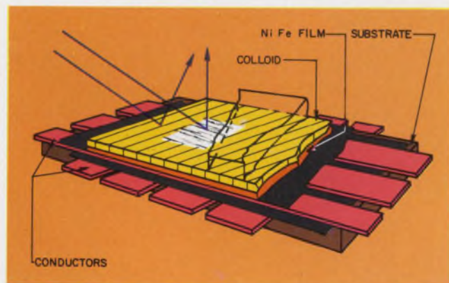
Magneto-optic display acts similarly to a diffraction grating. Display reflects light from external source. Magnetic particles create strain lines.
