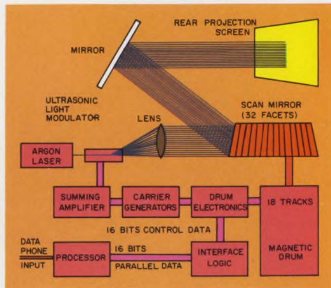
Block diagram of TI's large-screen laser display , which projects alphanumeric and graphics generated by computer software.
