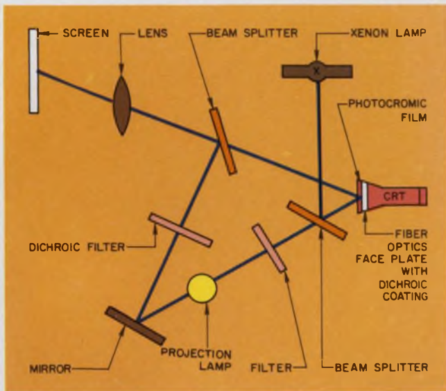
Simplified schematic of photochromic film system being developed for large-screen projection by Army Electronics Command at Fort Monmouth, N.J.
