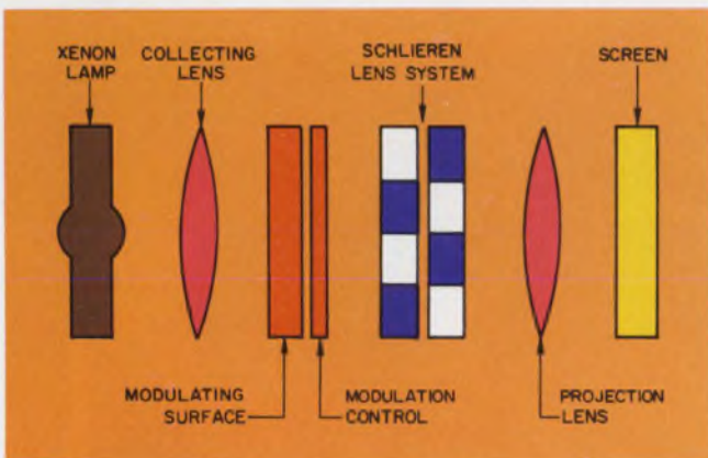
Light-valve display requires a 2-to-4-kW xenon lamp. The light is modulated on a fluid surface and passed through Schlieren optics to a screen.
