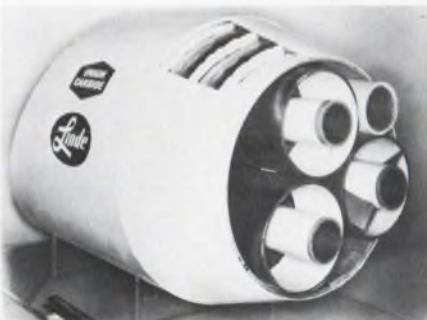
Mockup of superconductive cable. Three of the pipes within the cable would carry electricity. The fourth would carry liquid helium.
