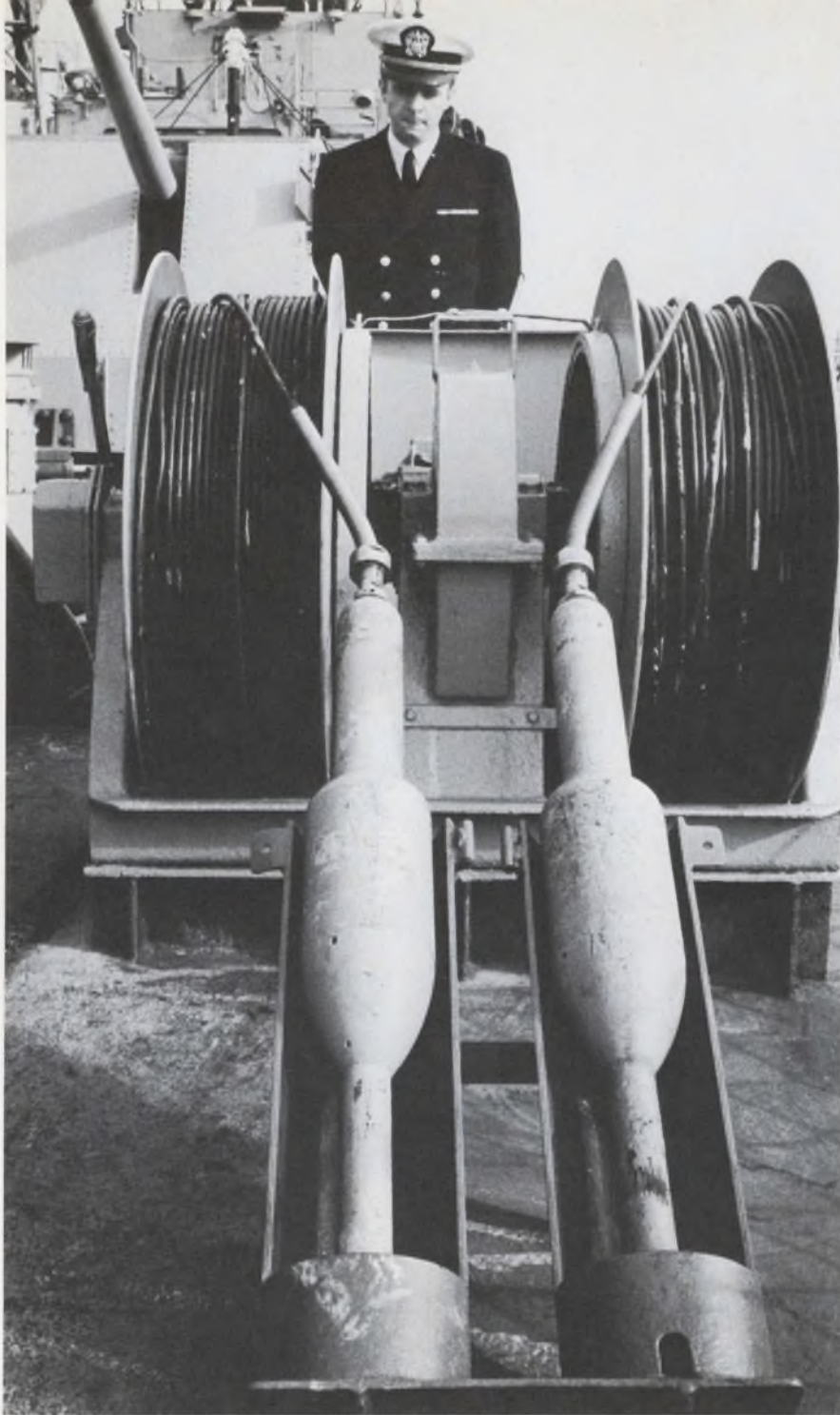
To mislead enemy sonar, these decoys, called Fanfare, are reeled out to a considerable distance behind the ship, where they put out more destroyer-like noise than a real destroyer. Hopefully, they will draw the enemy fire.
