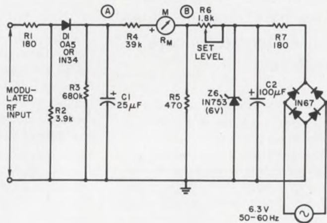
Peak sensing circuit measures rf carrier and modulation-depth level.
