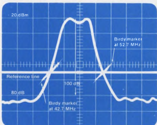
Typical display of narrow band amplifier response indicating 70 dB bandwidth (sensitivity, 20 dB per division)
