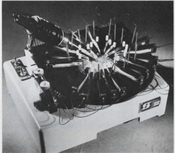
Probing system for thick- and thin-film hybrid assemblies covers 4-in. diameter substrates, p. 340.
