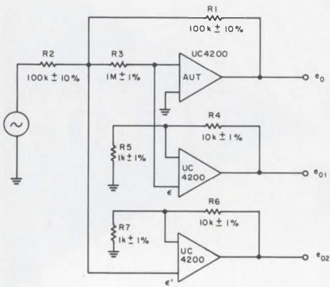
Input impedance of the amplifier under test (AUT) is a function only of resistance R_3 and the output voltages e_{01} and e_{02} .
