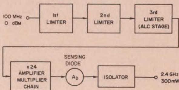
5. Input power variations are reduced by preceding the level-control stage with two stages of limiters. The amplifiers that follow the alc stage must be linear for the loop to have a linear control characteristic.
