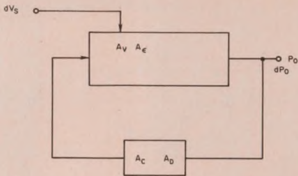
2. Power supply ripple can be analyzed with this simplified block diagram.
