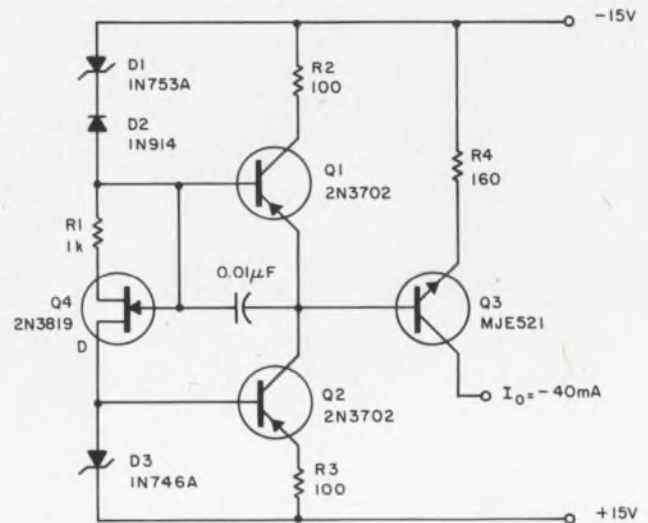
Constant current flows in the collector circuit of Q3, despite variations in the load and power supplies.
