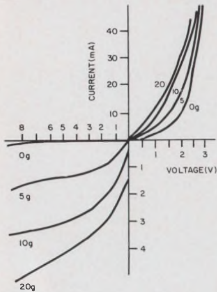
Large changes of current occur when stress is applied to the pressure-sensitive diode.
