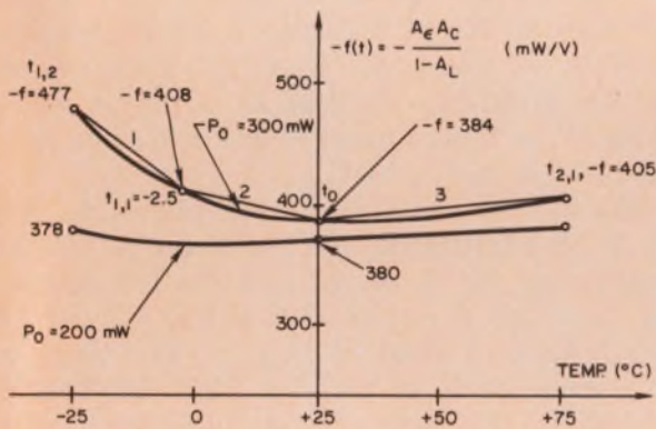
10. Graphical techniques are used to solve for the linear temperature drift when low loop-gain makes the drift equation coefficient a function of temperature.
