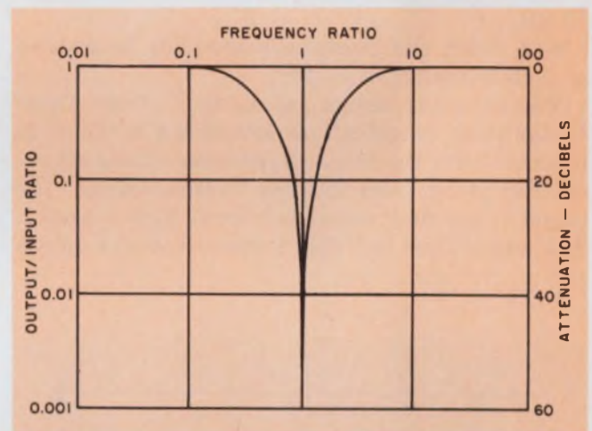
2. Symmetrical null characteristic of a notch network is shown here for a symmetry parameter of m=1.
