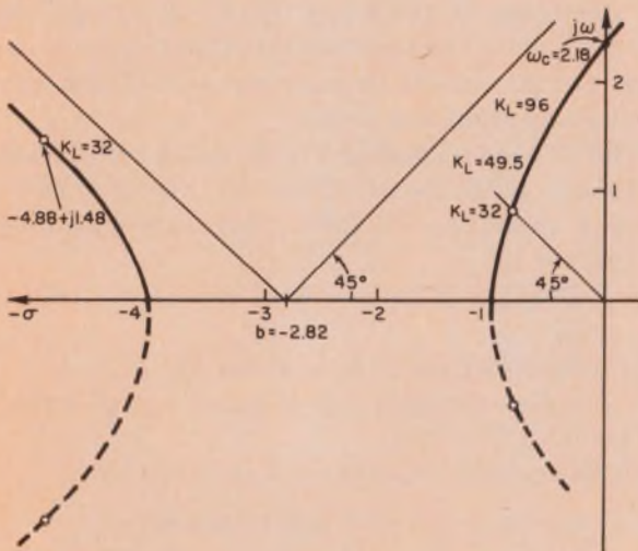
9. This root-locus plot is intersected at K_L=32 by the \theta=45^\circ line. The locations of the four closed-loop poles are shown as small circles.
