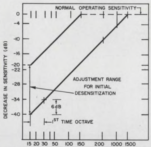
TIME (MEASURED FROM SYSTEM TRIGGER IN MICROSECONDS)
