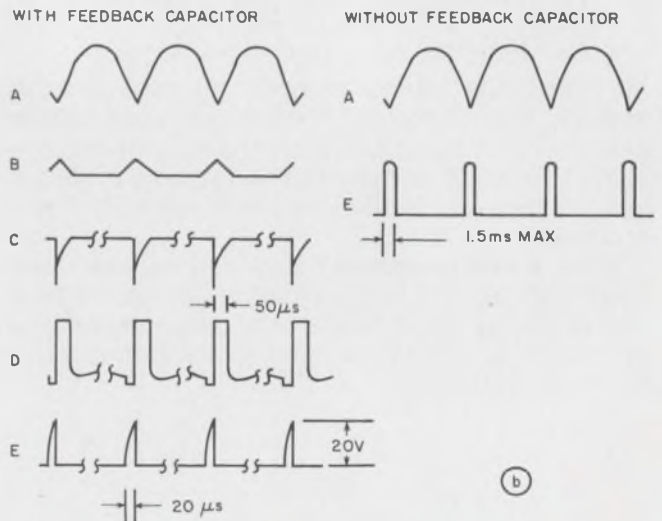
Each zero crossing of the rectified ac produces a narrow output pulse at point E.
