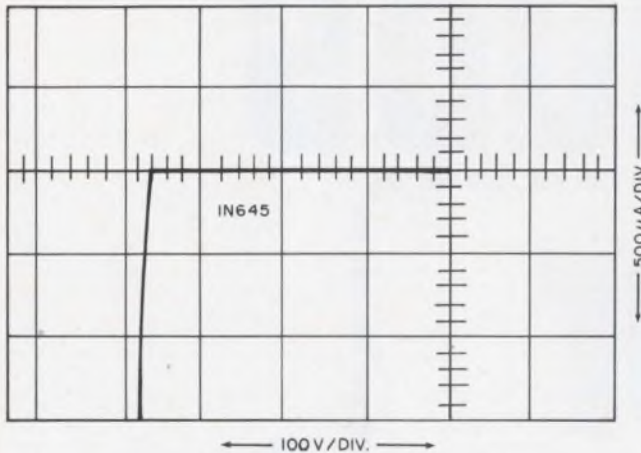
2. Traces demonstrate the versatility of the improved diode curve tracer.
