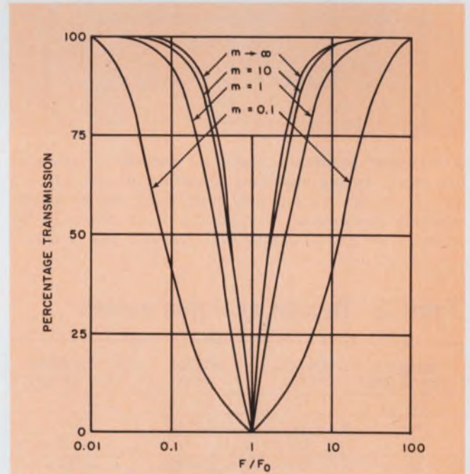
3. Notch sharpness increases as the value of symmetry parameter m is increased.
