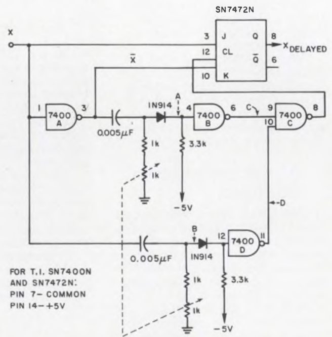
1. Circuit functions as delay line for digital signals.
