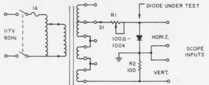
1. Diode curve tracer can be built from miscellaneous "junk box" parts.
