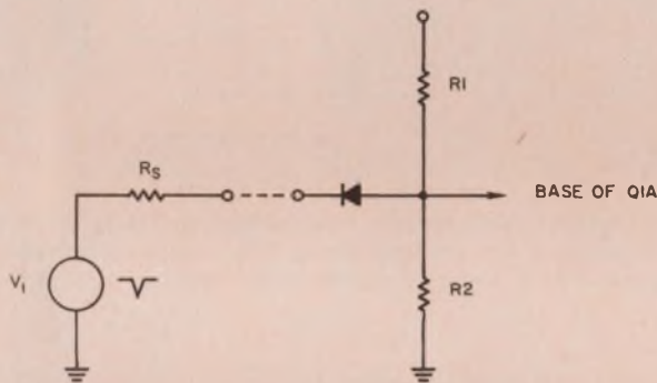
3. The diode isolates the loop from the loading of the pulser so that the natural response of the loop, alone, can be measured.
