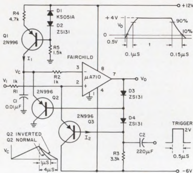
Output is delivered from this monostable circuit when an input trigger causes voltage V_c to rise above V_1 .
