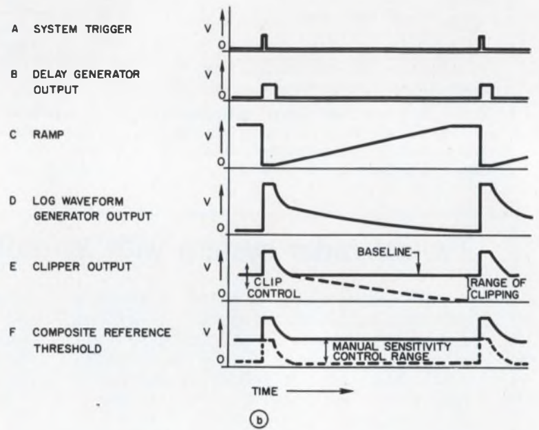
5. The comparison waveform generator (a) includes an adjustable delay to provide time coincidence of the system and the manual sensitivity control. Waveforms at various points are shown in (b).
