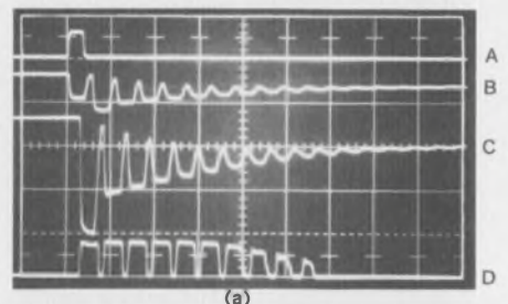
Fig. 3. Waveforms on unterminated (a) and terminated (b) 20-foot length of twisted pair.
