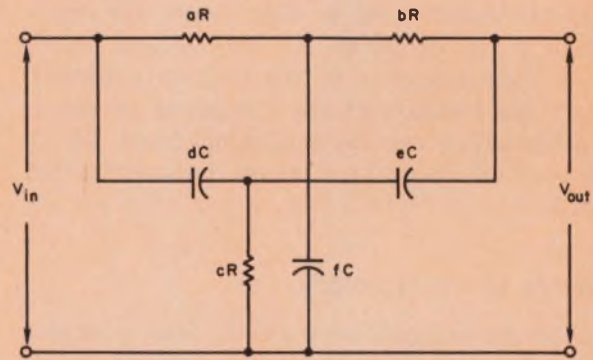
1. Component values of the parallel-T network can be expressed by the coefficients a through f.
