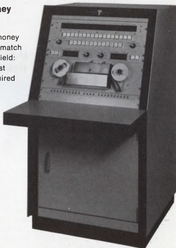
OMNITESTER™ 1000 CIRCUIT TESTER
