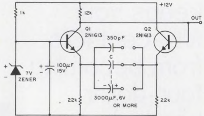
3. Input voltage changes produce output frequency changes in this VCO version of an astable multivibrator.
