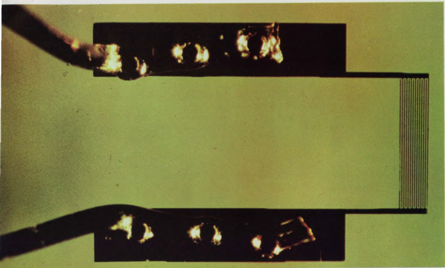
Surface wave transducer fabricated of "gold fingers" on a substrate of lithium niobate operates in the 400-to-500-MHz region. The spacing between the fingers is five
