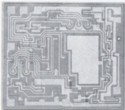
Self-compensated monolithic operational amplifier , developed by Motorola Semiconductor, is contained on a 56-mil-by-63-mil wafer.
