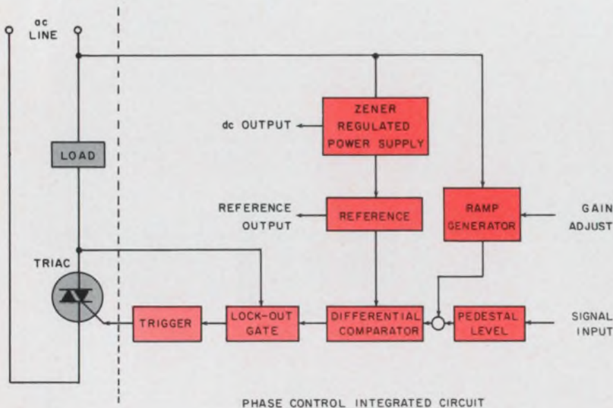
High-gain integrated trigger-circuit, developed by General Electric, is designed for proportional power control applications.
