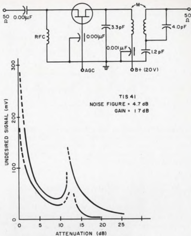
1. The cross-modulation performance of a junction FET (TI S-41) is shown here as a function of bias level. The ordinate shows the amount of 30% modulated interfering signal (at 188 MHz) needed to produce 1% of cross-modulation on the (200-MHz) carrier.
