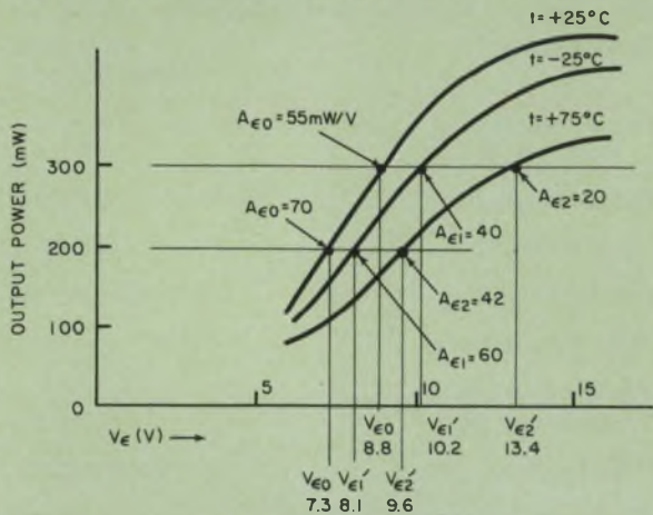
6. The temperature sensitivity of the rf chain is shown here under worst-case conditions. The input power is -3 dBm, and V_{cc} = -24 Vdc.
