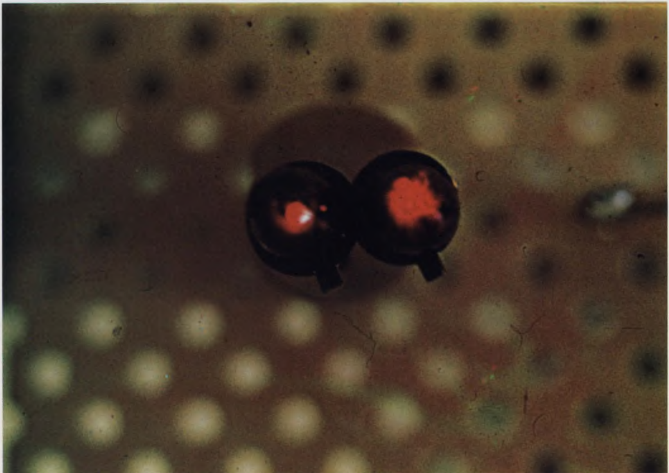
Improved red-light emitting GaAs diode (right) , developed by Monsanto (Booth 2F39), has a typical brightness of 1000 foot lamberts at 50 MA. The old diode (left) has a
