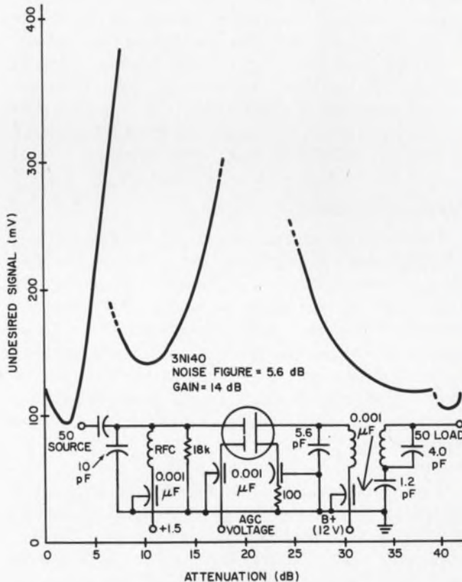
2. This double-valued cross-modulation curve was obtained from a dual-gate MOSFET (3N140). The curve is double valued because, at some points, the amount of undesired signal required to cause 1% of cross-modulation was high enough to change the bias level.
