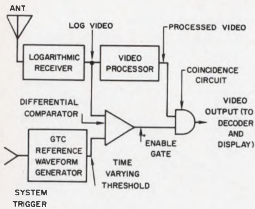
3. Video comparator arrangement for GTC/STC permits the GTC function to be performed at the receiver output rather than at the rf/i-f section.
