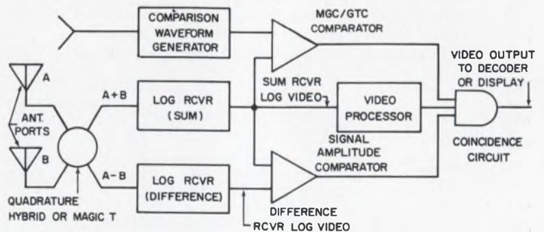
6. Dual-channel receiving system using GTC and manual gain control permits beam sharpening by comparing amplitude of signals received through separate ports. Only the amplitude transfer characteristics of the two receivers require matching, which is a simple matter with the log receiver.
