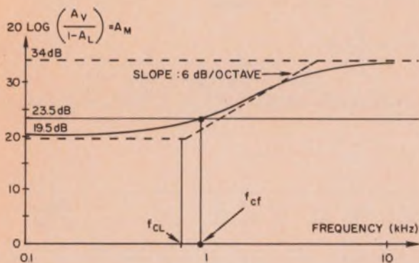
11. Eliminate line ripple by choosing a line filter whose cutoff frequency is < f_{cf} . In this case, with A_M specified as 23.5 dB, with A_L = -4.7 V/V and with A_V = 50 mW/V, f_{cf} = 920 Hz.
