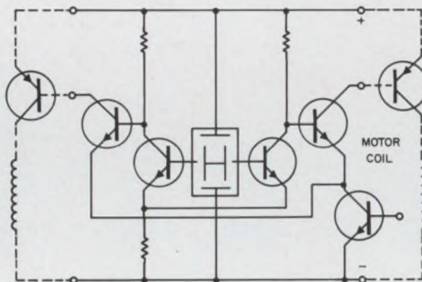
Integrated circuit with a Hall element is used as a switching circuit in a dc motor. It's fabricated by Philips Research Laboratories.
