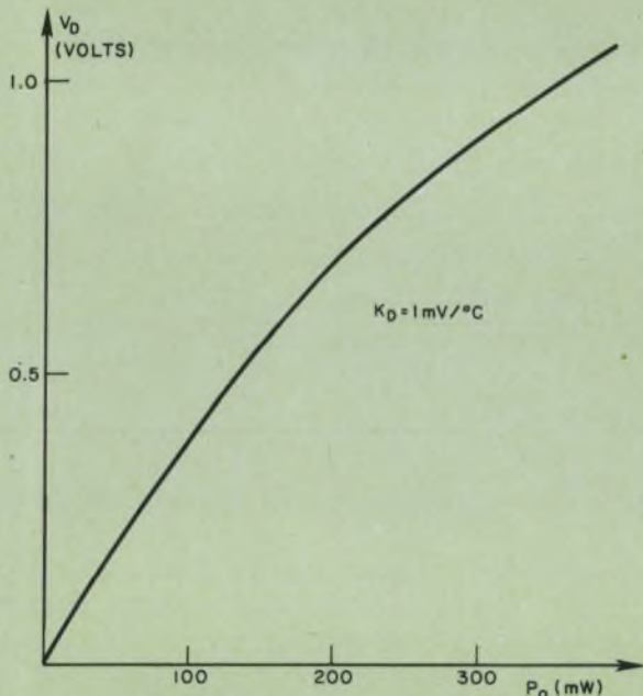
7. The sensing diode transfer constant, A_D , is given by the slope of this curve of V_D vs P . The slope at 200 mW is 1/400 V/mW; at 300 mW, 1/500 V/mW.
