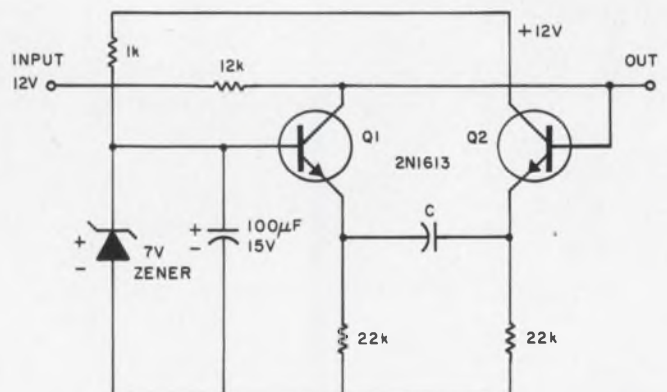
2. Wide frequency range is possible with this astable configuration by changing the value of capacitor C. Frequency coverage can exceed 7 decades.
