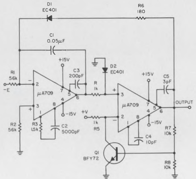
2. Two monolithic operational amplifiers are used in a practical version of the converter.
