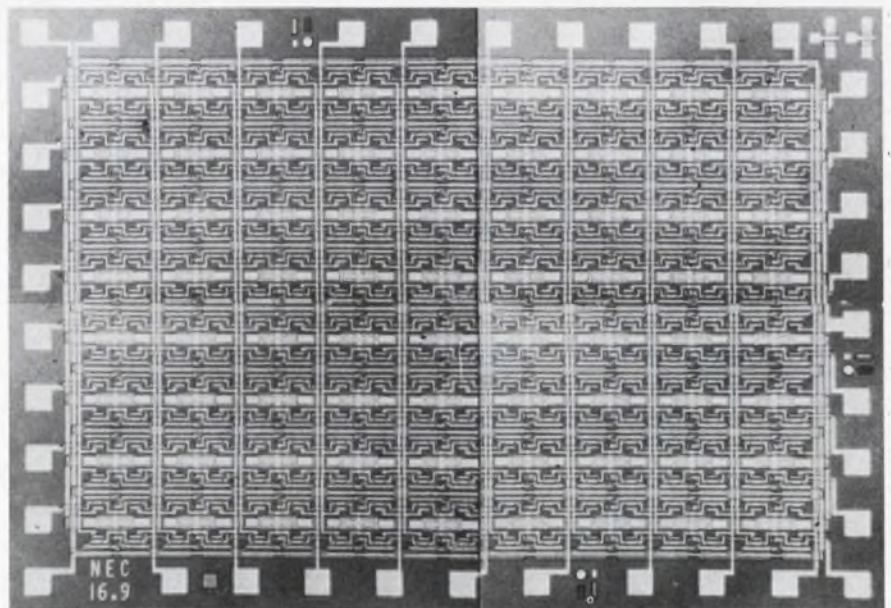
144-bit LSI memory chip, constructed by Nippon Electric Co., has a 30-ns read-cycle time and a 40-ns write cycle time.
