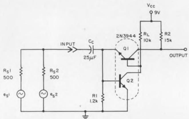
Exceptionally low input-impedance makes the input of this amplifier an excellent current summing junction.
