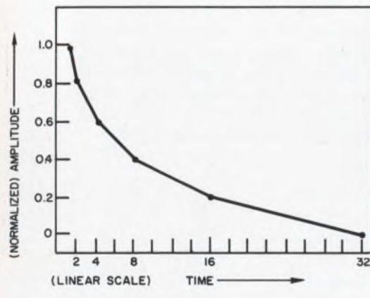
4. The GTC reference waveform is logarithmic (a) to meet the receiver amplitude transfer characteristics as shown in Fig. 1. The waveform shown on a linear time base appears in (b).
