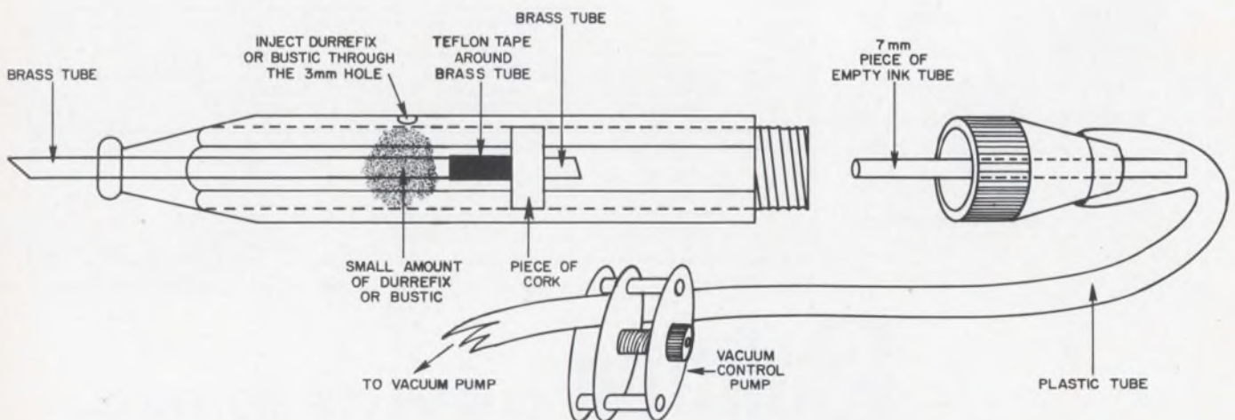
Common ball-point pen can be converted into a vacuum pencil by following the steps illustrated.
