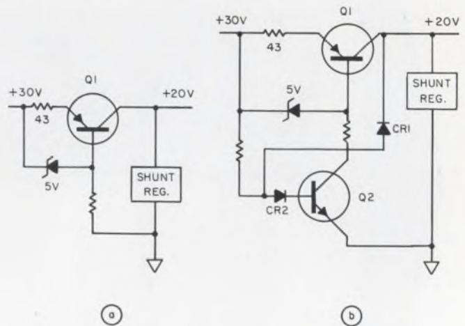
Shunt regulator with active current source (a) is susceptible to accidental shorting to ground. Addition of transistor Q2 (b) provides the required protection without the need for a heat sink and high-wattage current source.
