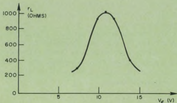
8. Tuning is critical in determining the location of the peak in this curve of r_L vs V_e . The peak is near the value of V_e at which the alc stage is tuned.
