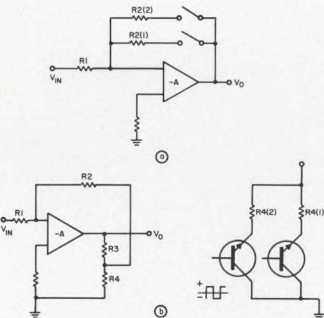
Transistor switching to program a power supply which uses operational amplifiers is possible when a standard circuit (a) is modified as shown (b).
