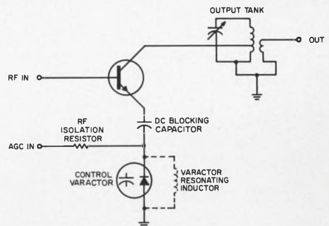
Varactor controls gain without contributing distortion. Gain control range can be extended by resonating the varactor.
