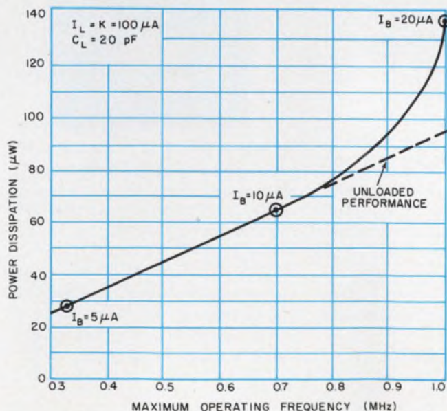
5. Power-vs-frequency plot reveals that increasing power beyond 140 \mu W will not improve frequency response for a given circuit and the load capacitance.
