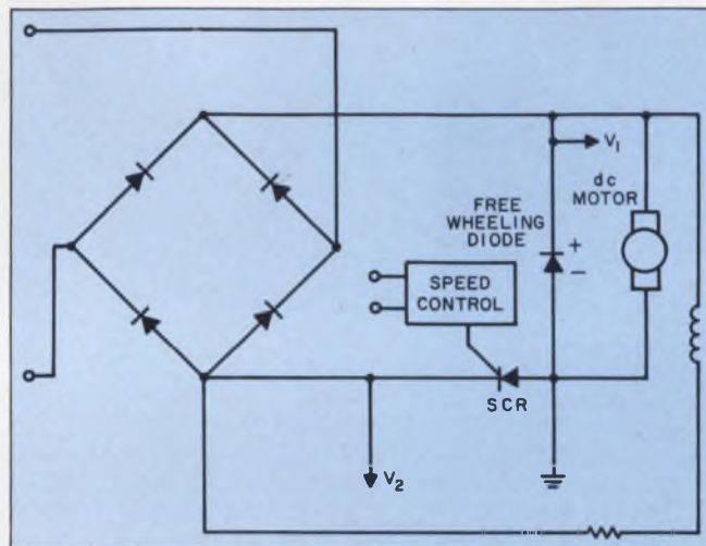
1. Turn-off time was incorrectly specified for this motor-control SCR circuit, so the devices were returned to the vendor as functional failures. But the culprit turned out to be a too small reverse bias in the circuit.
