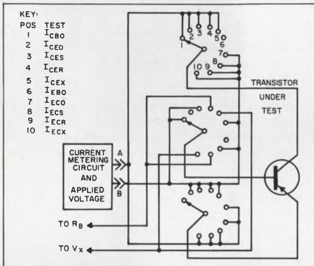
18. All ten leakage current measurements can be performed by placing a multiposition, three-deck wafer switch between the unit under test and the rest of the system. The switch can be solenoid-driven.
