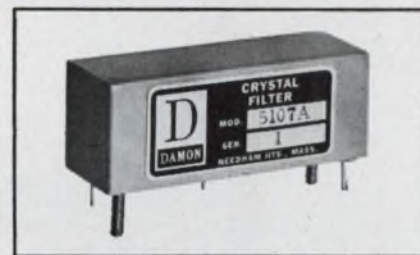
Typical Contiguous Comb Crystal Filter, Model 5107A is 1\frac{1}{16} " L x \frac{3}{16} " W x \frac{7}{8} " H.
