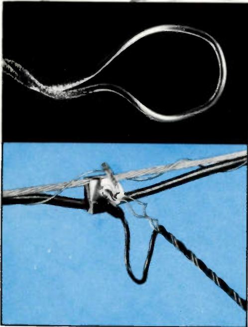
TELEGRIP for attachment of RG 59/U Coaxial Cable at pole, tap, and house. Neoprene coated stainless steel. Holds full rated strength of the cable.
