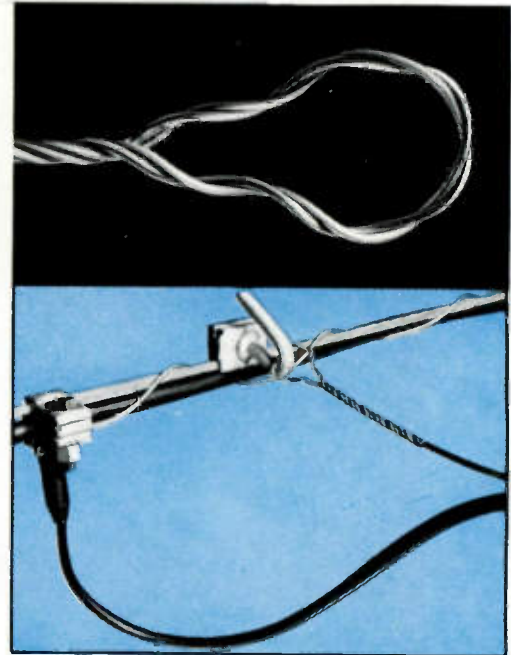
PREFORMED Dead-End provides fast, easy method of attaching Figure-8 Cable. Simply strip the messenger and wrap on the dead-end.
