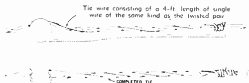
Twisted pair outside distributing wire dead-end.
