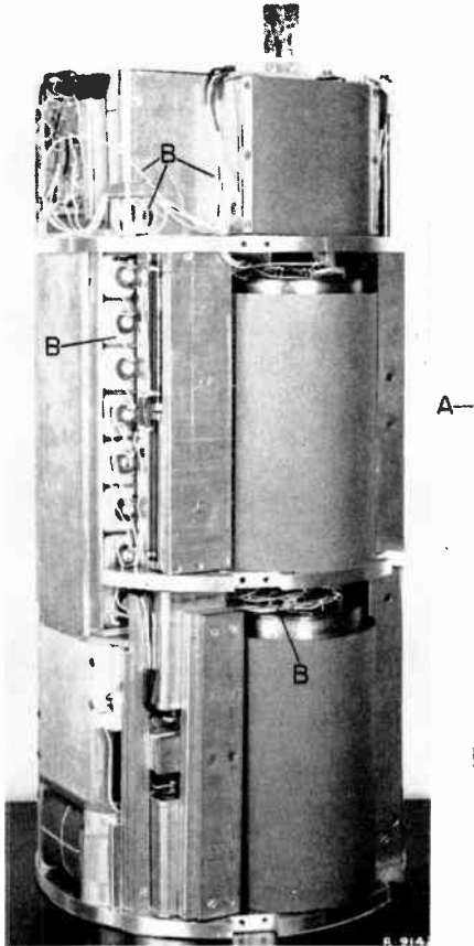
Figure 22. Submerged telegraph repeater with outer steel casing removed "A" shows No. 18 A.w.g. solid silverplated copper conductor insulated with 10 mils of fluorothene employed for the wiring at "B"
