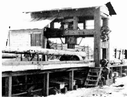
Machine for incising the ground line section of cedar poles
