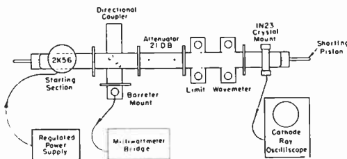
Figure 4. Block diagram of test set
