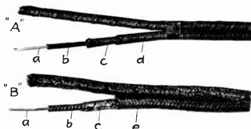
Figure 18. Outside distributing wires "A" City distributing wire "B" Tree wire
