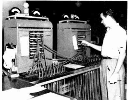
Incoming and outgoing concentrator turrets and cords associated with printer-perforators and distributor-transmitters (New York)
