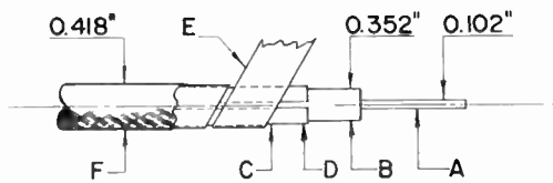
Figure 20. Shielded line wire
