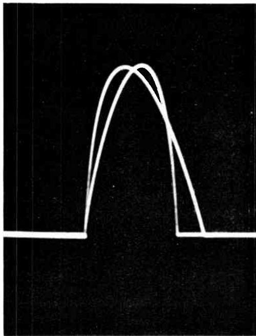
Figure 5c. Normal power characteristic of klystron for one sweep of voltage through the oscillating range for a complete cycle of voltage change
