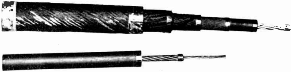
Comparison of armored and nonarmored cable
