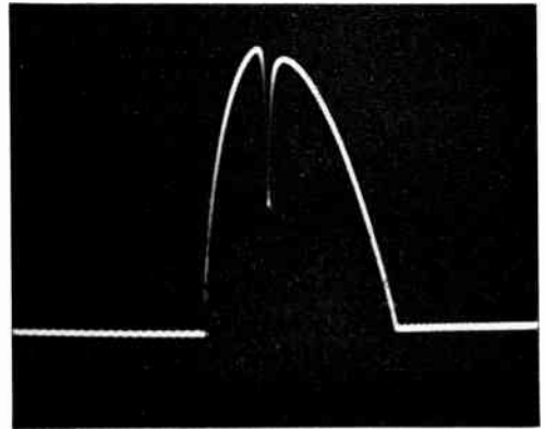
Figure 5b. Normal power characteristic of klystron for one sweep of voltage through the oscillating range with dip caused by frequency meter, the klystron adjusted to deliver maximum power at the particular frequency
