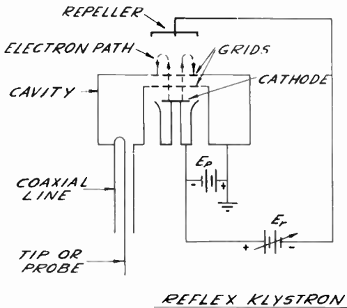
Figure 2. Theory Diagram of Klystron 2K56
