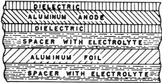
Figure 3. The various layers of an electrolytic capacitor
