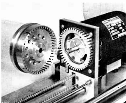
Figure 5. Tone generator
