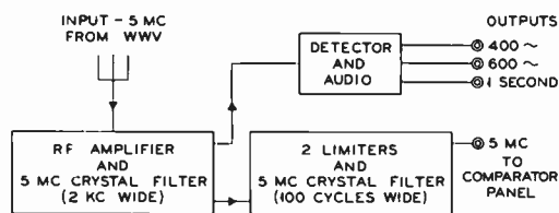
Figure 2. Block diagram of the radio receiver
