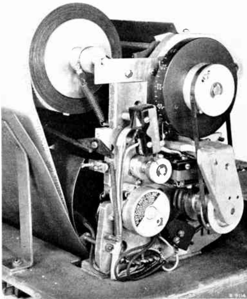
Figure 6. Feed meter mechanism
