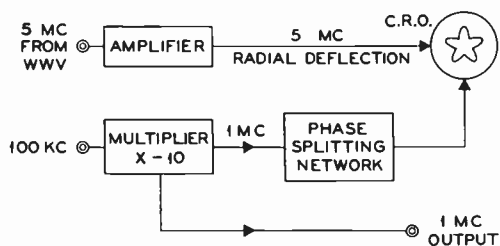
Figure 3. Comparator panel
