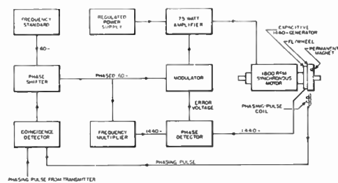
Figure 7. Recorder drive and phasing systems
