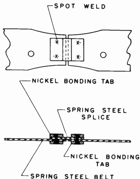
Figure 7. Welded splice—stylus belt
