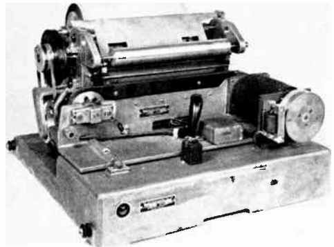
Figure 2. High-Speed Recorder—cover removed
