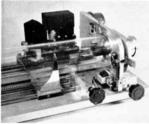
Figure 8. Solenoid-operated lock, and positioning controls
