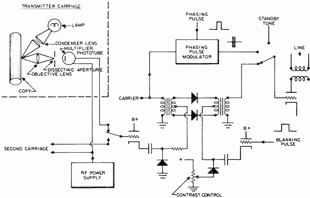
Figure 2. Transmitter scanning system
