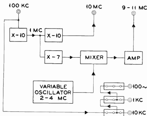
Figure 5. Frequency divider panel
