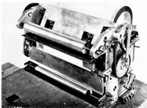
Figure 3. Paper-feed mechanism
