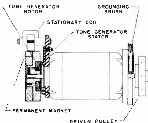
Figure 9. Stylus motor drive
