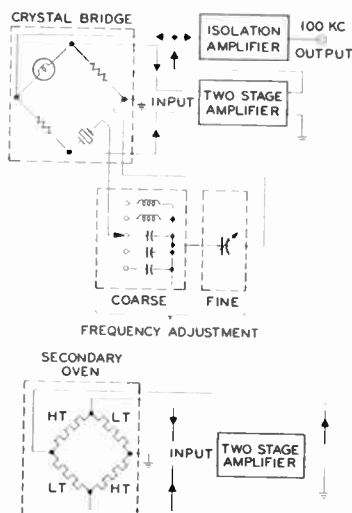
Figure 4. Circuit arrangement of frequency standard oscillator panel
