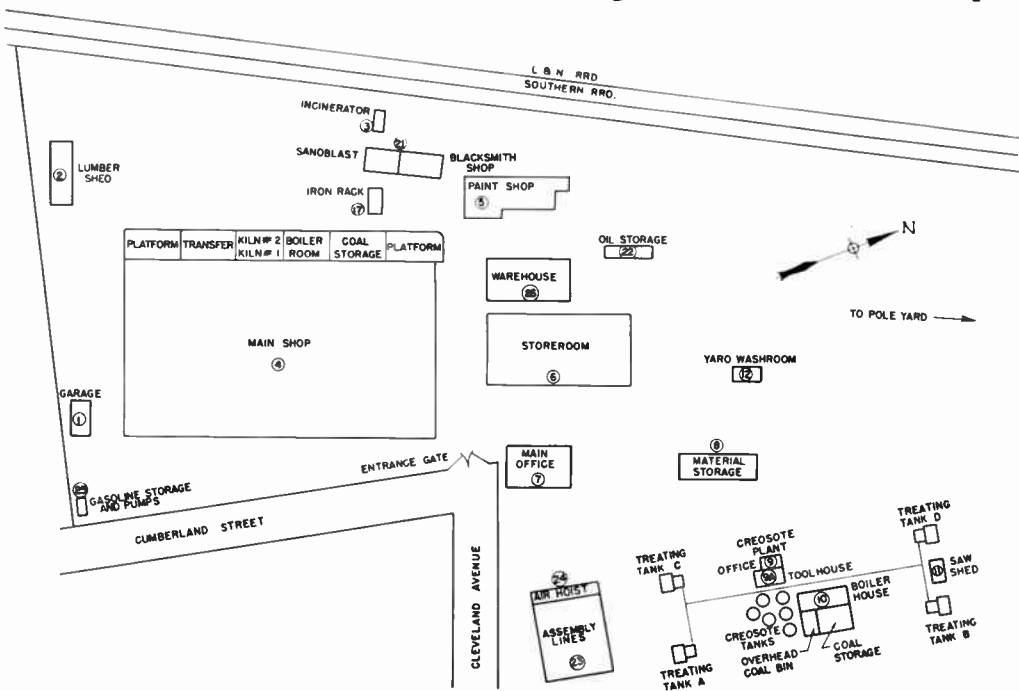
Figure 2. Layout of Chattanooga Works
