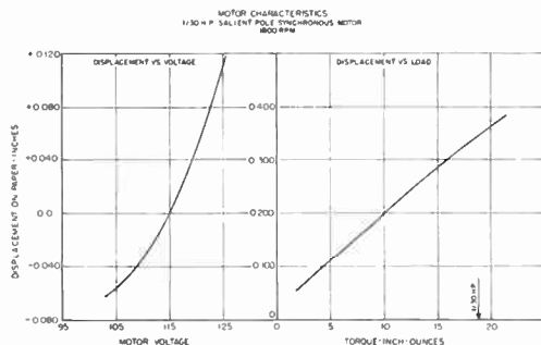
Figure 5. Motor voltage and load characteristics
