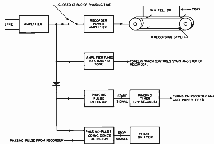
Figure 11. Recorder scanning and signal detection
