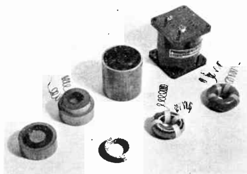
Figure 1. Comparison of filter coil having two-piece molded core, copper tube shield and case (above) with toroid-core coil (below, right) shows size reduction
