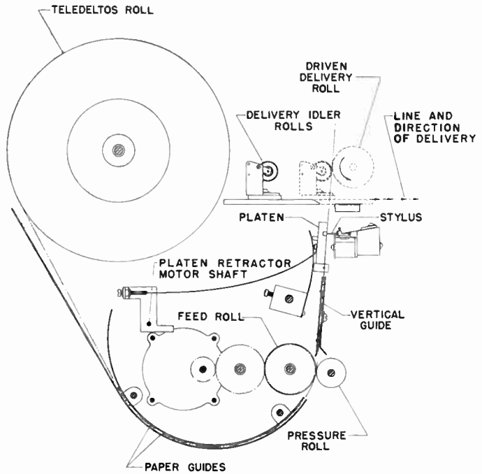
Figure 5. Paper course
