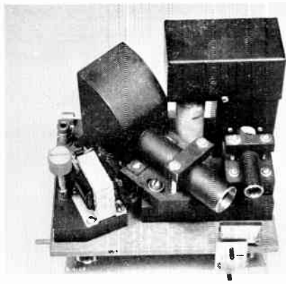
Figure 7. Carriage—top view
