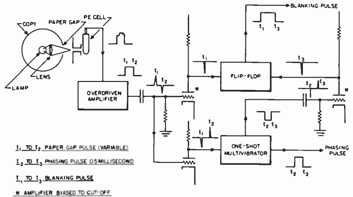
Figure 10. Transmitter pulse circuitry
