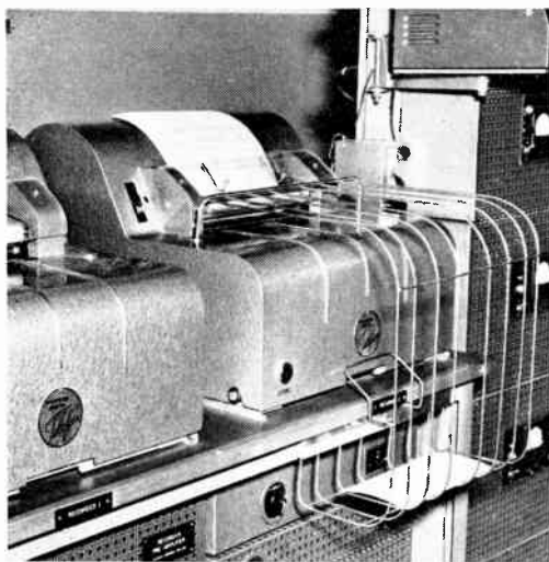
Figure 10. Receiving table
