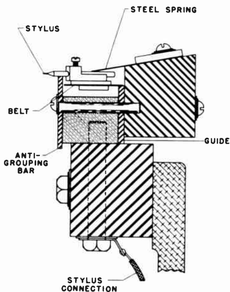
Figure 8. Cross-section of belt and guides
