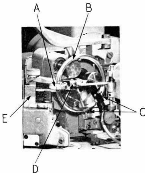
Figure 4. Coil clamp and shuttle of toroid winder
