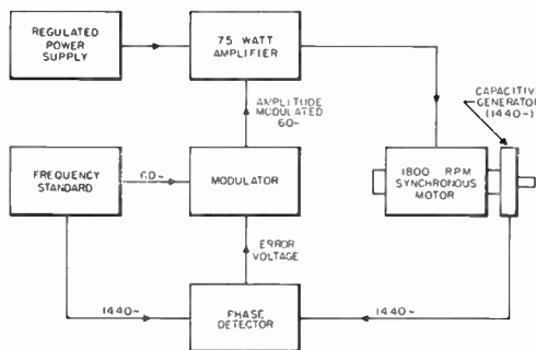
Figure 6. Transmitter drive system
