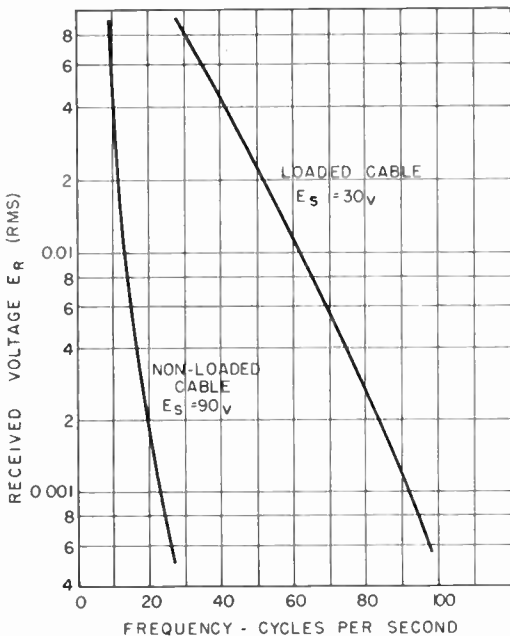
Figure 1. Attenuation Curves
