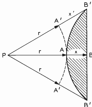
Figure 2. Convex lens
