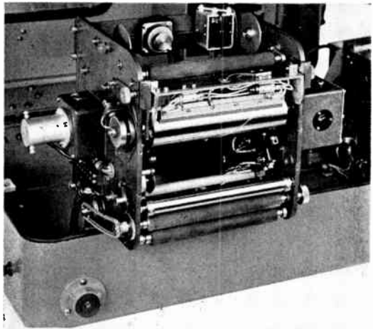
Spiral wire-and-blade recorder assembly of Bludworth Marine echo sounding equipment
