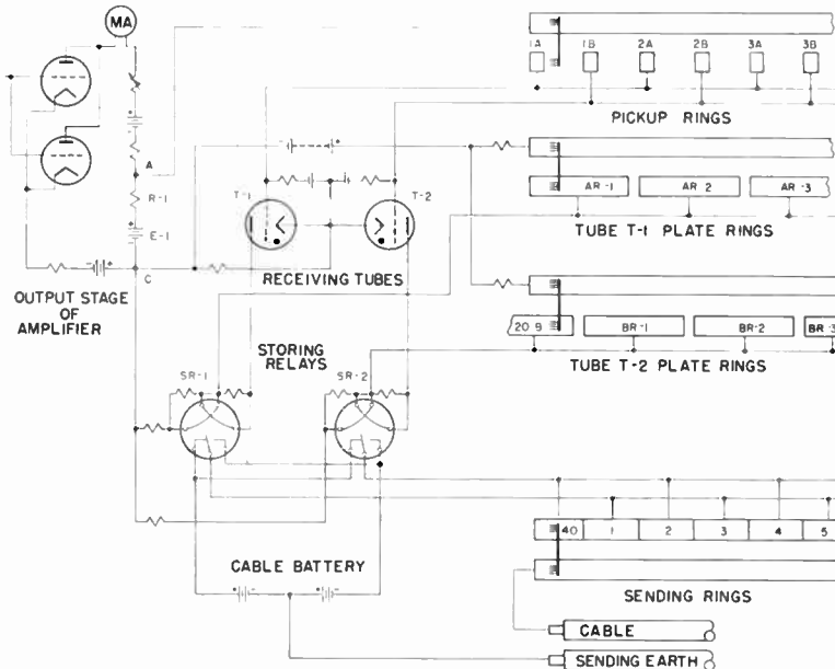
Figure 6. Receiving and interpolating circuit
