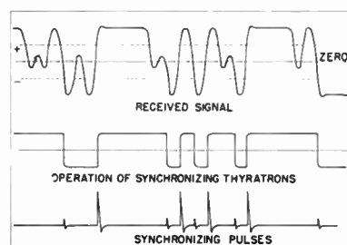
Figure 10. Synchronizing tube signals
