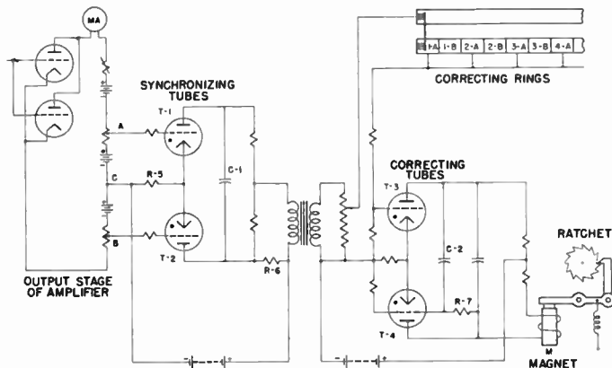
Figure 9. Phase correction control circuits
