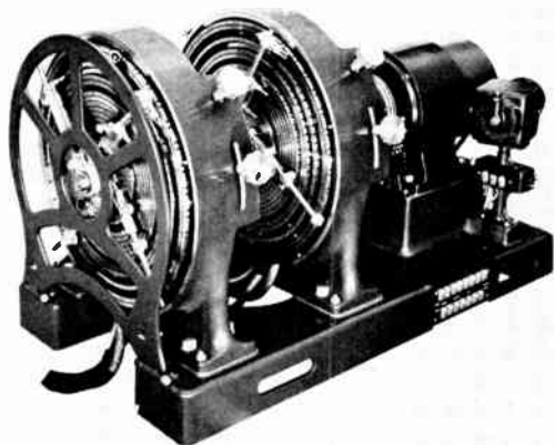
Figure 4. Distributor used with regenerative repeaters
