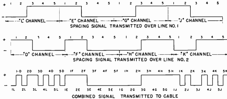
Figure 5. Interleaved signals from two feeder circuits
