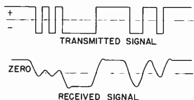
Figure 3. Signal attenuation
