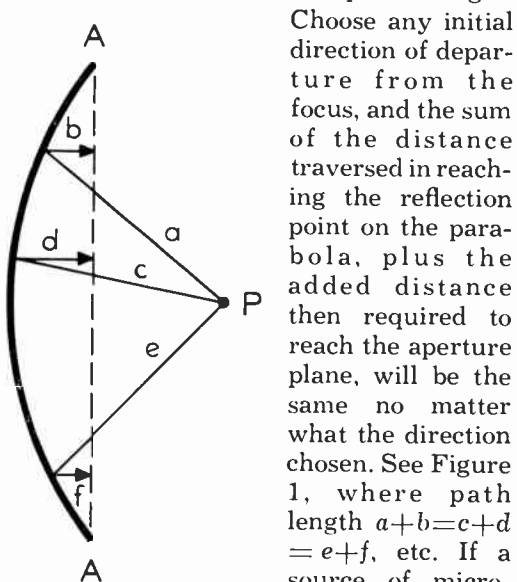
Figure 1. Parabolic reflector
