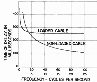
Figure 2. Time Delay Curves
