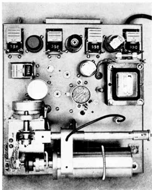
Figure 6. Top view of Deskfax transceiver showing layout of parts
