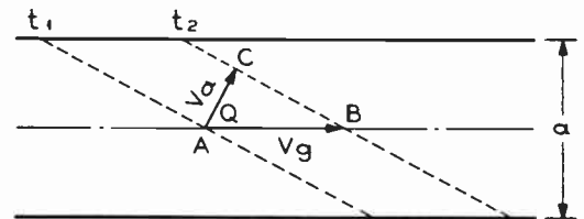
Figure 5. Wave propagation in a wave guide
