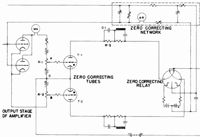
Figure 11. Earth current correction circuits
