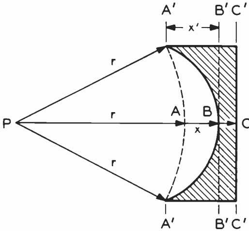
Figure 3. Concave lens
