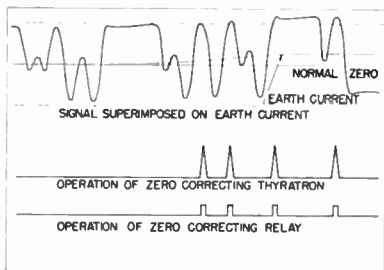
Figure 12. Zero correcting circuits
