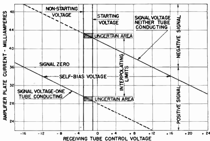
Figure 8. Signal limits chart
