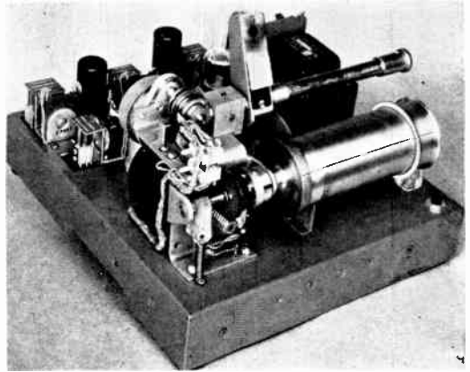
Figure 5. Deskfax transceiver—cover removed
