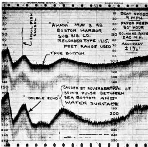
Echo sounding chart depicts harbor bottom
