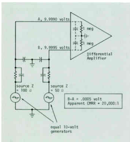
Figure 8. Schematic that shows the small affect on CMMR caused by low-impedance test points compared to that of Figure 7.
