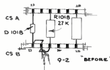
Field Mod Wiring Diagrams
