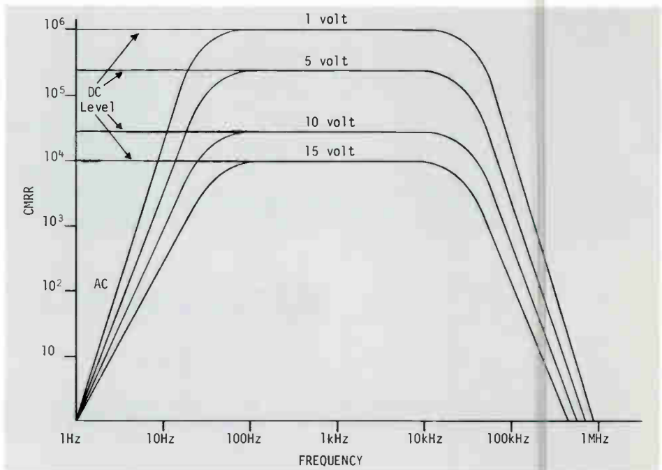
Figure 4. The common-mode rejection ratio related to frequency, voltage level, and input coupling of a typical differential amplifier.
