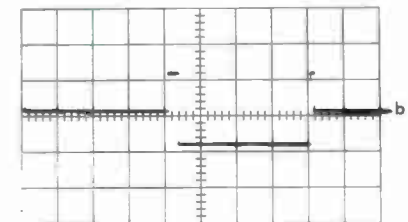
Figure 3. a, Two square waves of different amplitude and coincidental applied to a differential amplifier. b, the difference waveform seen on the crt.
