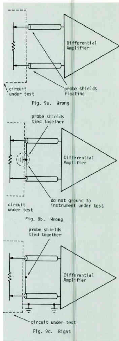
Figure 9. The right and wrong way to connect a differential amplifier into a circuit. The ground shown in c is for safety purposes and not essential to the measurement.
