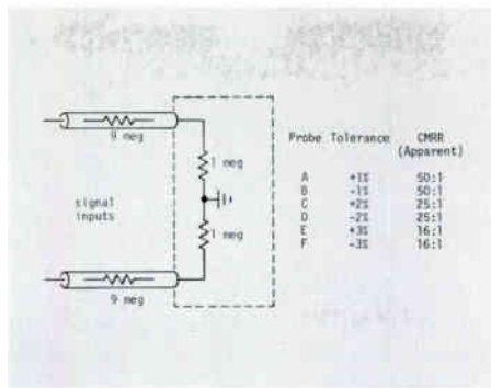
Figure 6. Simplified input circuit and table that shows the change in CMRR (apparent) due to X10 probes that are within 1, 2, and 3% of their attenuation value.
