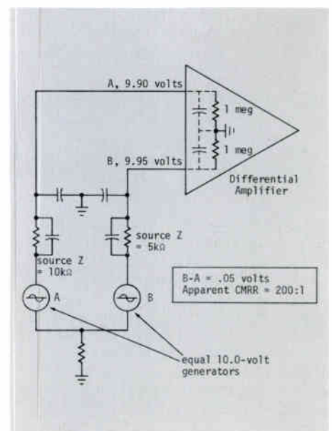
Figure 7. Schematic that shows the relationship of test-point source impedance to the amplifier-input impedance, and also shows the apparent CMRR caused by large value difference between test-point impedances.
