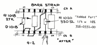
Figure 2. "Before" and "After" sketches showing how to install the 330 Ω resistor R1020.
