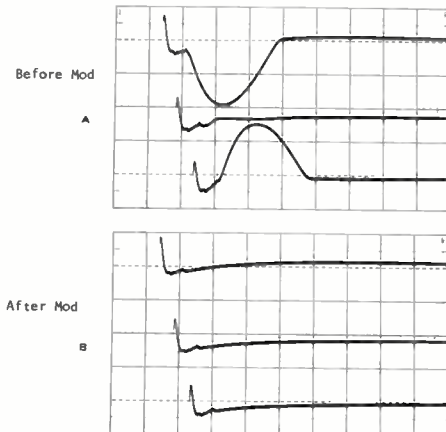
Figure 1. A—Waveform aberration before addition of R1020. B—After addition. Signal Source: 1 Volt Cal, Sweep Rate 1 μs/cm. Type W Unit Control Settings: Vc + 11, INPUT ATTEN 1, DISPLAY A-Vc, MILLIVOLTS/CM 5. (Triple exposure photos.)
