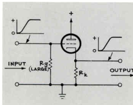
Fig. 5 — Illustrating that the polarity of the cathode-follower output-signal voltage is the same as that of the input-signal voltage—in contrast to the polarity reversal that occurs in the plate-loaded amplifier.
