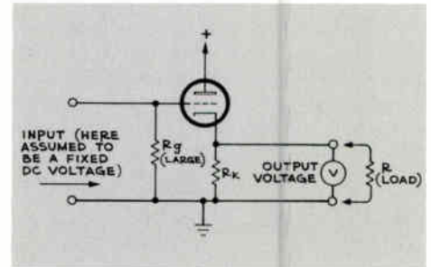
Fig. 6 — Illustrating that the internal output impedance of a cathode follower is small. A given cathode current makes the voltmeter V show a certain dc output voltage (the IR voltage drop across R_k ). If we connect the external load R , we thereby reduce the total resistance in the cathode output circuit. Thus we might at first expect the voltmeter to show a sharply reduced output-circuit IR voltage drop. But this voltage drop is also the negative dc grid-to-cathode bias voltage—so that the tube allows a greater cathode current to flow. Therefore the new output voltage is the IR voltage drop produced by a larger current in a smaller total resistance. As a result, this new output voltage isn't much less than the original voltmeter reading. The fact that the output voltage changes only a little when we connect the load R shows that the internal source impedance of the cathode follower is small.
