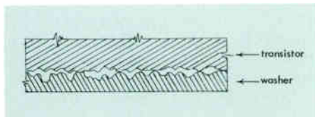
Figure 2. How a magnified cross-section view of the surface might look.
