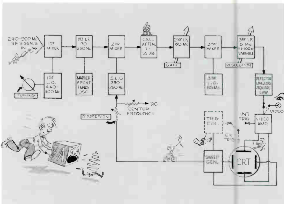
Block diagram of typical Tektronix Plug-In Spectrum Analyzer.
