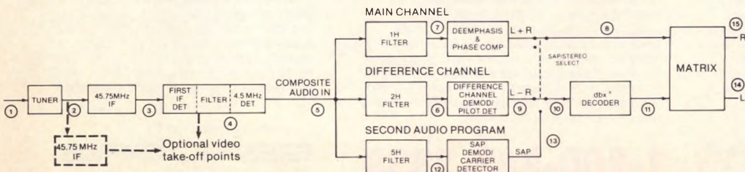
Fig. 1: Phase-locked signals from the ST66 Stereo TV Analyzer let you prove which circuits are working properly from the tuner to the speakers. Isolates defective stages in minutes.
