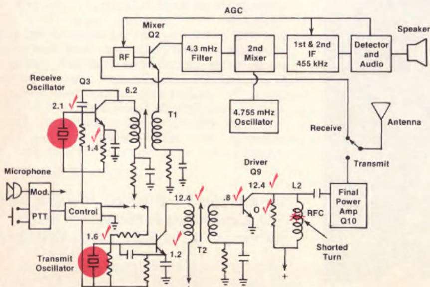
Fig. 1: Proving the crystals good and following the frequency with the Snoop Loop provided positive troubleshooting leads . . . while normal DC voltages failed to head us in the right direction.
