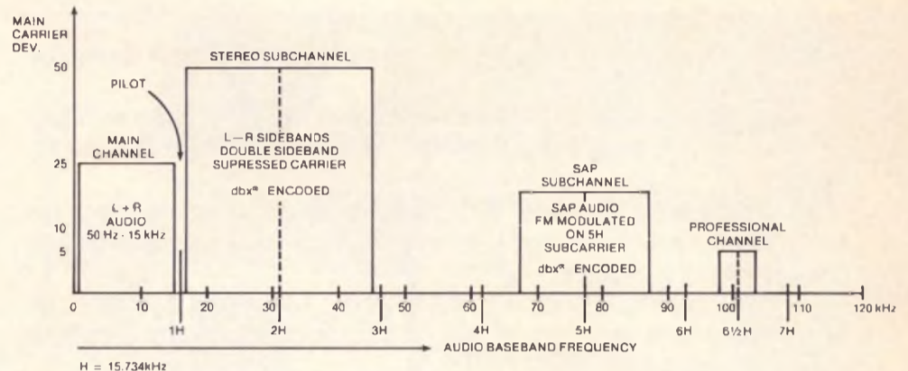
Fig. 2: Each signal will cause an amount of deviation proportional to its amplitude.
