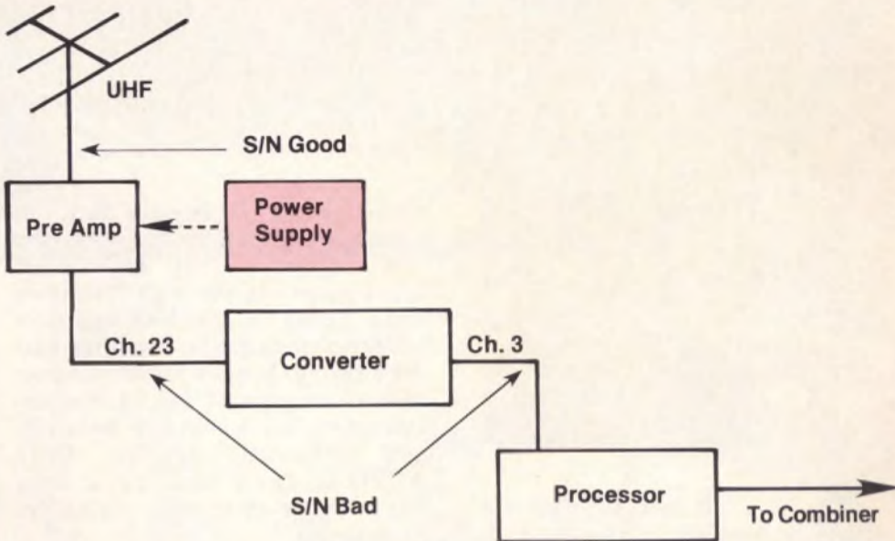
Fig. 8: Power supply ripple decreases picture quality and is often observed on a single channel. This leads you back to the headend.
