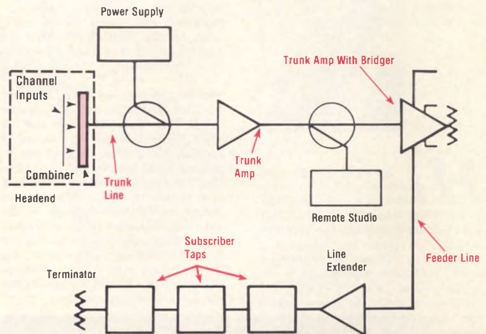
Fig. 2: Performance test key points within the distribution system to detect problems before they affect customer's service.
