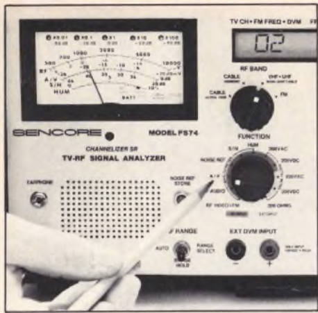
Fig. 4: Testing the video and audio carrier amplitude ratio (A/V).
