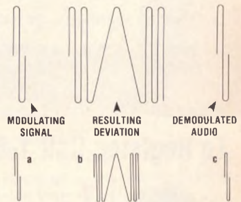
Fig. 3: Decreasing the modulating signal by 1/2 (a), causes 1/2 the deviation (b), which results in 1/2 the demodulated audio (c).
