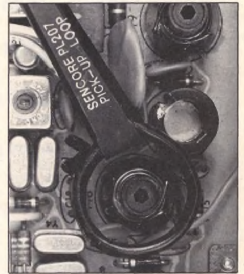
Fig. 3: The Snoop Loop lets you quickly follow the frequency through the multiplier stages in a radio.
