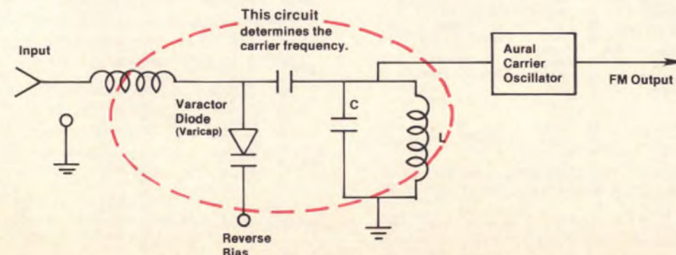
Fig. 1: The carrier frequency is controlled by the varicap diode; the greater the change in bias, the greater the change in frequency.
