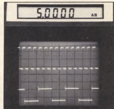
Fig. 5: The frequency ratio function automatically displays the ratio of two waveforms.
