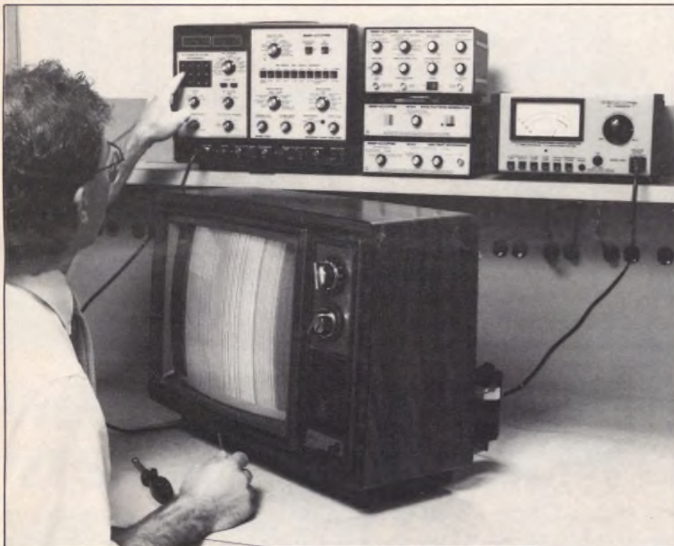
Fig. 3: Inability of the AFT to follow a cable channel offset is immediately apparent from the unstable CRT display with an offset VA62 signal.
