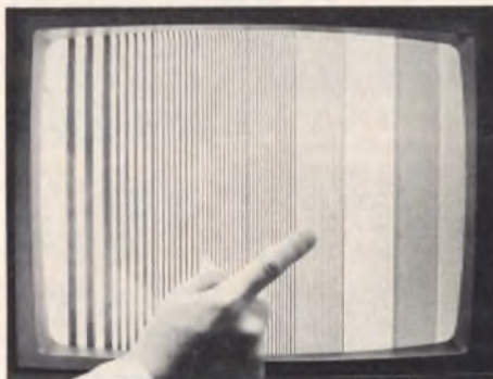
Fig. 1: Sencore's patented Bar Sweep Pattern gives you an instant visual frequency response check to 4.5 MHz.
