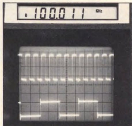
Fig. 2: Automatic frequency measurements to 100 MHz are 10,000 times more accurate than a conventional scope.
