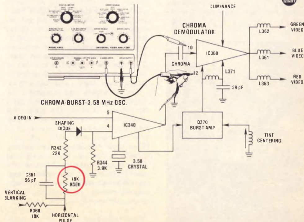
Fig. 3: The VA62 lets you quickly replace IC Chip signals for proof positive chip testing.
