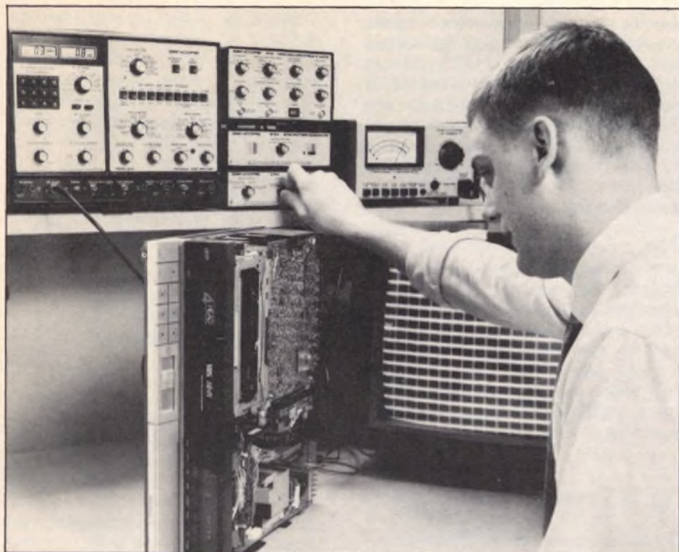
Fig. 8: The VCR head substitution signal lets you know immediately whether the heads are truly the cause of the bad or missing picture from the VCR.
