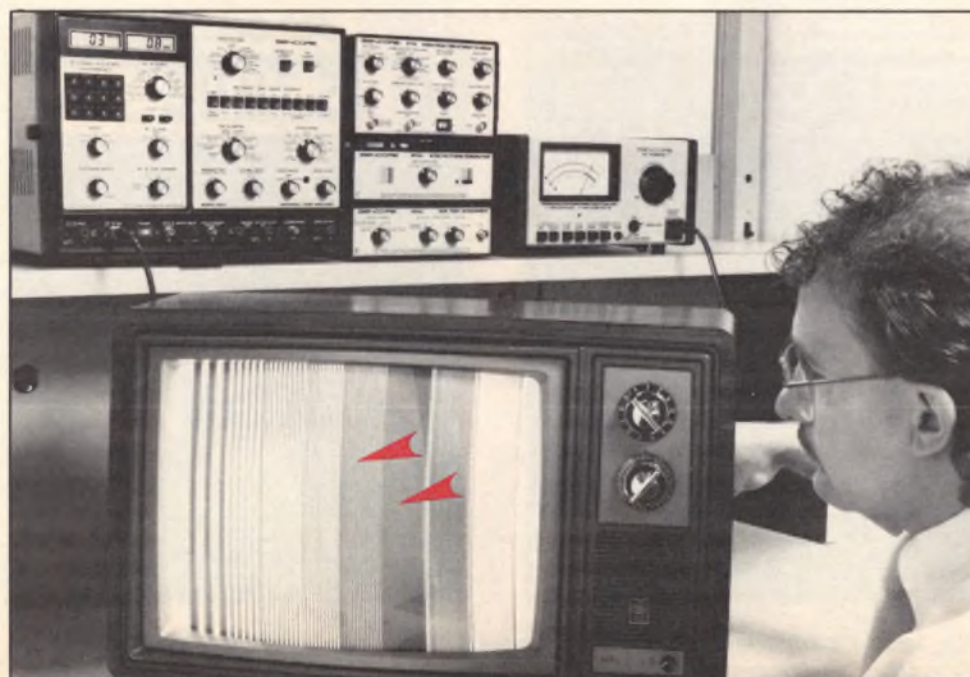
Fig. 2: Dark bars which correspond to video frequencies of 2.5 and 3.0 MHz indicate poor frequency response in luminance channel.
