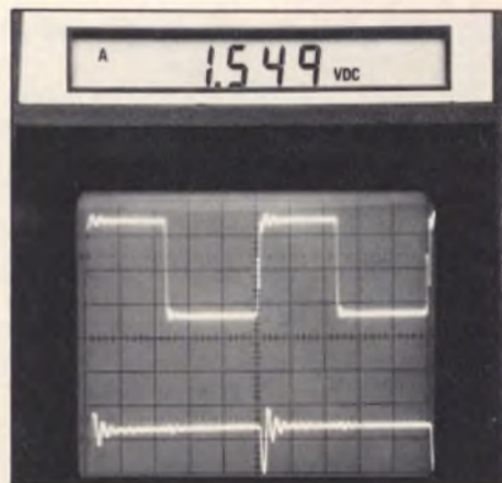
Fig. 3: The DC level of a waveform is displayed simultaneously with the waveform.
