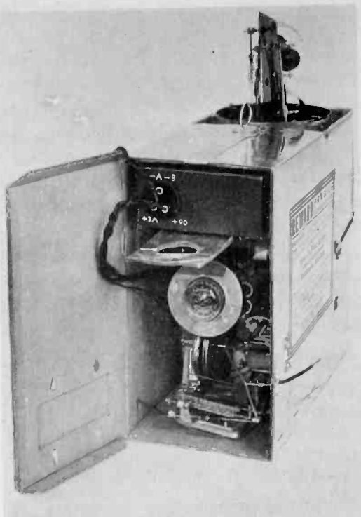
Figure 2. The Radiosonde, Originally Developed for the Navy by the National Bureau of Standards in 1936, Suspended from a Free Balloon, Telemeters Information on Upper-Air Pressure, Temperature, and Humidity. The instrument is in general use by the Navy, Army, Coast Guard, and Weather Bureau for collecting meteorological data employed in weather forecasting, and has replaced the airplane for obtaining information of this type. The radiosonde employs a modulator and oscillator, the ultra-high-frequency output of which is controlled by special resistors that are sensitive to changes in atmospheric phenomena. The changes in modulation frequency are thus measures of the phenomena studied.
