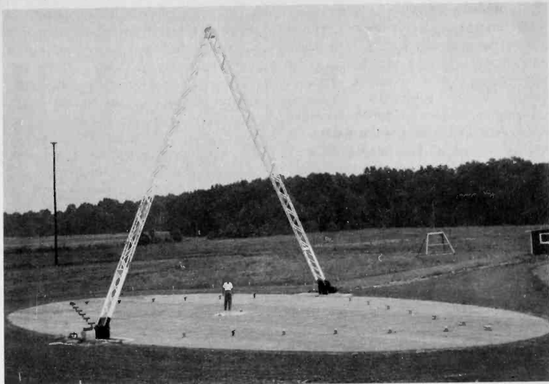
Figure 5. NBS Model Antenna Range. This range is believed to be the largest of its kind designed to measure antenna radiation patterns in the vertical plane. The inverted-V structure supports a self-contained target transmitter at the vertex and is designed to move in a 180-degree arc. The antenna to be tested is placed at the center of the oval-shaped ground plane. The model techniques that are used permit an investigation of antenna characteristics in the 1-to-25-mc. region while actually operating at frequencies between 60 and 1500 mc.
