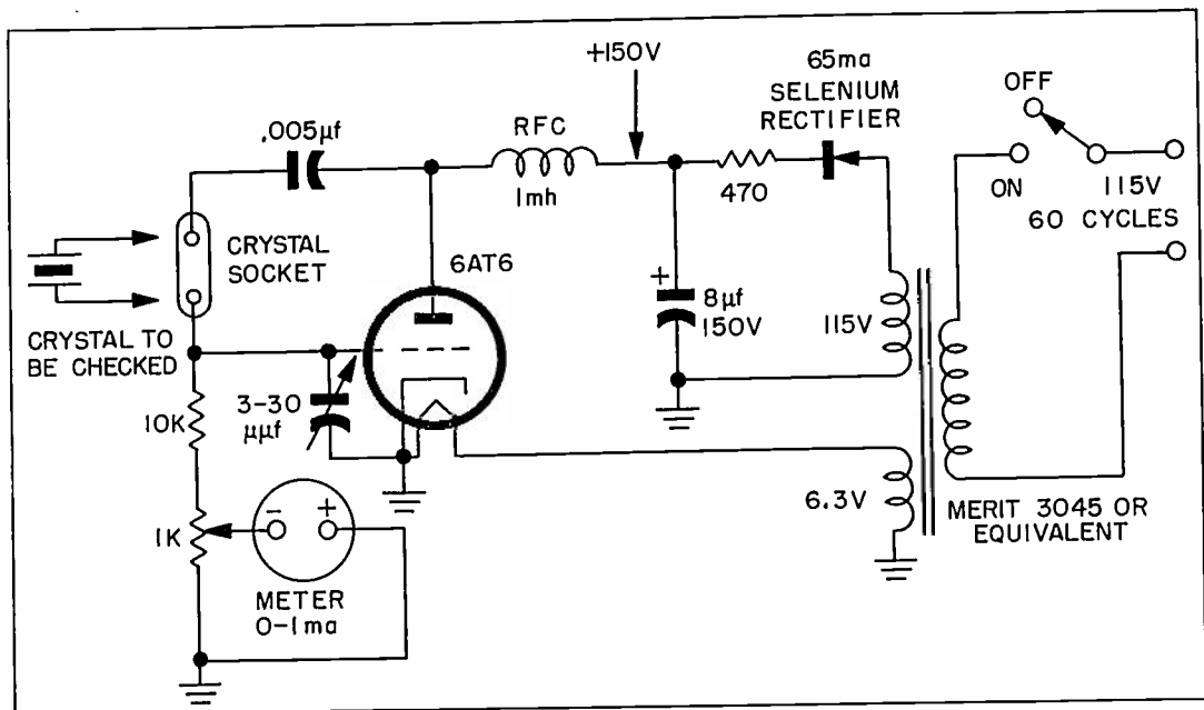
Figure 1. Schematic Diagram of Crystal Checker
