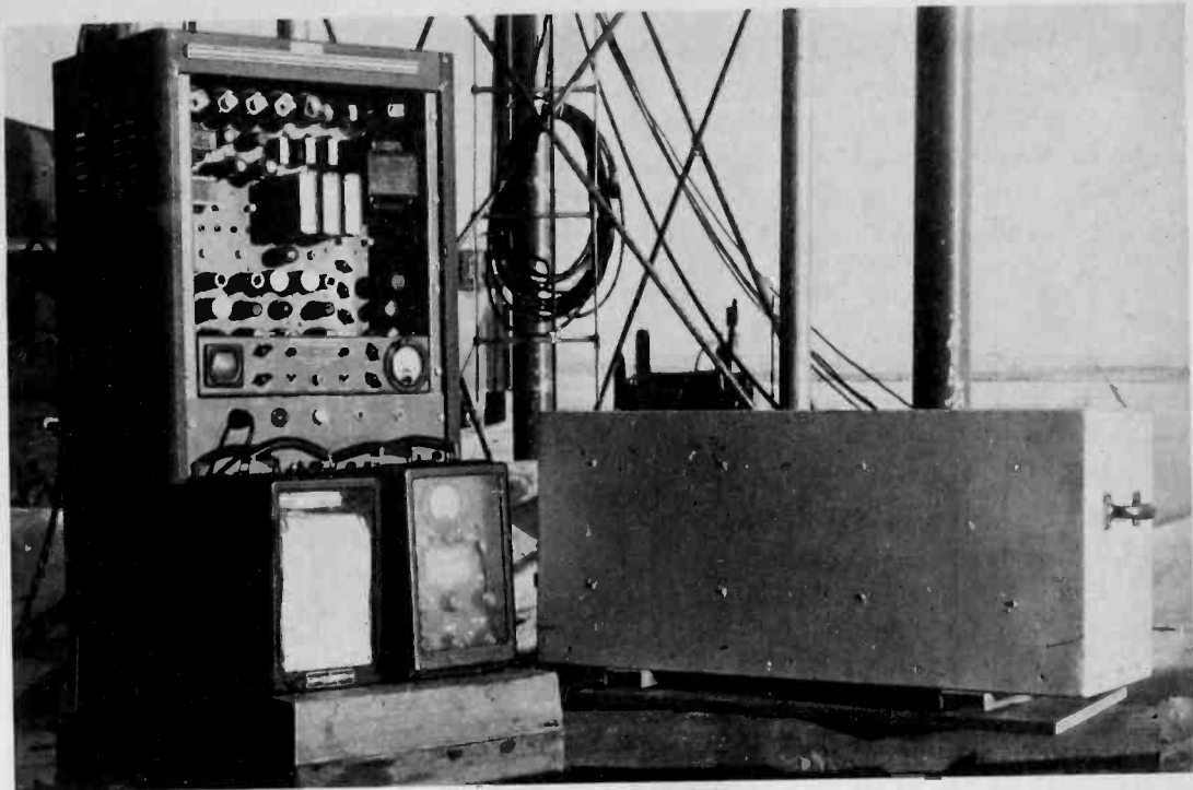
Figure 10. The NBS Microwave Refractometer Employed at a Midwestern Site Near Boulder, Colorado, as Part of a Program for Measuring the Refractive Index of the Lower Atmosphere. The unit at the left includes the electronic control and recording circuits. The box-like unit at the right contains the microwave elements and associated electronic components. During a measurement, this unit is raised to the top of a 500-foot tower.
