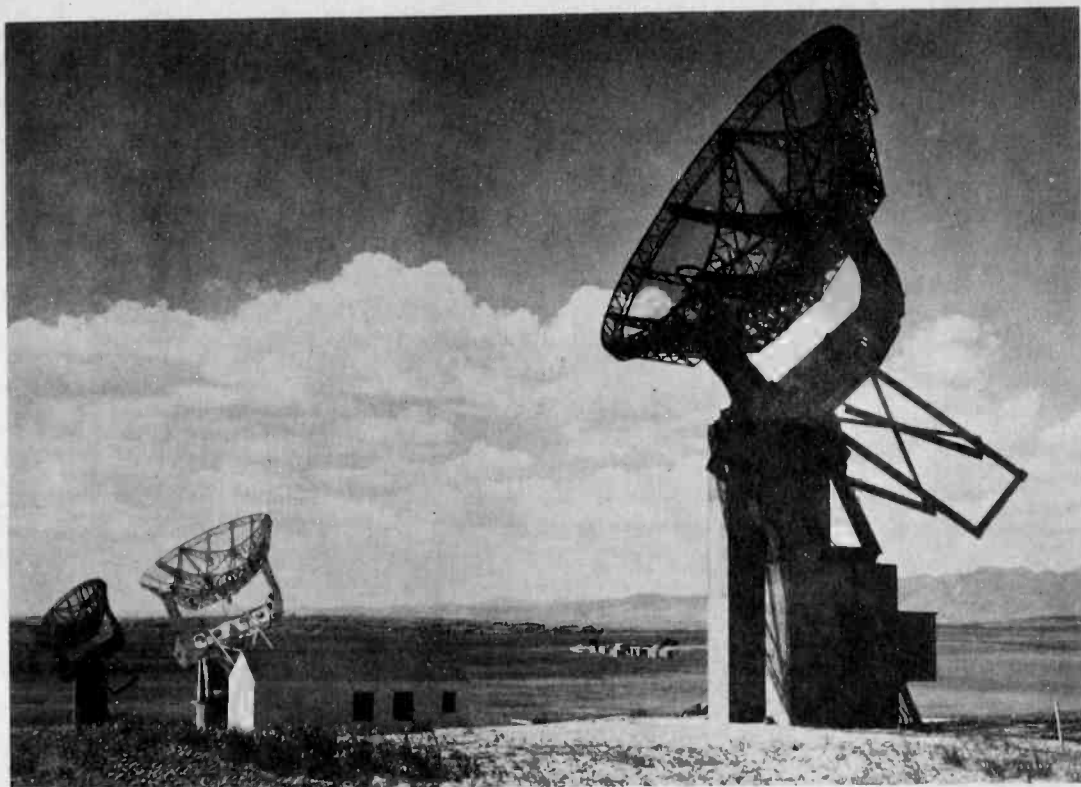
Figure 4. Gun Barrel Hill, Colorado, NBS Field Station Containing Three Giant Wurtzburg Antennas. These devices are arranged to receive signals of a certain frequency radiated from the sun and to track the sun automatically as it moves across the sky. Each antenna is tuned to receive a different frequency from the many emitted by the sun.
