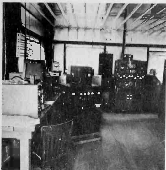
Figure 17. Interior of NBS Field Station Near Boulder, Colorado, Established to Monitor and Study the Signals Transmitted by Radio Station WWV and WWVH. The station is also used as one of the network of ionosphere probing stations maintained by, or operated in cooperation with, the National Bureau of Standards. The C3 ionosphere recorder (right, background) is one of the basic instruments used widely by science and the military for investigating the outer atmosphere by radar techniques.
