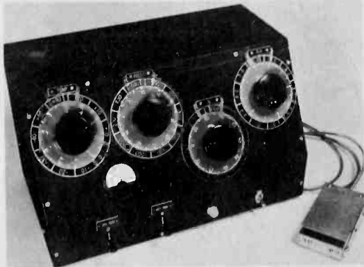
Figure 12. Analogue Computer for Solving the Radio Refractive Index Equation. This device is one of the products of the CRPL instrumentation program devoted to the development of equipment to be used in studies of the ionosphere and troposphere. This instrument computes the refractive index automatically from observed meteorological parameters, including temperature, atmospheric pressure, and relative humidity.
