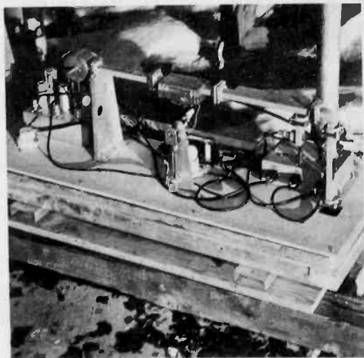
Figure 11. Microwave Components of NBS Microwave Refractometer Used by CRPL to Measure the Refractive Index of the Lower Atmosphere. In normal use, these components are suspended from the top of a 500-foot tower.
