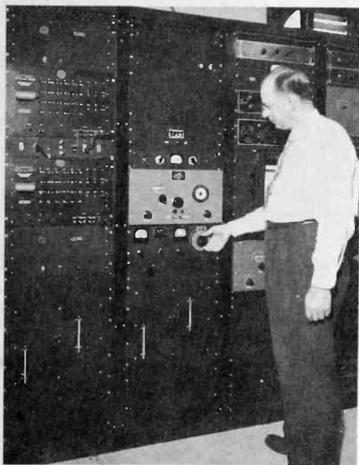
Figure 13. NBS Primary Resonator Frequency Standard. Temperature-controlled quartz crystals are made to resonate at a frequency of 100 kc. Several of the oscillators are offset from 100 kc. by a small number of cycles to permit comparison measurements by dual electronic counters. A variable oscillator is also employed in the comparison measurements. The accuracy of this system is more constant than the rotation of the earth, the present National standard of time. Therefore, deviation of the oscillator frequency (and, therefore, that transmitted by WWV) from the mean sidereal day must be computed. These variations are periodically issued as corrections to the NBS frequency standard utilized by science, industry, and commerce.
