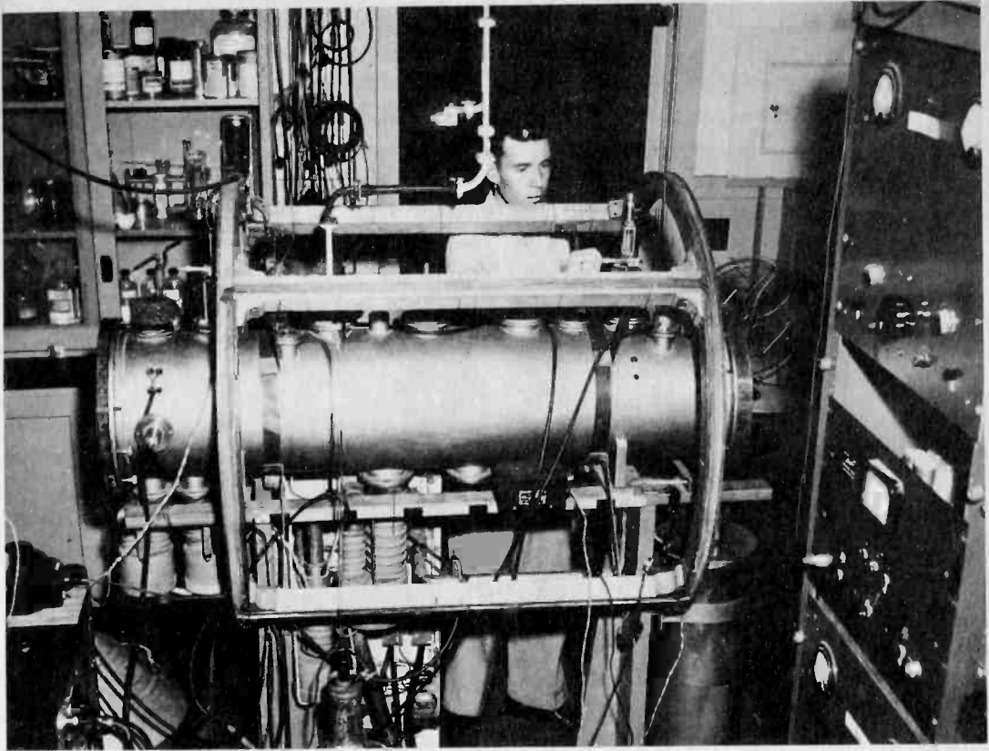
Figure 18. NBS Atomic Beam Clock. A beam of cesium atoms is discharged and made to move down the cylinder from left to right. When these atoms pass through the electromagnetic field set up by microwave energy, they vary from a straight-line path. Suitable instruments can be arranged to detect this variation and feed a voltage back into the microwave generator so as to make it correct itself, and, thereby, produce the correct frequency. With this system, accuracies can be obtained of better than one part in 10 billion.
