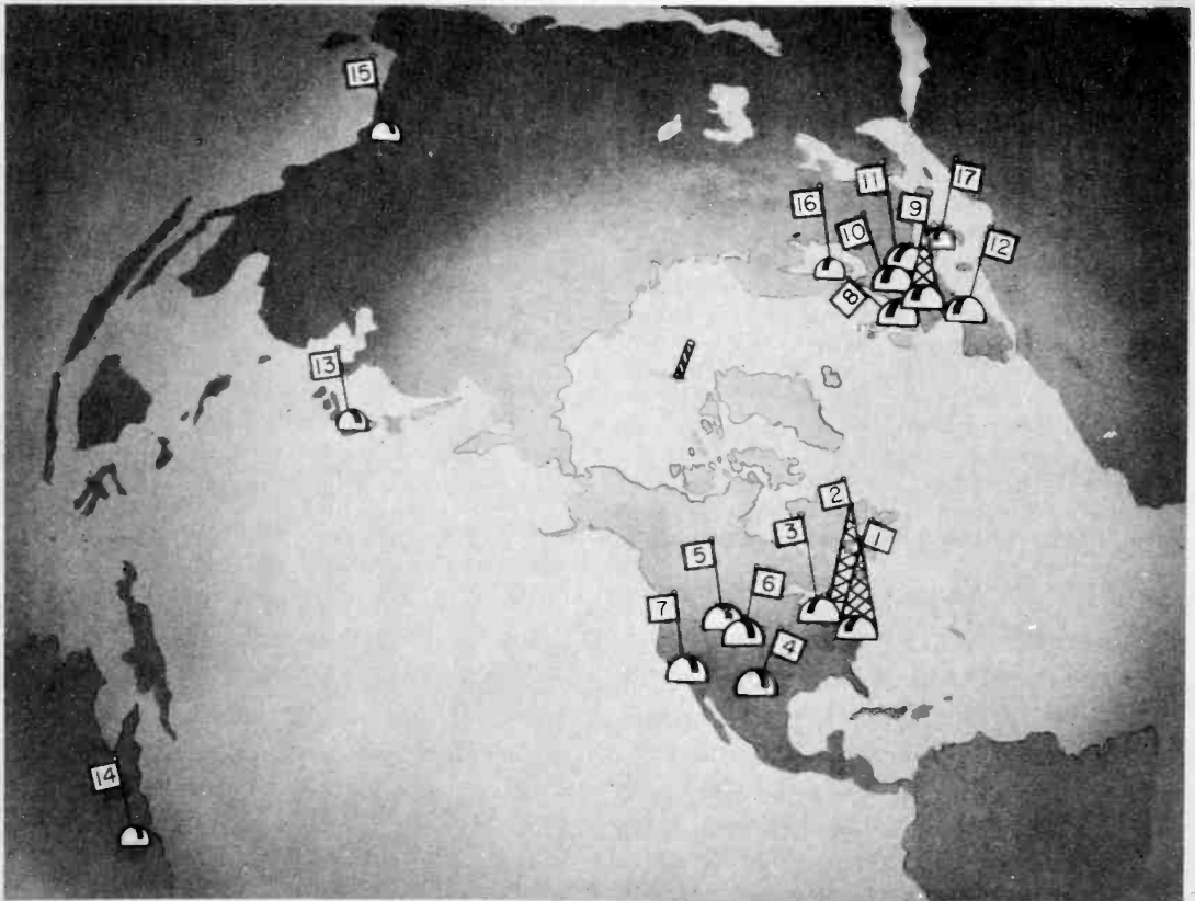
Figure 3. Network of World-Wide Observatories Supplying CRPL with Solar Activity Information. (Numbered flags designate location of each observatory.) 1: NBS and Naval Observatory, Washington, D.C.; 2: Cornell University, New York; 3: McMath-Hulbert Observatory, Michigan; 4: Sacramento Peak, New Mexico; 5: Climax, Colorado; 6: Boulder, Colorado; 7: Mt. Wilson, California; 8: Greenwich, England; 9: Meudon, France; 10: Wendelstein, Germany; 11: Kanzelhoehe, Austria; 12: Pic du Midi, Pyrenees; 13: Tokyo, Japan; 14: Mt. Stromlo, Australia; 15: India; 16: Sweden; 17: Italy.
