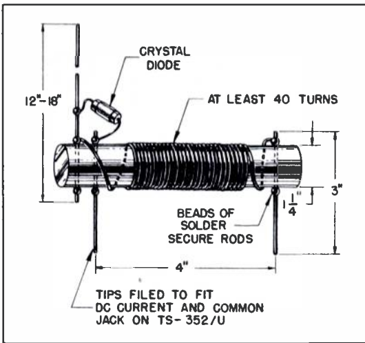
Figure 2. Sketch of Field Strength Attachment
