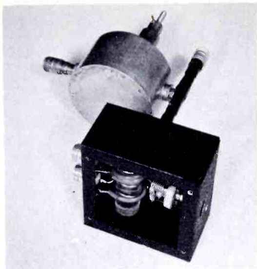
Figure 6. Crystal mixer for combining frequencies generated by the NBS microwave fixed-frequency standard. By means of resonant circuits in series, three standard signals—50, 250, and 3000 mc.—are applied simultaneously to the crystal converter. By extending these methods, additional frequencies may be added. The small box contains tuned circuits for the 50-mc. and 250-mc. signals. The cylinder is a cavity tuned to 3000 mc.
