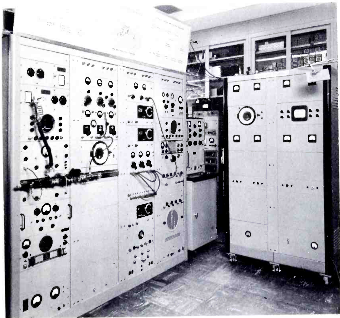
Figure 1. The microwave adjustable-frequency standard with which the National Bureau of Standards calibrates secondary frequency standards for Government agencies and defense activities, as well as science and industry. The four-rack system includes frequency multipliers, adjustable-frequency oscillators, and the necessary metering and monitoring equipment. The adjustable-frequency standard occupies the two center racks. Two transmission-type wavemeters are shown mounted for a calibration; the meter to the left has been sent to the Bureau to be calibrated against the standard. Variations in output with change in meter setting are monitored on the visual analyzer mounted in the first rack. The system of panel jacks permits the mixing of many standard frequencies. The pair of dolly-mounted racks to the right contain the electronic components of the Model II ammonia clock.
