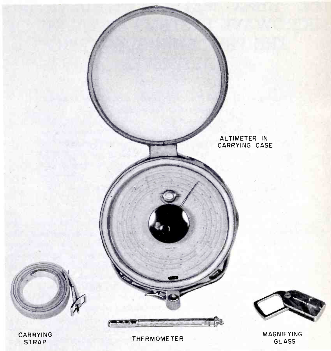
Figure 1. Precision Surveying Altimeter, with Accessories
