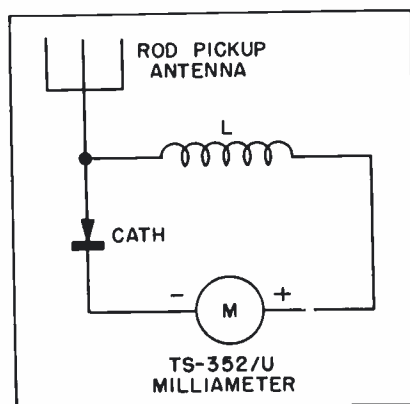
Figure 1. Schematic Diagram of Field Strength Meter
