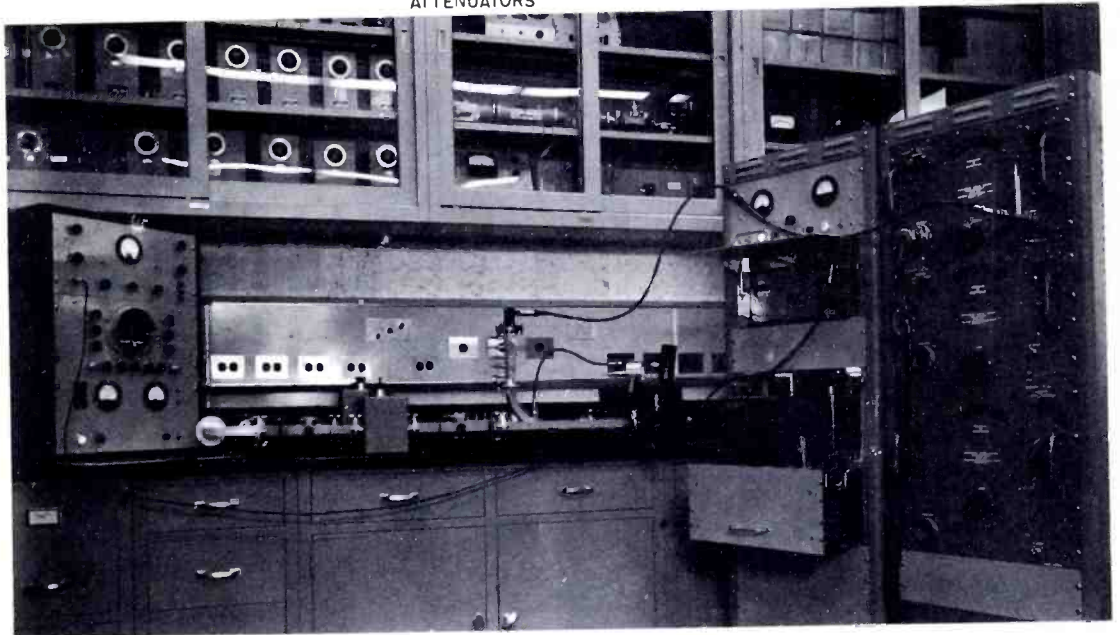
Figure 3. Calibrating a frequency meter with the NBS microwave fixed-frequency standard. The rack to the far right contains the local oscillator and associated power supplies; the rack to the left of the first contains the fixed standard. The r-f components on the bench include (in a clockwise direction): directional coupler, matching section, and coaxial-to-waveguide transformer; variable attenuator; the frequency meter to be calibrated (similar to those in the shelves above); another attenuator; buffer; tunable transmission filter; another buffer and matching section; crystal harmonic generator; connector for the standard; and mixer (black box and cylinder) for mixing the standard signals. The output of the system (an intermediate frequency) is fed to the spectrum analyzer at the far left. The accompanying block diagram shows the relative positions of the r-f components used in the calibration.
