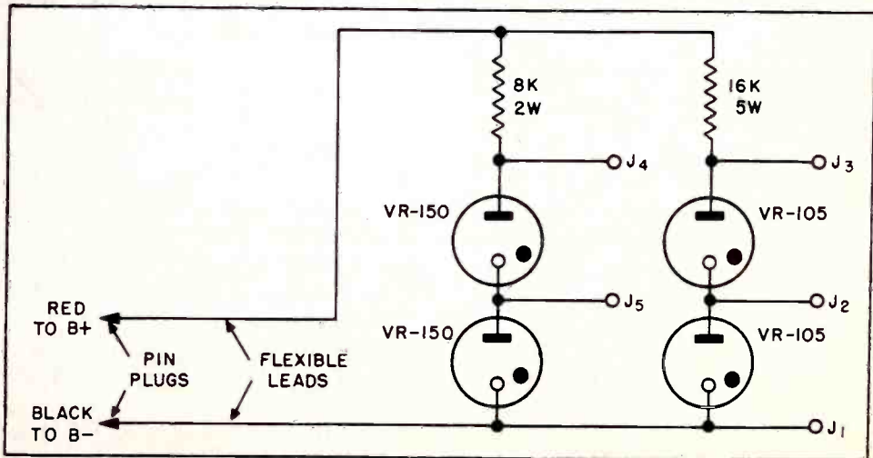
Figure 1. Schematic Diagram of Regulated Voltage Source
