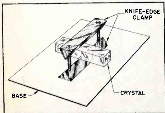
Figure 12. Knife-Edge Mount for Longitudinally Vibrating Crystal
