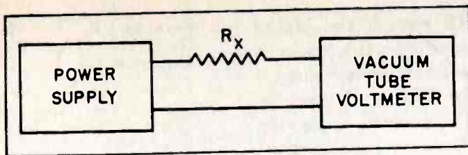
Figure 2. Block Diagram of Setup For Measuring Large Resistances
