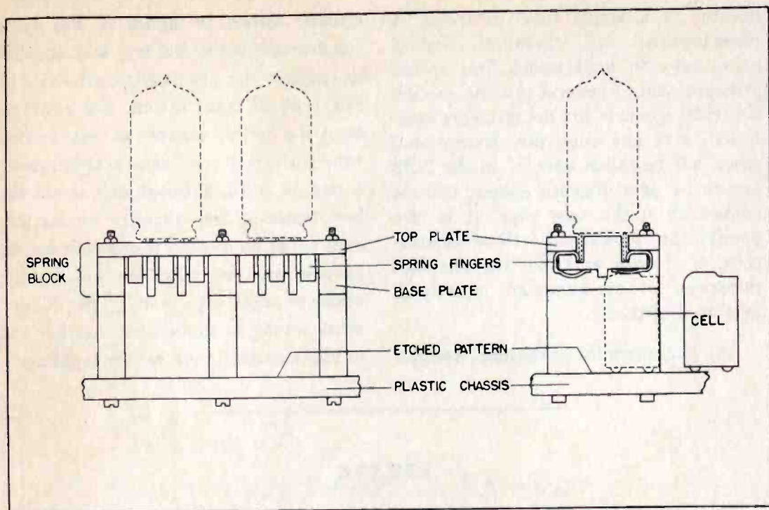
Figure 2. Drawing showing details of the NBS cellular assembly method.
