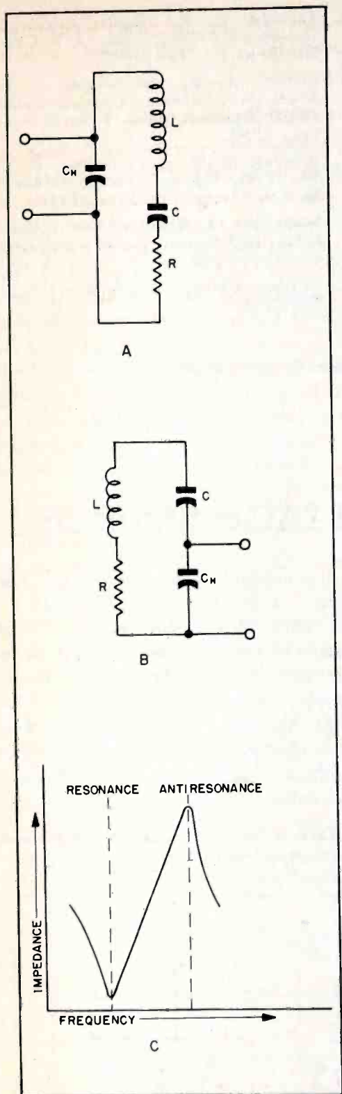
Figure 19. Equivalent Electrical Circuit of Quartz Resonator in a Holder
