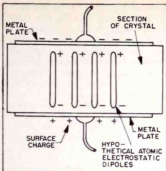
Figure 1. Cross-Section View of Piezoelectric Crystal, Showing Dipole Alignment (Dipoles Greatly Exaggerated)
