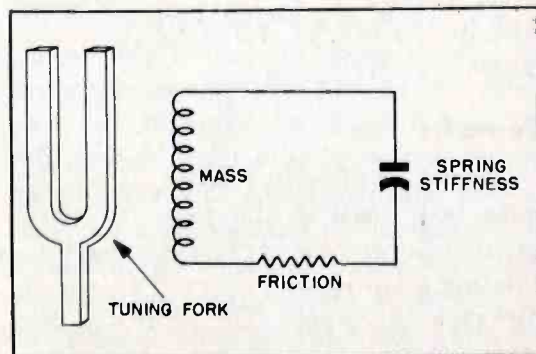
Figure 4. Tuning Fork and Electrical Equivalent
