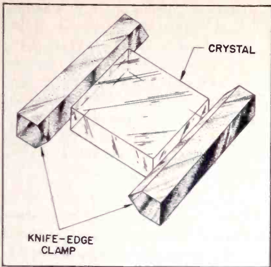
Figure 14. Knife-Edge Clamp for Supporting a Crystal Operating in Thickness Shear
