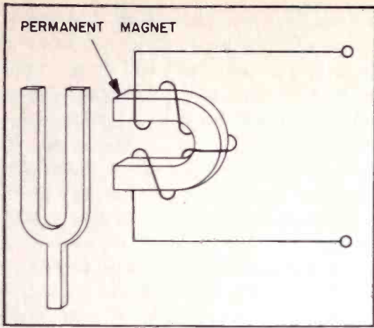
Figure 5. Tuning Fork with Electric Drive
