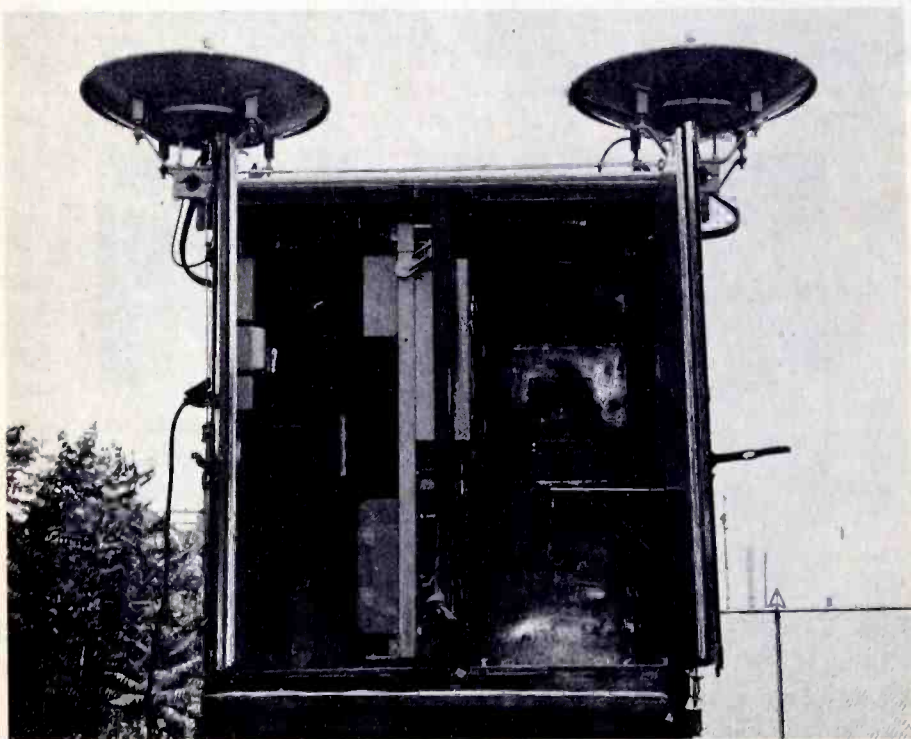
Figure 3. Rear View of Truck, Showing Microwave Dishes Mounted in Operating Position
