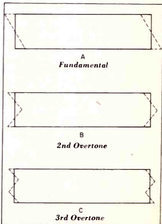
Figure 10. Overtone Shear Vibration (Cross-Section View of Crystal)
