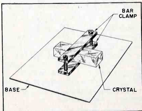
Figure 13. Bar Mount for Longitudinally Vibrating Crystal
