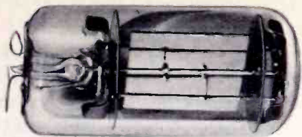
Figure 17. Vacuum-Mounted Quartz Resonator Used by the National Bureau of Standards as a Frequency Standard
