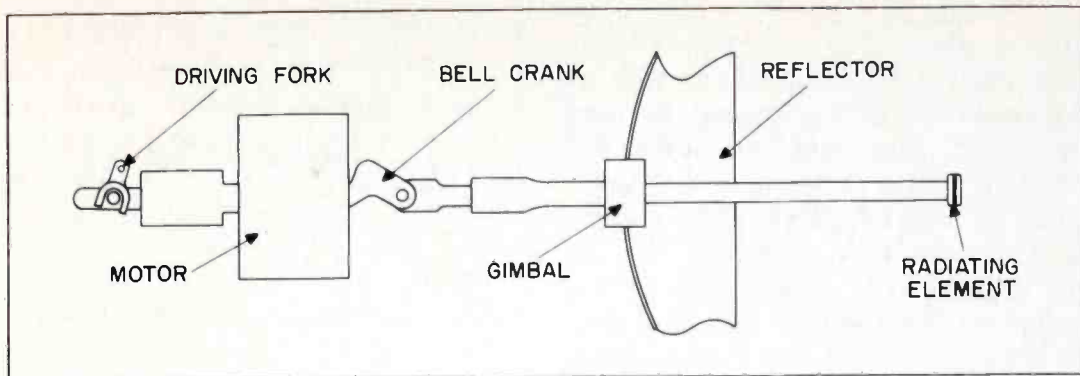
Figure 17. Nutating-Scan Feed for SCR-584
