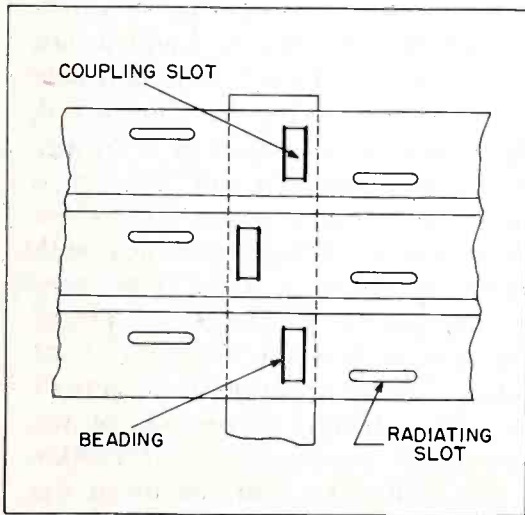
Figure 32. Feeder for Short-Range Array of MK-6 Antenna
