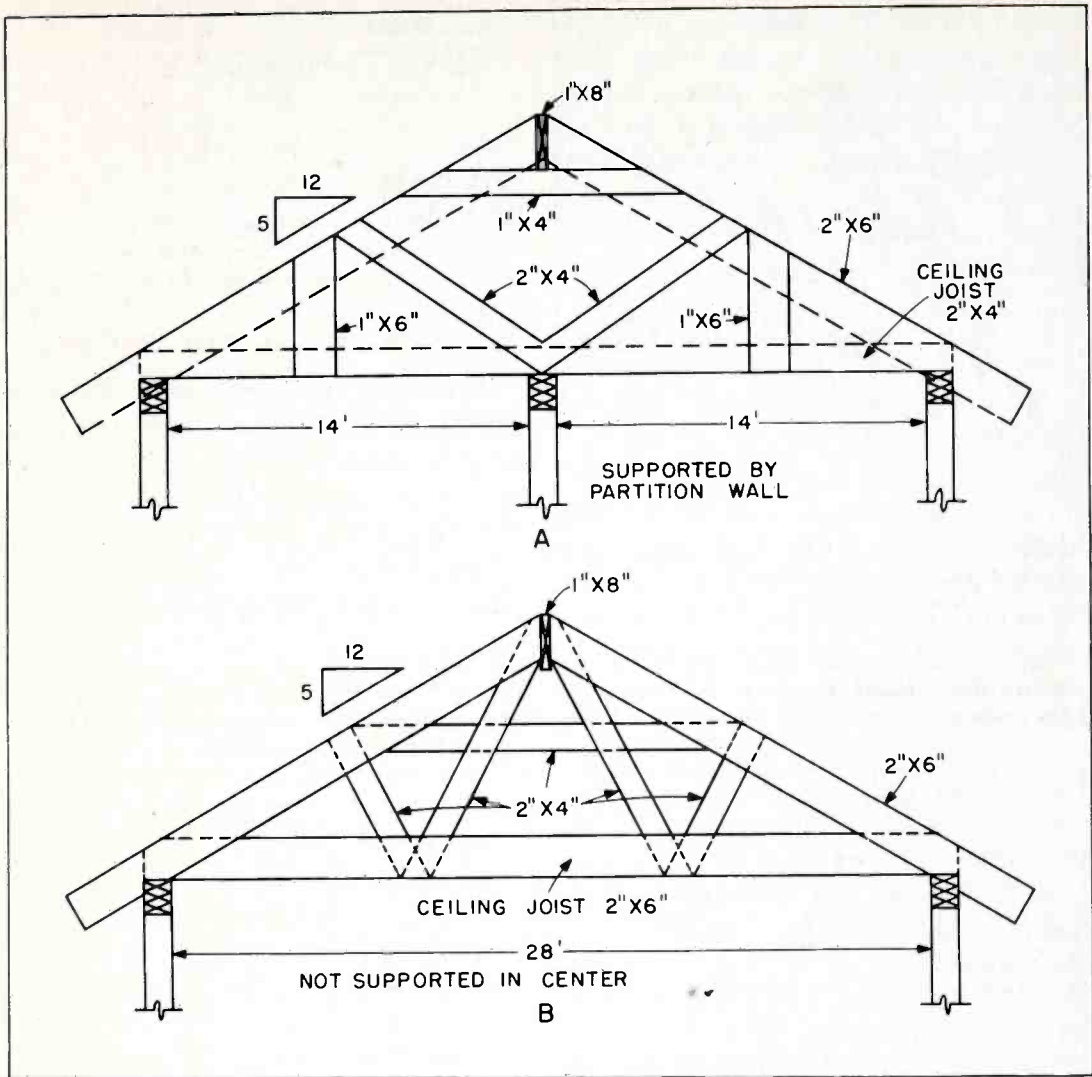
Figure 10. Typical Roof Trusses (A—Supported, B—Non-Supported)
