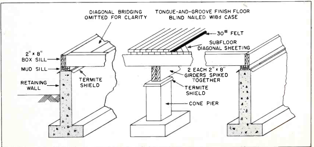
Figure 4. Foundation for Wood Floor
