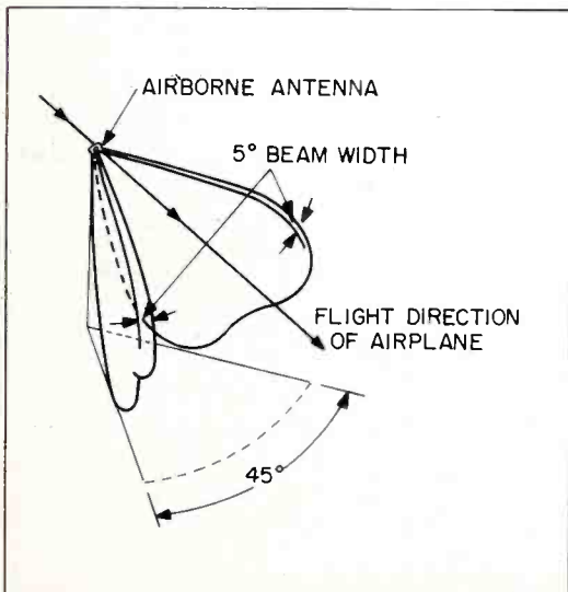
Figure 16. Sector Scan of AN/APQ-13
