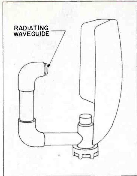
Figure 5. SL Radar Antenna
