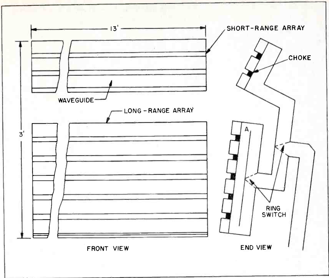
Figure 29. Front and Side Views of MK-6 Antenna
