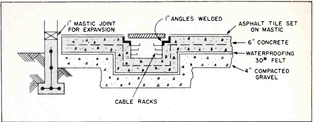
Figure 2. Cross-Sectional View of Typical Concrete Floor
