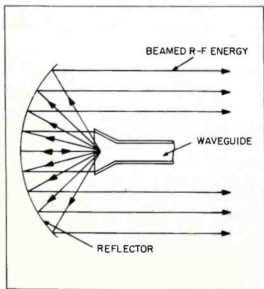
Figure 18. Open-End Waveguide Feeding into a Reflector
