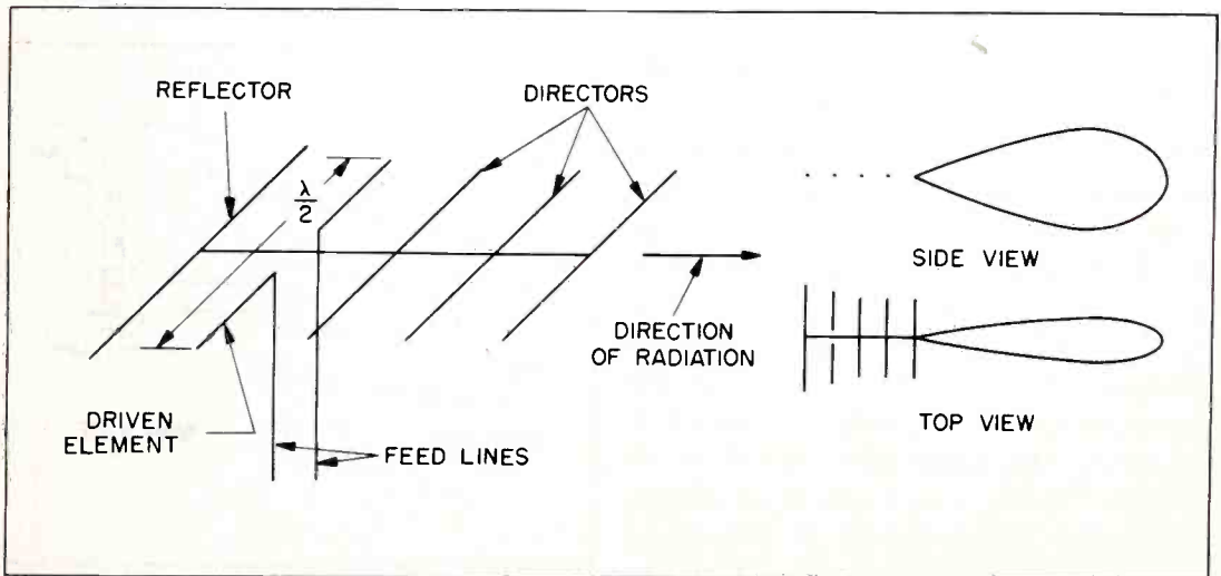
Figure 25. Yagi Antenna and Radiation Pattern
