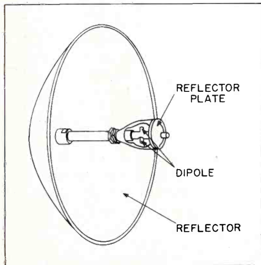
Figure 3. SCR-584 Antenna
