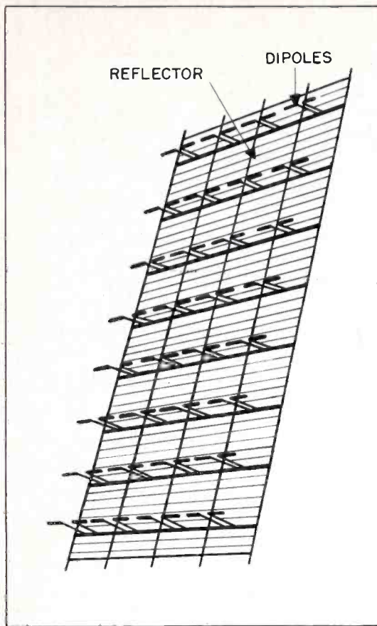
Figure 2. SCR-270 Bedspring Antenna
