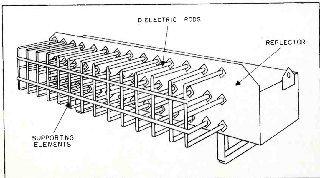
Figure 23. Array of End-Fire Polyrod Radiators
