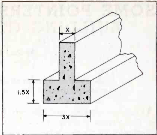
Figure 1. Aspect Ratio of Concrete Foundation
