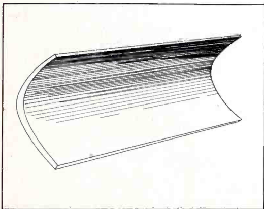
Figure 8. Parabolic-Cylinder Reflector
