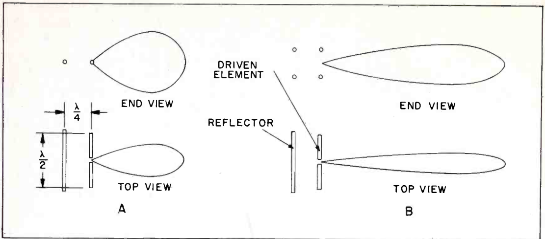
Figure 11. Radiation Pattern of Dipoles and Reflectors
