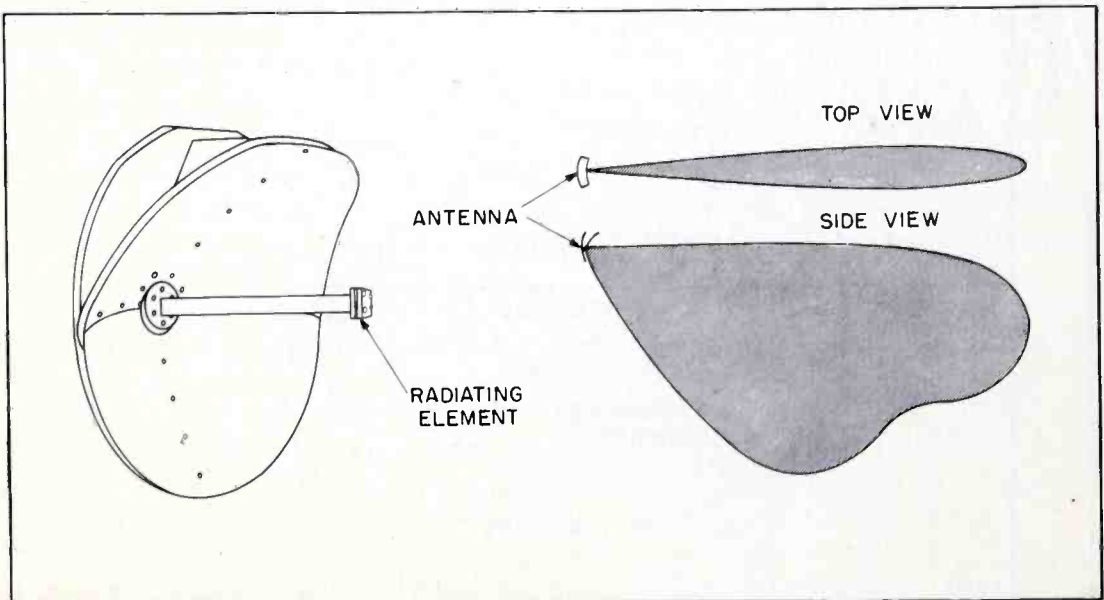
Figure 10. Cosecant-Squared Antenna and its Radiation Pattern
