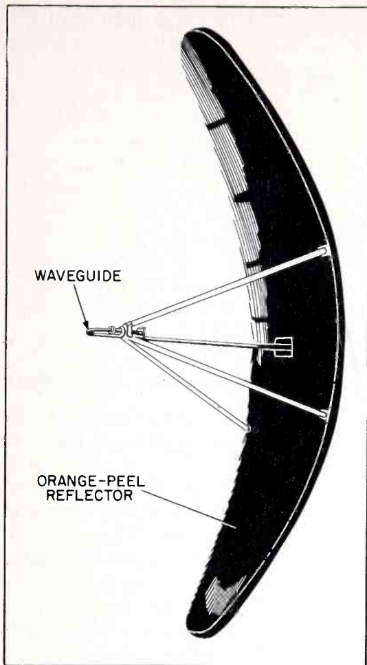
Figure 7. AN/TPS-10 Antenna
