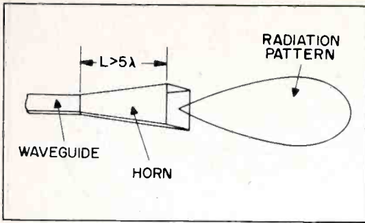
Figure 24. Horn Antenna
