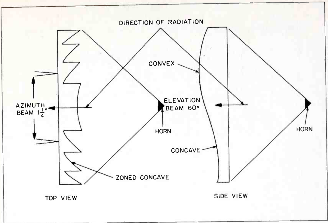
Figure 34. T33 Lens Antenna
