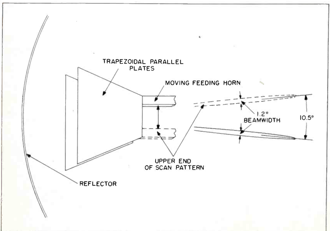
Figure 21. Robinson Electrical Feed for SCI Height-Finder Antenna
