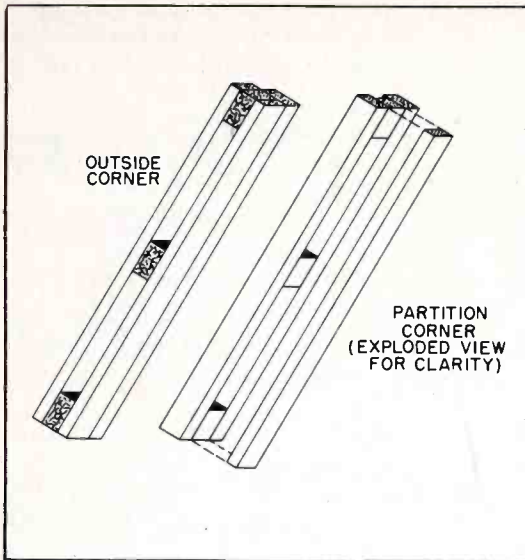
Figure 7. Construction of Standard-Type Corners
