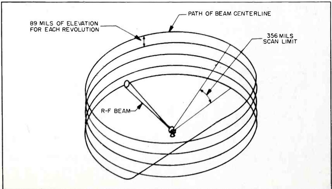
Figure 14. SCR-584 Helical Scanning
