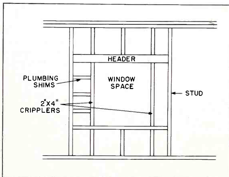
Figure 9. Construction of Wall Framing around Windows
