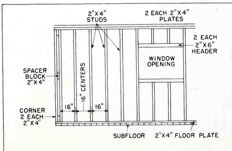
Figure 6. Typical Wall Framing
