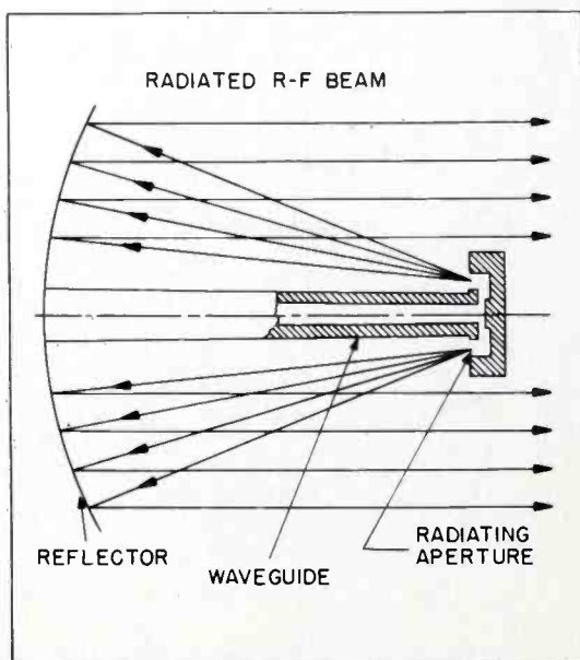
Figure 19. Cutler Feed
