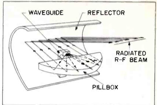
Figure 20. Pillbox Feed to a Cylindrical Reflector
