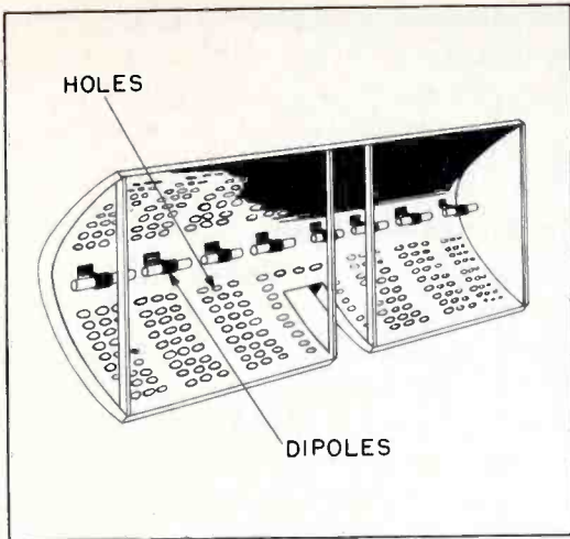
Figure 9. Parabolic-Cylinder Antenna
