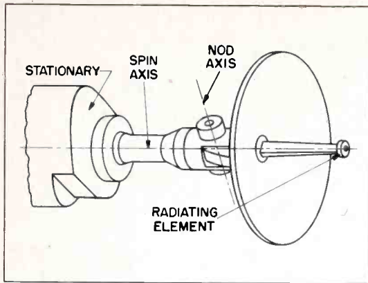
Figure 15. AN/APS-6 Antenna System
