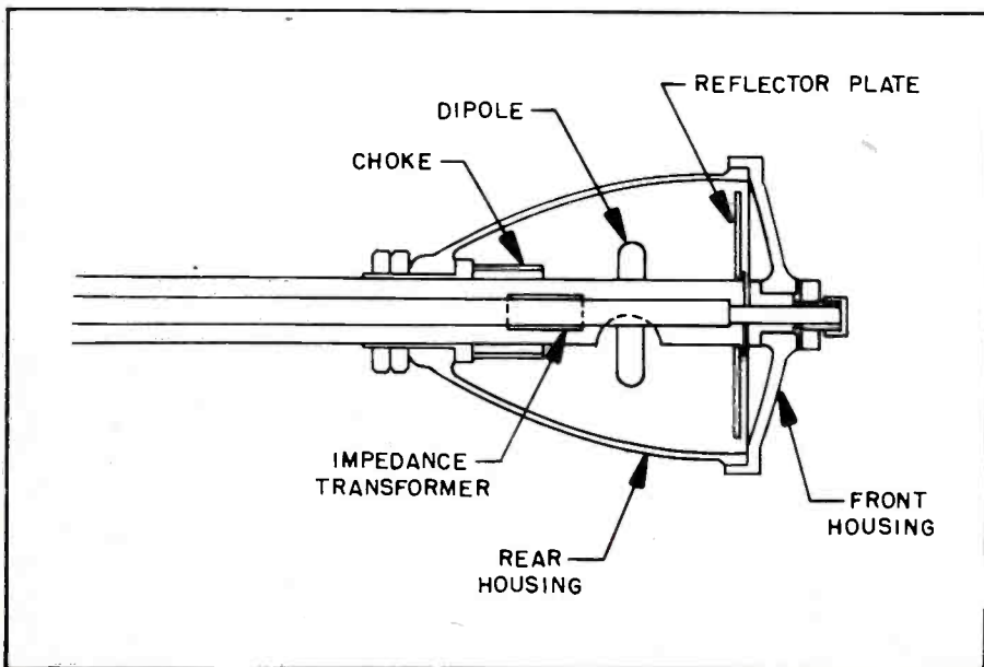
Figure 12. SCR-584 Dipole Assembly
