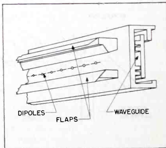
Figure 27. Dipole and Waveguide of AN/APQ-7 Eagle Scanner
