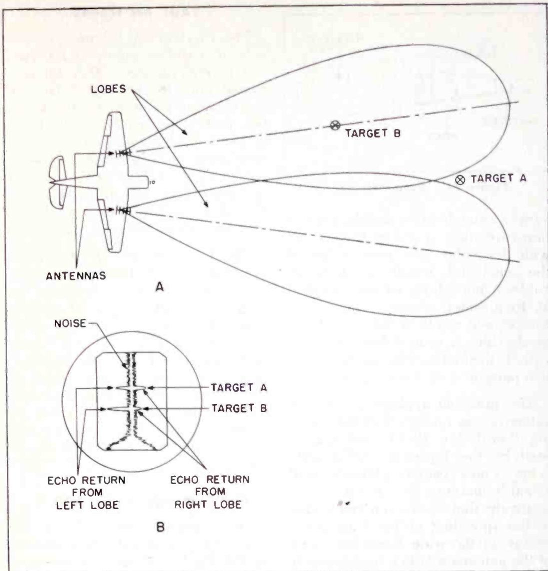
Figure 26. Yagi Antennas Used for Lobing
