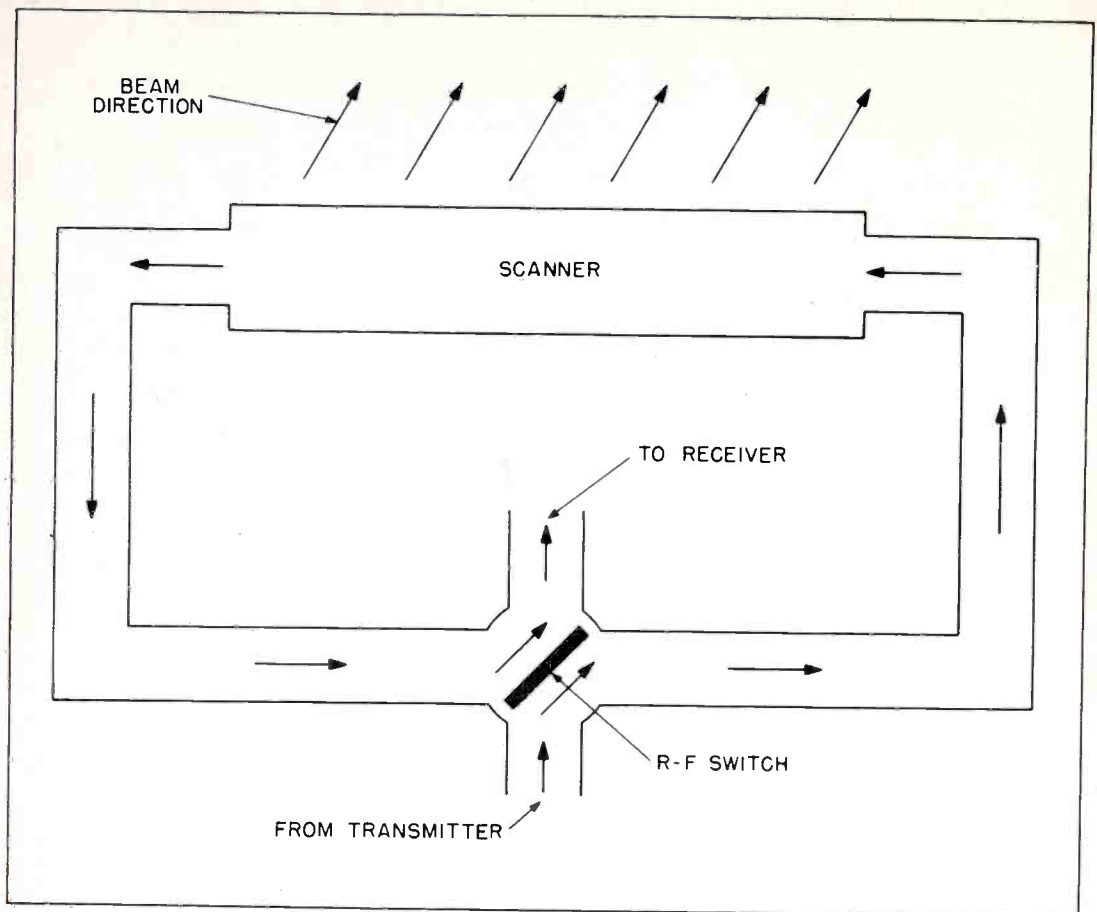
Figure 28. Energy Flow in Waveguide of Eagle Scanner
