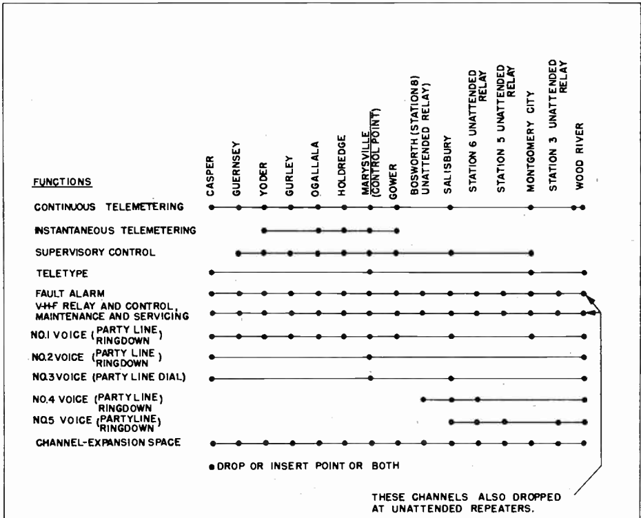
Figure 3. Channelizing Diagram
