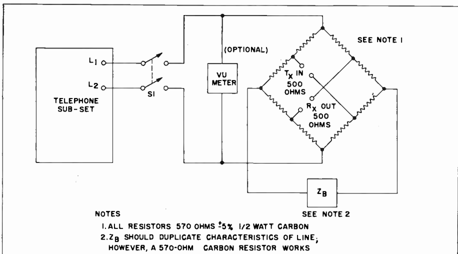
Phone-Patch Circuit
