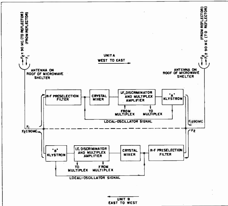
Figure 4. CLR-6 Functional Block Diagram
