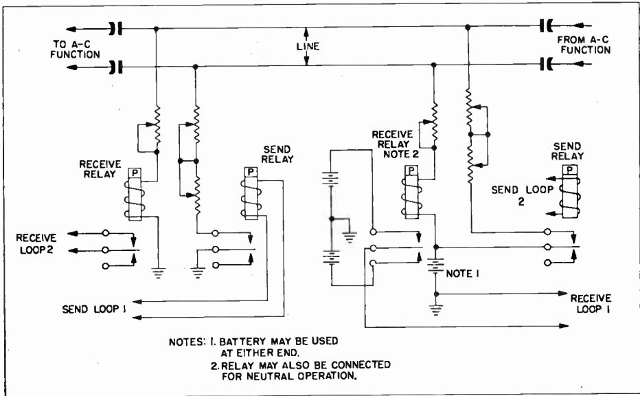
Figure 9. Compositing an A-C Metallic Circuit To Provide Two Additional D-C Teletype Circuits
