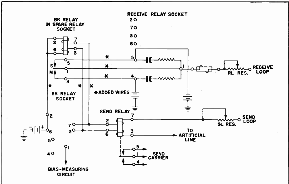
Figure 1. Simplified Schematic, Showing Modification
