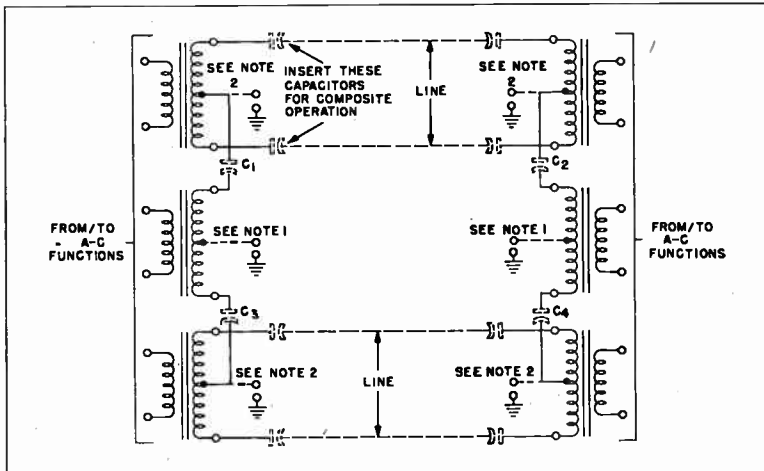
Figure 10. Method of Phantoming a Circuit, with Provisions for Simplex or Composite Operation
