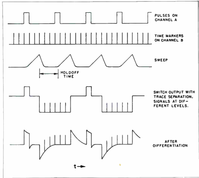
Figure 2. The effect of differentiator circuit on a sync waveform.
