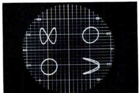
Figure 16. Set up and display when electronic switches are used to compare four signals on one cathode-ray screen.
