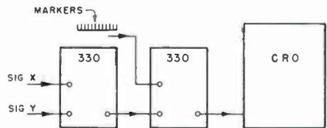
Figure 6. Arrangement used to minimize phase shift effect between signals X and Y (see text).
