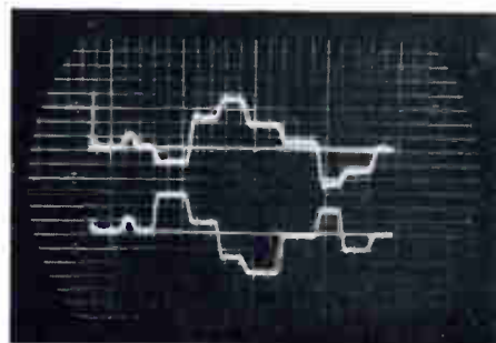
Figure 18. Color T-V I and Q signals displayed simultaneously through use of electronic switch.
