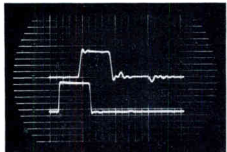
Figure 12. Set up and resulting display when the electronic switch is used to align delay lines.
