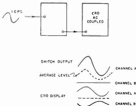
Figure 10. Drawing showing the effects of an a-c coupled oscillograph on low frequency phenomena.
