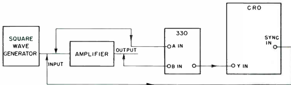
Figure 1. Typical connection for synchronization of related signals.
