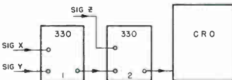
Figure 5. Arrangement used to get three channel display.
