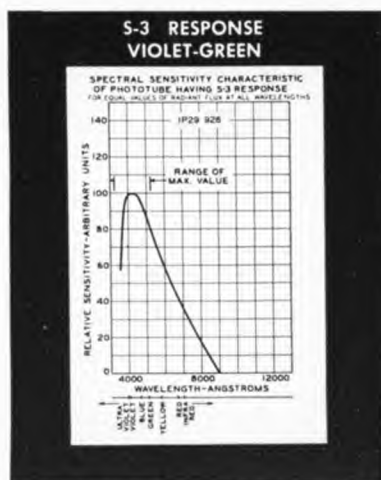
Figure 32. Spectral response of typical phototube. (Courtesy of the Radio Corporation of America)
