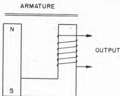
Figure 27. Generator type of variable reluctance element
