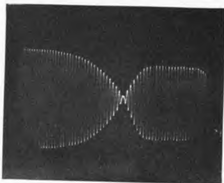
Figure 31. Envelope obtained from differential transformer. Null is not in center of displacement
