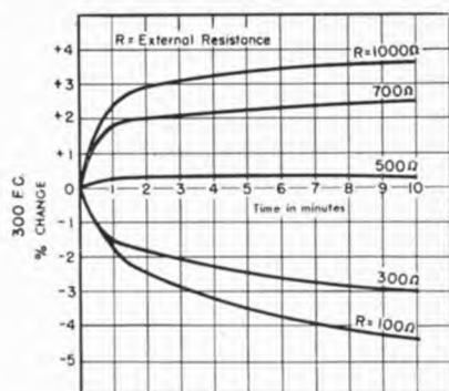
Figure 41. Temporary fatigue curves of barrier layer photocell showing percentage change in current output and external cell resistance. (Courtesy of General Electric Company)
