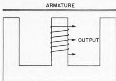
Figure 28. Variable inductance reluctance element
