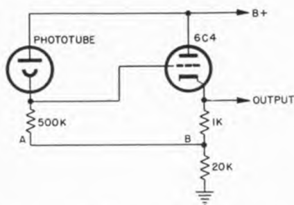
Figure 35. Vacuum phototube with cathode-follower amplifier for small signal variation and with a frequency response from d-c to reasonably high frequencies
