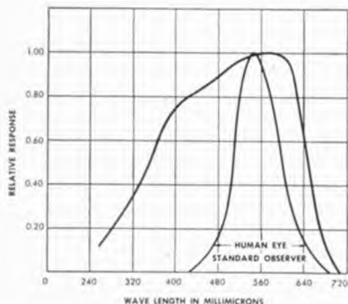
Figure 40. Spectral response of typical photocell (Courtesy of Vickers, Inc.)
