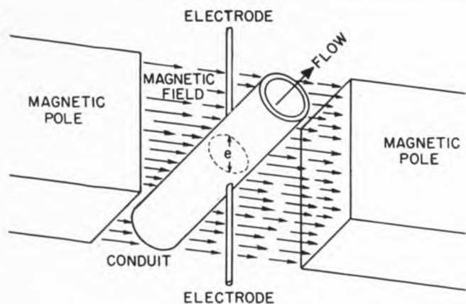
Figure 26. Steady-field transducer for fluid flow through tube
