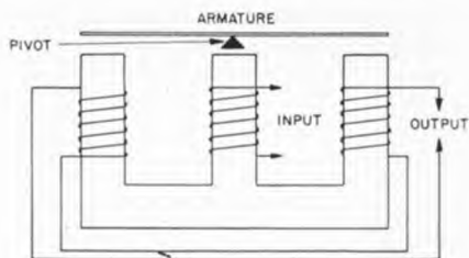
Figure 29. Balanced coil arrangement
