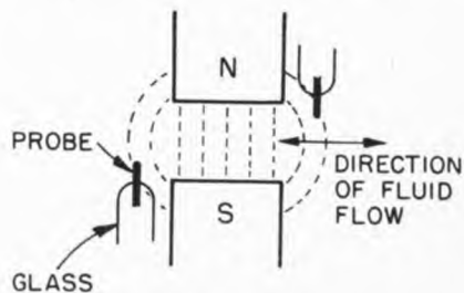
Figure 25. Steady-field transducer for total submergence
