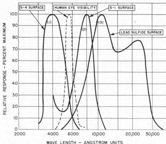
Figure 38. Spectral response of three lead sulfide cells and human eye. (Courtesy of the Continental Electric Company)
