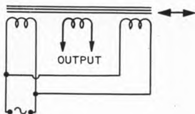
Figure 30. Differential transformer
