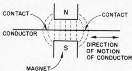
Figure 24. Steady-field transducer
