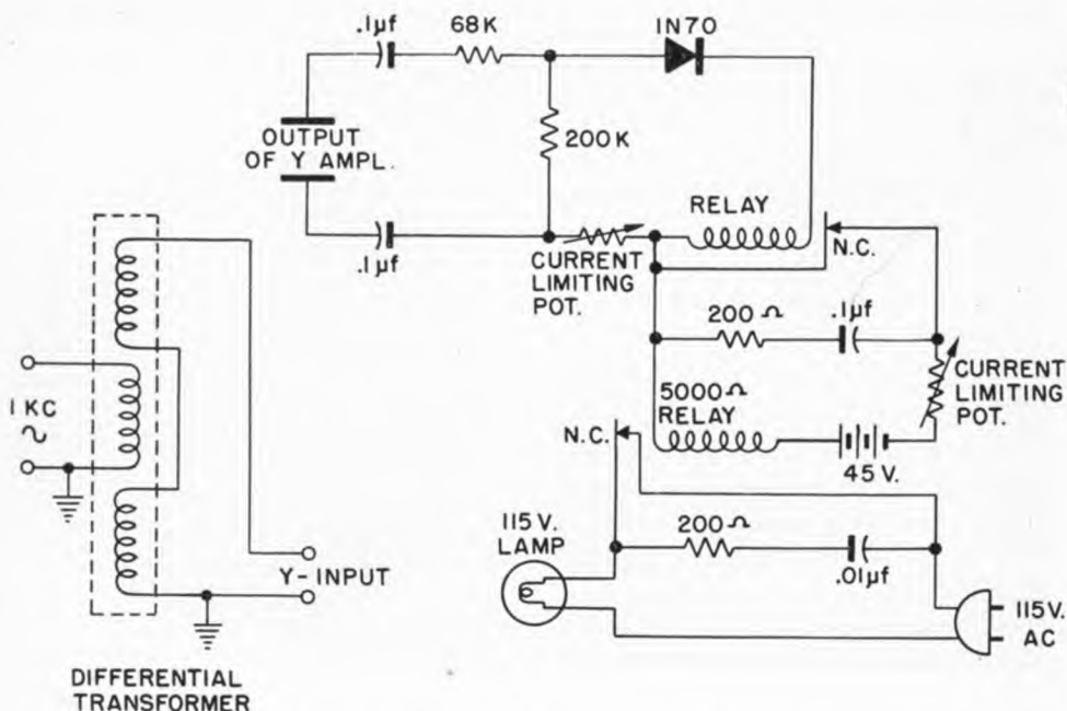
Figure 1. Schematic diagram of the automatic hardness tester
