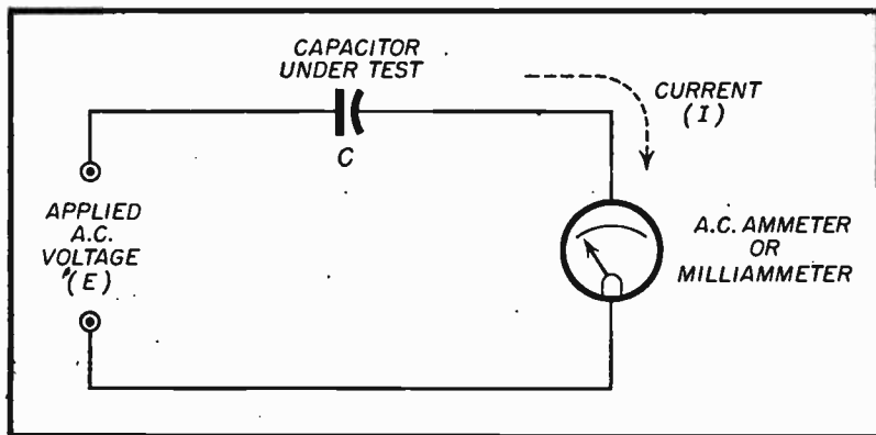
Fig. 1. Simple Reactance-Type Capacitance Meter.
