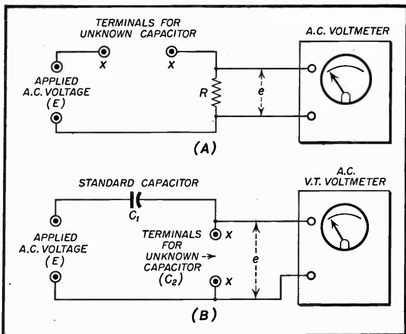
Fig. 2. Use of Voltmeter to Check Capacitance.
