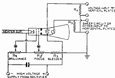
Fig. 9. Typical cathode-ray tube circuit.
