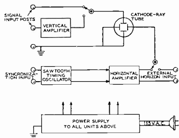
Fig. 3. Block diagram of a typical cathode-ray oscilloscope.
