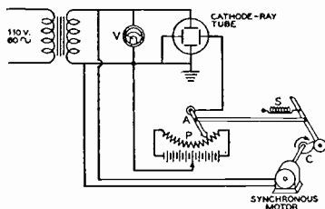
Fig. 11. Mechanical sweep circuit.
