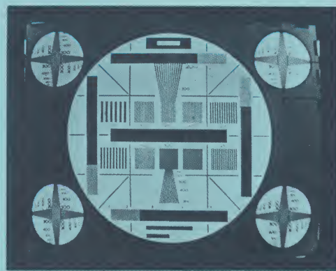
FIGURE 1. Typical test pattern used to measure resolution.
