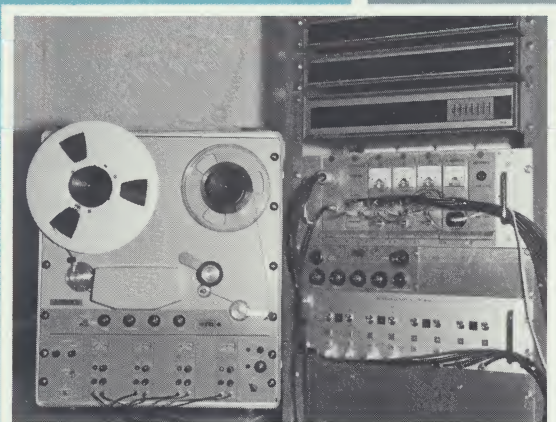
Ampex SP-300 four-track instrumentation recorder records and plays back digital data in Swiss air pollution studies.
