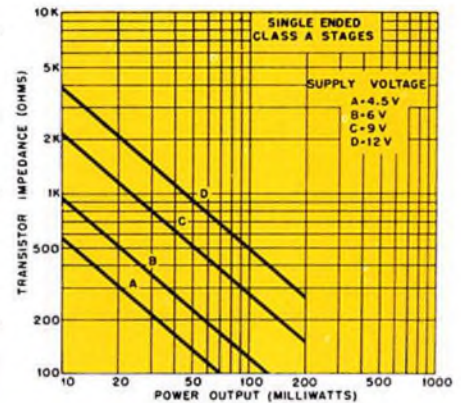
Transistor Impedance Characteristic Curves
