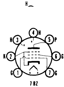
SYLVANIA TYPE 5AQ5 BEAM POWER AMPLIFIER
