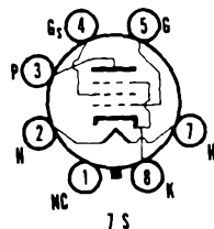
SYLVANIA TYPE 35L6GT BEAM POWER AMPLIFIER
