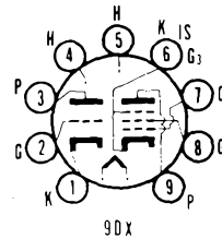
SYLVANIA TYPE 6AV8 TRIODE PENTODE
