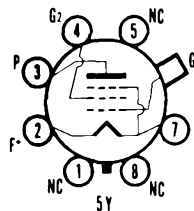
SYLVANIA TYPE 1N5GT SHARP CUTOFF R F PENTODE
