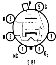
SYLVANIA TYPE 6CD6G BEAM POWER AMPLIFIER
