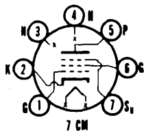
SYLVANIA TYPE 6BZ6 SEMI-REMOTE CUTOFF PENTODE
