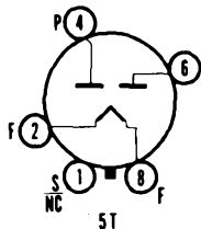
SYLVANIA TYPE 5Y3G 5Y3GT
