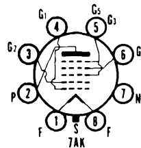
SYLVANIA TYPE 1LA6 HEPTODE CONVERTER
