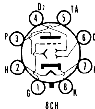
SYLVANIA TYPE 6AL7GT TUNING INDICATOR
