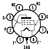
SYLVANIA TYPE 1LB4 PENTODE POWER AMPLIFIER
