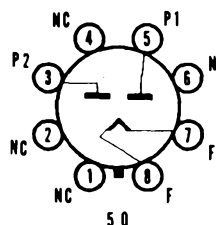
SYLVANIA TYPE 5Y4G FULL-WAVE RECTIFIER
