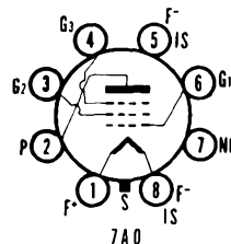
SYLVANIA TYPE 1LN5 SHARP CUTOFF R F PENTODE
