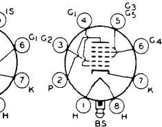
7B8 7B8-LM
