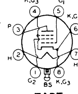
7AB7
