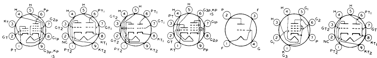
10C8
