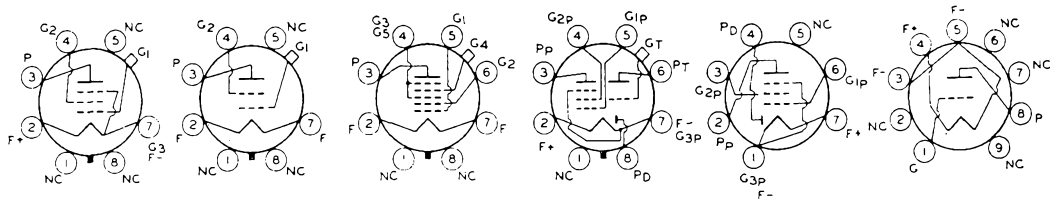
1D5-GP 1D5-GT 1D7-G 1D8-GT 1DN5 1E3
