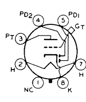
6V7-G
