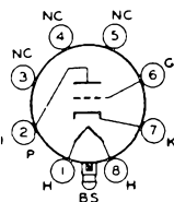
7B4
