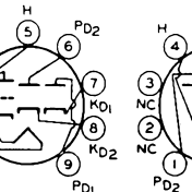
6BV8
