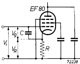
Fig. 5 Basic circuit for the compensation of input capacitance variation.
