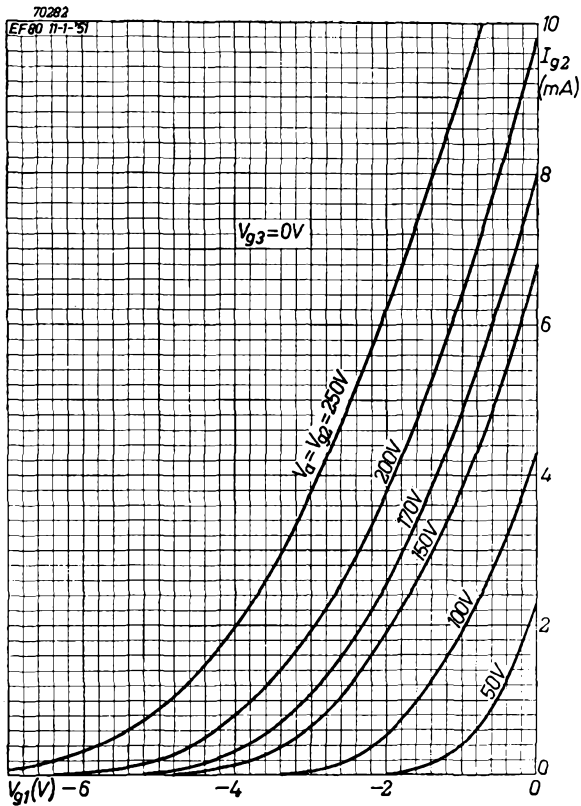
Fig. 11 Screen-grid current plotted against control-grid voltage for anode and screen-grid voltages between 50 V and 250 V.
