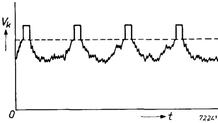
Fig. 2 Polarity of the signal required at the cathode of the picture tube.
