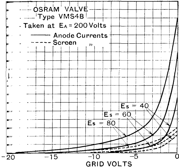
CHARACTERISTIC CURVES AVERAGE VALVES.
