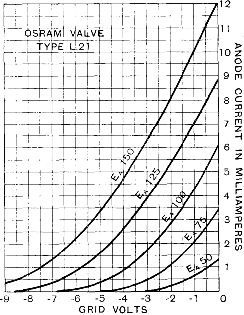
CHARACTERISTIC CURVES OF AVERAGE VALVES.
