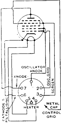
HEPTODES
