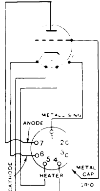
TRIODES WITH GRID TOP CAP.
