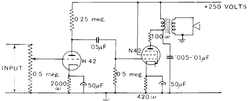
TYPICAL RESISTANCE COUPLED AMPLIFIER
