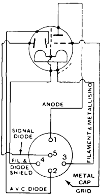
BATTERY DOUBLE DIODE-TRIODE
