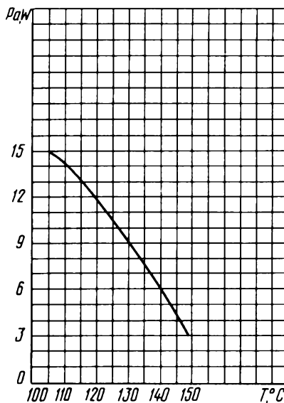
Characteristic Curves Showing Anode Dissipation P a max versus Ambient Temperature (at bulb temperature T a 200 °C)
