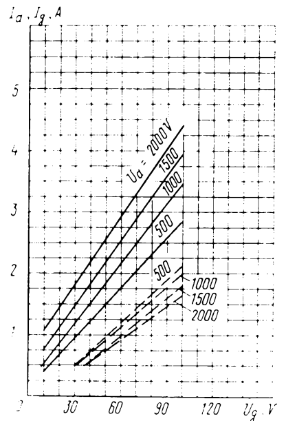
Averaged Characteristic Curves in Pulsed Operation: U_i = 12,6 \text{ В} ; \tau = 2 \text{ мкс} ; pulse frequency 500 Hz
