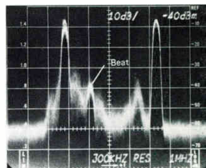
Figure 36. Beats within the Channel
