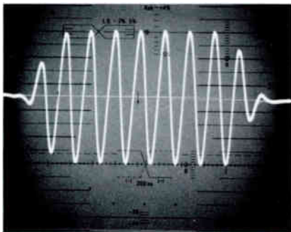
7. FCC standards require a minimum of 8 cycles of color burst. The burst shown here contains 8½ cycles.
