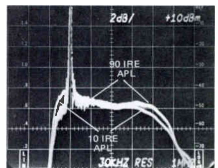
Figure 18. Transmitter Differential Gain Display for 20% Amplitude 0 and 100 IRE Test Sweeps
