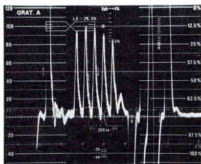
4. Off-air signal showing luminance nonlinear distortion. The tallest spike is set to 100 units, and the shortest spike pictured is down 14 units from 100.
