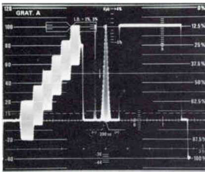
1. The modulated staircase is used to evaluate differential phase. As generated, the chrominance on the staircase is equal in phase and amplitude.
