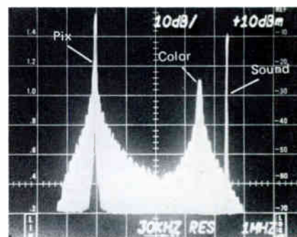
Figure 10. Typical TV Channel with Picture and Color Carriers
