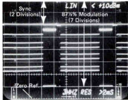
Figure 25. Modulation Adjustments Using the Spectrum Analyzer
