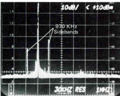
Figure 39. Beats Noted on Carrier Due to Local Broadcast Station
