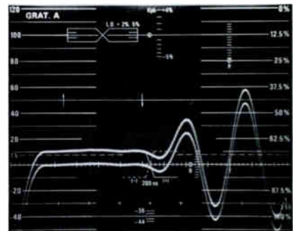
8. Double exposure showing breezeway measurement. Starting point at 1/10 of sync. Shown here, at 0.1 µsec/div, breezeway = 0.620 microseconds.
