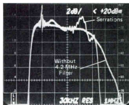
Figure 7. Response with and without 4.2 MHz Filter (Note Serrations Due to Filter)
