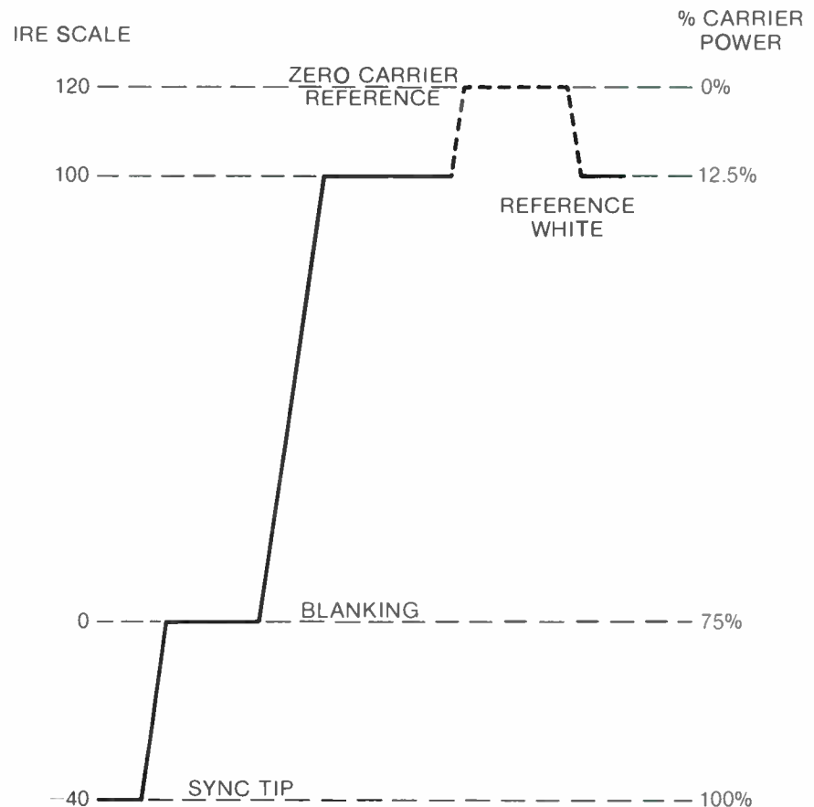
Relative levels of sync, picture and zero carrier.
