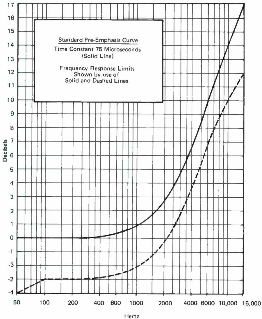
Figure 27. Standard 75 \mu s Pre-Emphasis on the Spectrum Analyzer
