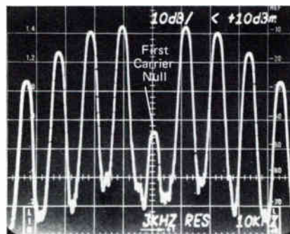
Figure 31. Bessel Null Technique of Determining 100% Modulation
