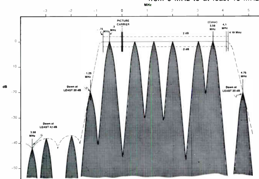
Figure 2. Idealized Color Transmitter Response (NTSC-Multi-burst Superimposed)
