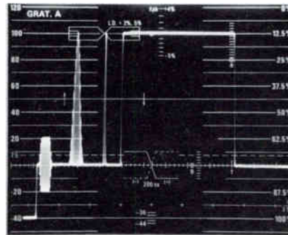
1. Modulated 12.5 T pulse used to measure chrominance to luminance gain and delay, here shown as part of a composite test signal.
