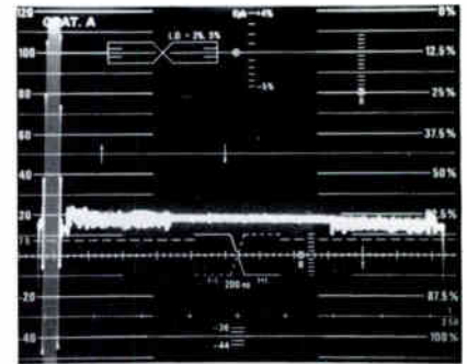
2. Vertical gain expanded, inserted pedestal adjusted to same level as video signal being measured.
