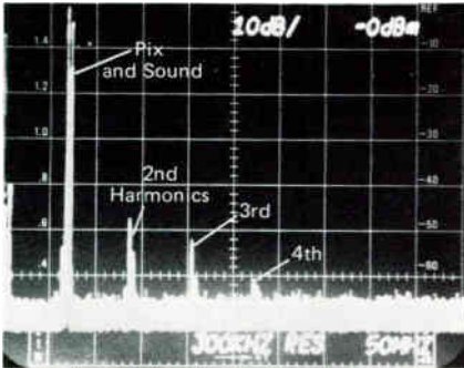
Figure 38. Harmonics of TV Transmitter
