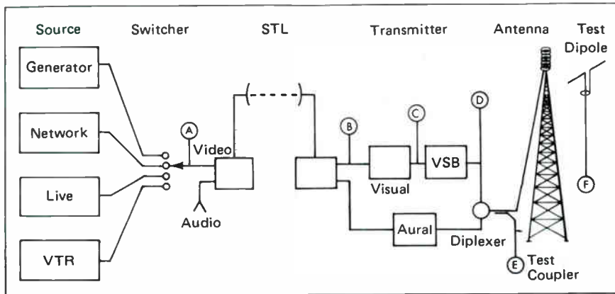
Figure 1. Typical Station Layout Showing Test Points
