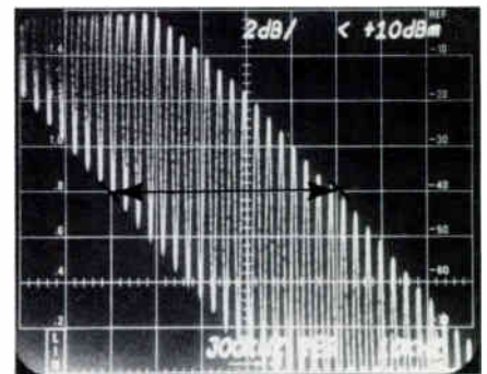
Figure 26. Measuring FM Deviation on the Spectrum Analyzer (5 divisions equals 50 kHz.)
