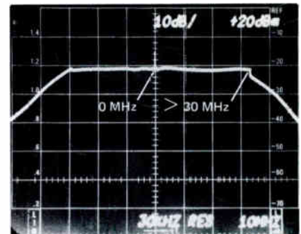
Figure 3. Sideband Analyzer Response at Baseband
