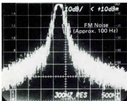
Figure 30. FM Noise on Aural Transmitter
