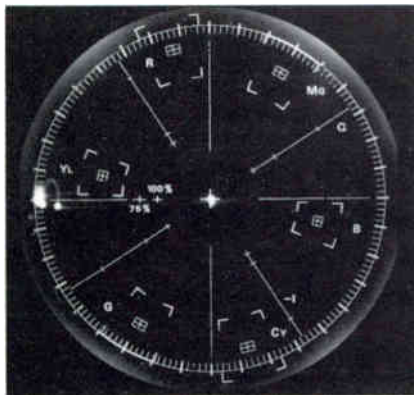
2. Viewed on a vectorscope in the VECTOR mode, the staircase chrominance component is positioned to the 0°-180° axis, and the gain is adjusted to place the staircase chroma at the perimeter of the circle.
