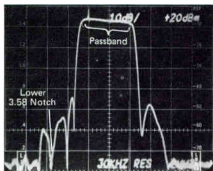
Figure 4. Transmitter Response at 2 MHz/Div and 10 dB/Div
