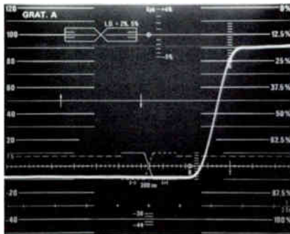
9. Shown here at 0.1 \mu sec/division. Sync pulse leading edge, 0.120 \mu sec, (Figure 9) sync pulse trailing edge 0.125 \mu sec.
