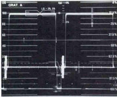
1. Sync should be 40/140 of the composite video signal.
