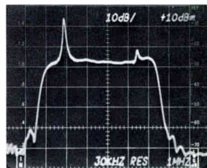
Figure 11. In-Service Low Level Sideband Response
