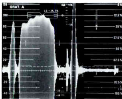
3. Signal expanded so that largest burst packet is 100 IRE peak. The amplitude difference between 100 and the smallest step is the amount of differential gain. Shown here, DG = 21%.
