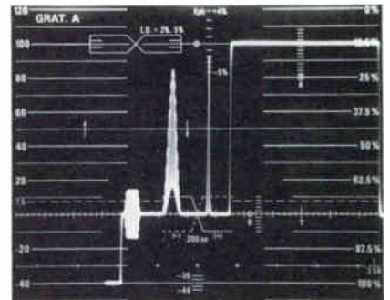
2. Pulse height is down about 8 IRE units. This corresponds to a K factor picture impairment of -2% ( K_{PB} ).
