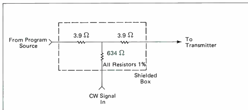
Figure 9. Insertion "T" for In-Service Low Level Testing
