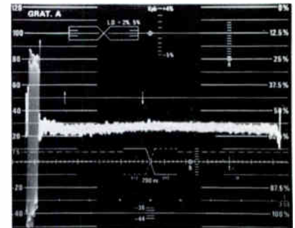
3. Adjustment of noise generator to match noise on signal. When the two signals cannot be differentiated visually, the dials of the noise generator are read to determine relative signal to noise ratio. In this case, SNR = -52 dB.
