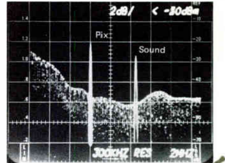
Figure 41. Return Loss (Match) of a TV Antenna
