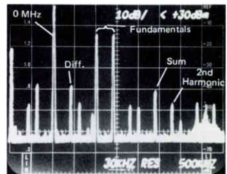
Figure 23. Distortion Measurements on the Spectrum Analyzer
