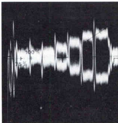
4. For greater accuracy in differential phase measurement, the double trace technique can be used. In this mode, the signal is set up as before, and the CALIBRATED PHASE shifter is set to 0. The CHANNEL A or CHANNEL B PHASE control, as appropriate, is adjusted so that the reference signals are overlaid.
