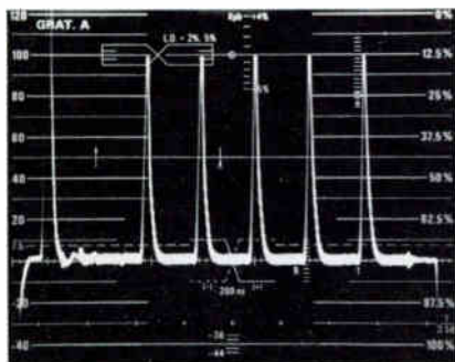
2. After passing through the staircase differentiator and chrominance filter, the CRT display shows spikes in proportion to the amplitude of the staircase risers.
