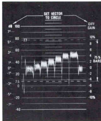
3. Depressing the DIFFERENTIAL PHASE button, the staircase chroma is positioned so that the reference point is on the 0° scale division. The peak of the signal corresponds to the differential phase error. In this photo, differential phase equals about 3°.
