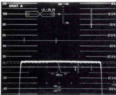
12. 3 full lines in duration, with serrations as shown here. 0.5 μsec/div, serration width = 4.5 μsec.
