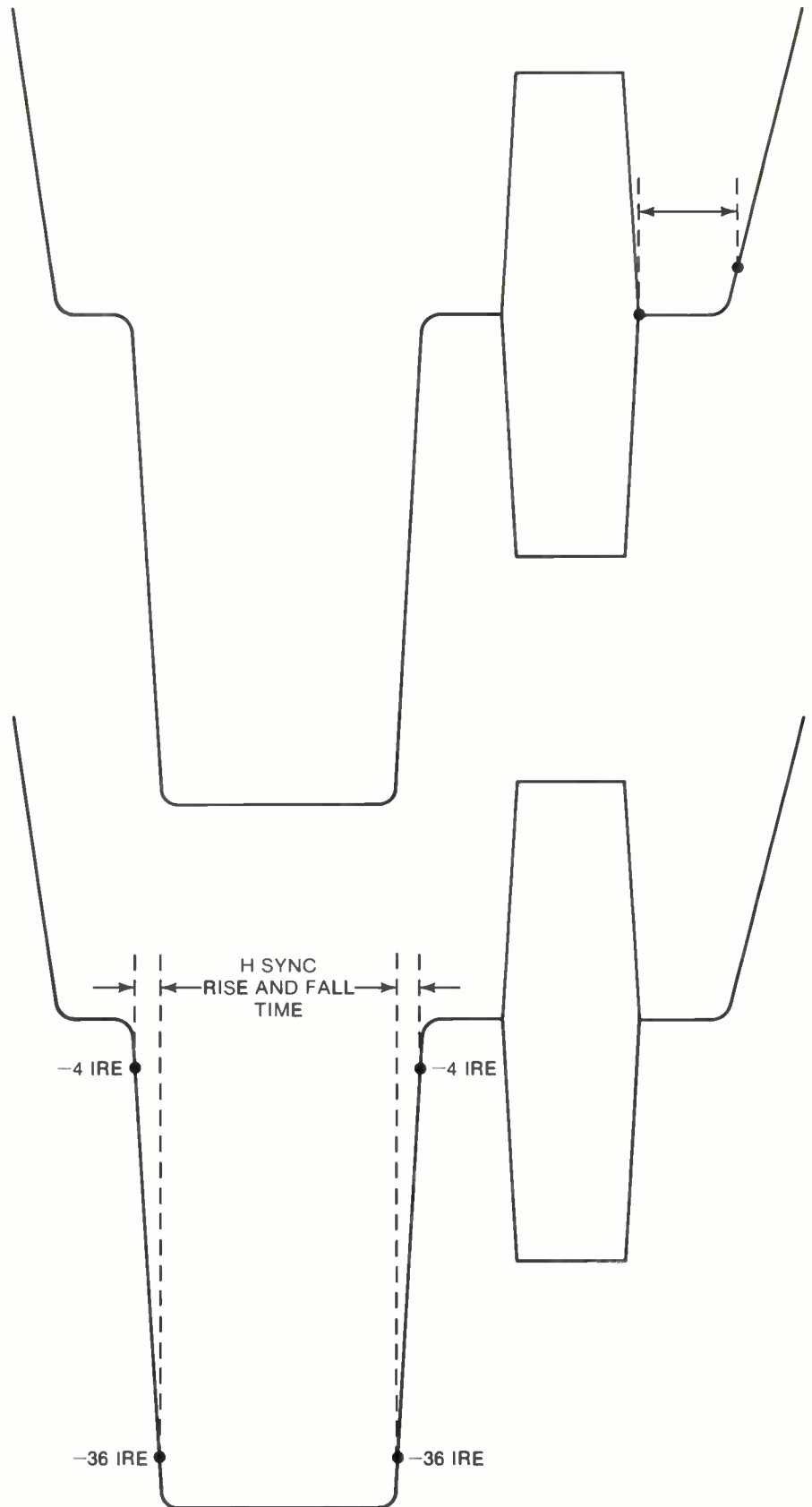
9. Shown here at 0.1 \mu sec/division. Sync pulse leading edge, 0.120 \mu sec, (Figure 9) sync pulse trailing edge 0.125 \mu sec.
