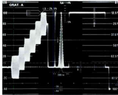
1. The modulated staircase is used to measure differential chroma gain.
