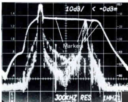
Figure 16. Sideband Response Using VIT Insertion
