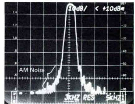
Figure 28. AM Noise on Aural Transmitter Due to Low Level Stages
