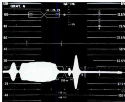
2. Off-air signal viewed with waveform monitor chroma bandpass filter.
