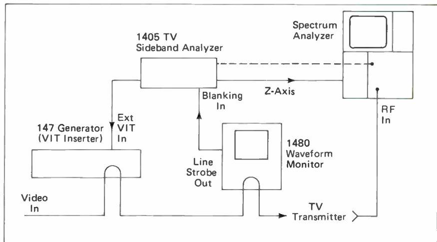
Figure 14. Sideband Analyzer Connections for VIT Insertion
