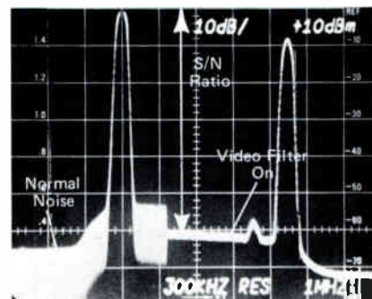
Figure 20. Display of Noise Measurement
