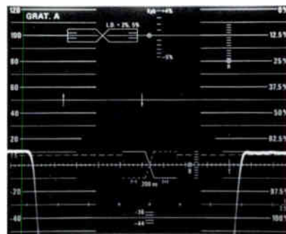
11. Measured between points at the 1/10 sync (-4 IRE) level. Shown here at 0.25 \mu\text{sec/div} : 2.40 \mu\text{sec} . Depending on the width of H sync, equalizers may be between 2.0 and 2.54 \mu\text{sec} .
