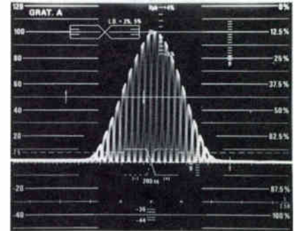
2. Undistorted modulated 12.5 T pulse.
