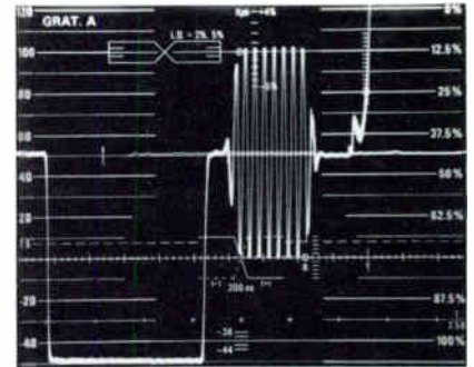
2. Reposition the signal so that burst extends upward from the 0 IRE scale division. Burst amplitude must be between 90 and 110 units on the scale. Burst shown here is about 2% high, which is well within specifications.
