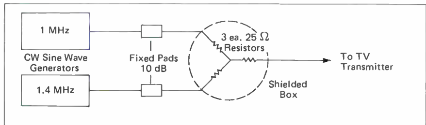
Figure 22. Combining Two CW Sine-wave Generators for Distortion Tests
