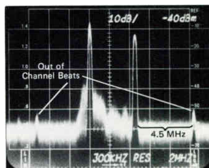
Figure 37. Out-of-Channel Sum and Difference Beats
