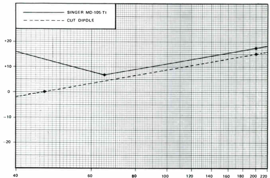
Figure 34. Correction Factors for Test Dipole
