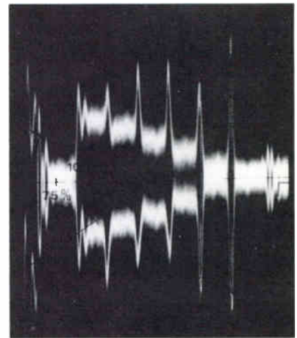
5. The CALIBRATED PHASE control is then adjusted to overlay the step being measured. The CALIBRATED PHASE dial now indicates the differential phase present. This method allows differential phase distortion as small as 0.1° to be measured.
