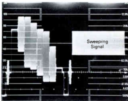
Figure 15. Waveform Monitor Display of VIT Interval Including Sideband Envelope
