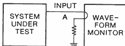
Synchronizing timing measurement setup.
