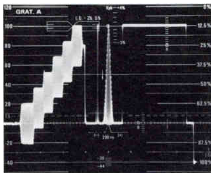
3. The staircase of the composite test signal may also be used for this measurement.
