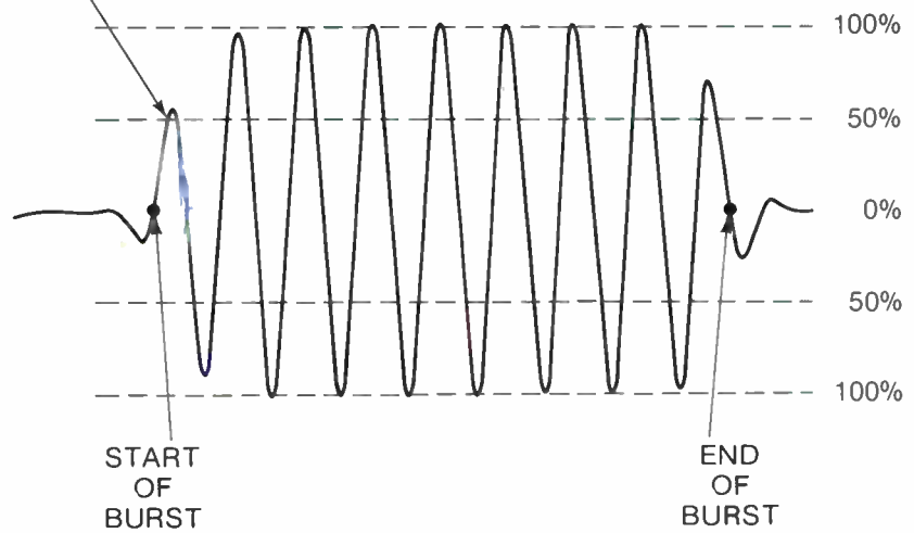
7. FCC standards require a minimum of 8 cycles of color burst. The burst shown here contains 8½ cycles.
