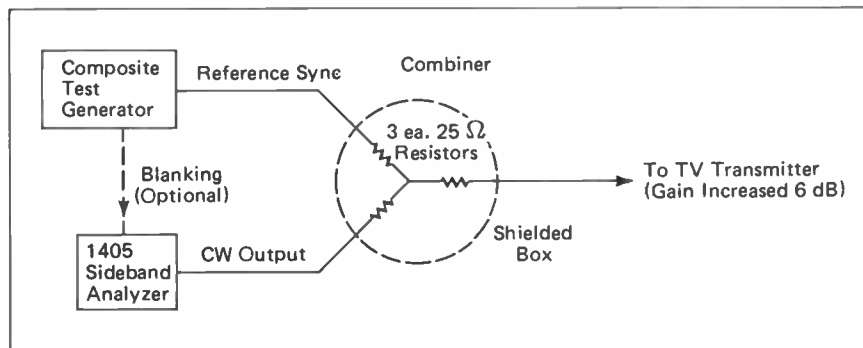
Figure 8. Combining CW Signal with Test Generator for Special Tests (See Text)
