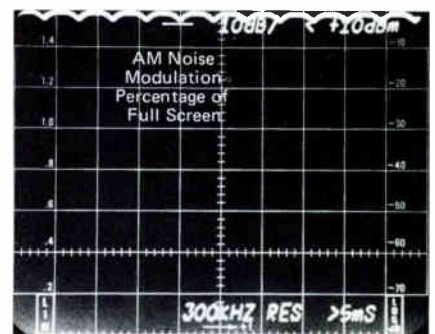
Figure 29. AM Noise on Aural Transmitter from Improper Tuning
