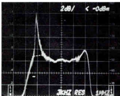
Figure 13. Low Level Sideband Response at 2 dB/Div
