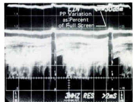
Figure 21. Linear Display of TV Waveform for Hum and Field Time Distortion Measurements
