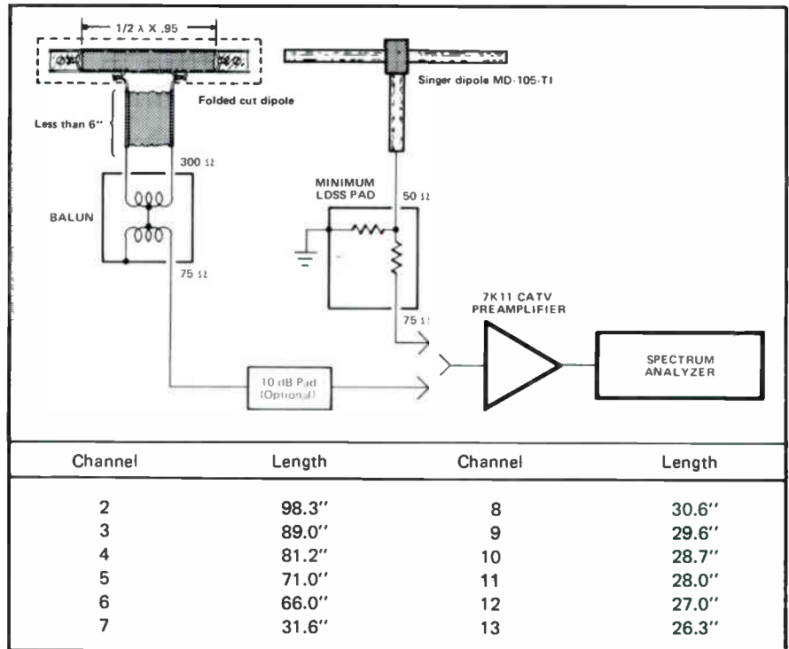
Figure 33. Constructing a Test Dipole
