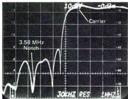
Figure 5. Lower Sideband and 3.58 Trap Tuning
