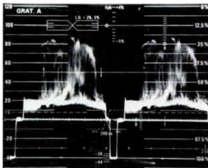
1. Picture black is separated from blanking by 9 IRE. Setup must be within the range of 5 to 10 IRE.
