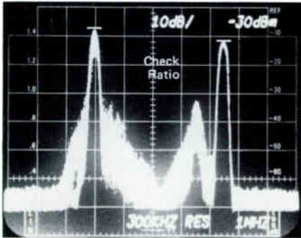
Figure 32. Checking the Picture-to-Sound Ratio
