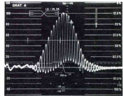
3. Modulated 12.5 T pulse from off the air feed. Pulse amplitude is first set to 100 IRE. Any aberration in the baseline indicates either CIL gain or delay distortion. The distortion can be evaluated by measuring the baseline disturbances and applying these values to the nomogram shown in figure 3A. In this photo, the baseline deviates to -10 IRE and +13 IRE. From the nomogram, chroma gain is -0.6 dB relative to luminance gain, and chroma is 220 nanoseconds ahead of luminance.
