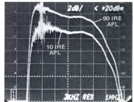
Figure 17. Transmitter Variations with 10 and 90 IRE Test Sweeps
