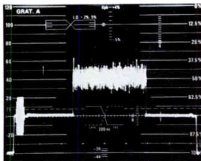
1. In noise measurement, a pedestal signal with noise is inserted by the noise measuring set. By adjusting the pedestal amplitude and noise level to match the video signal noise level, the system noise is measured.
