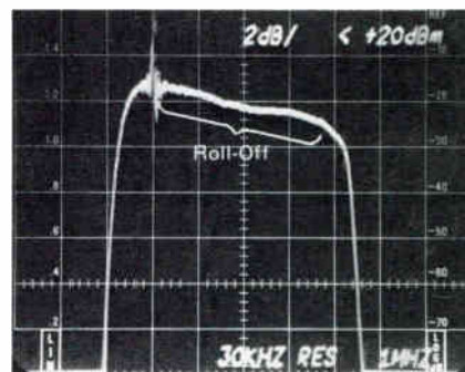
Figure 6. Transmitter Response at 2 dB/Div (Note Response Rolloff of about 2 dB)
