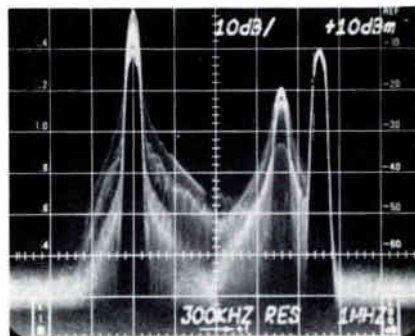
Figure 19. Spectrum Analyzer Display of TV Signal
