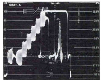
3. The comparison of pulse to bar amplitude is simplified by the sweep foldback feature of the TEKTRONIX 1480 Waveform Monitor.
