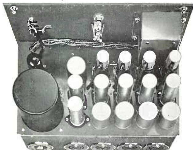
OP-7 chassis, rear view. Four microphone receptacles and output receptacle are provided.
