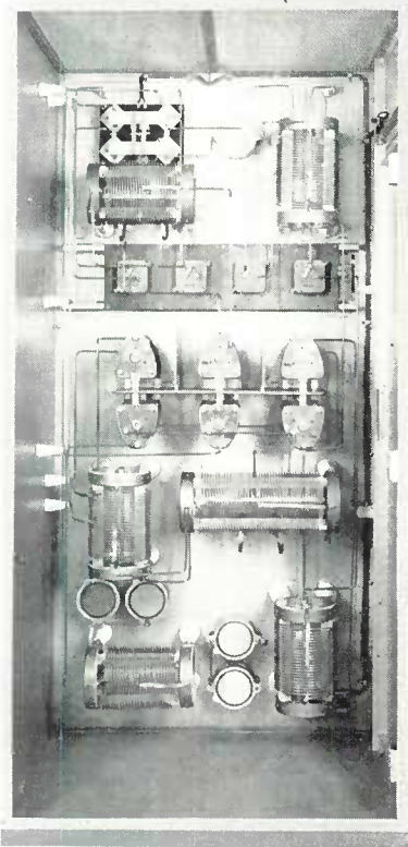
Interior rear view of a 5 KW phasing and branching equipment housed in MI-7485-F left wing extension cabinet
