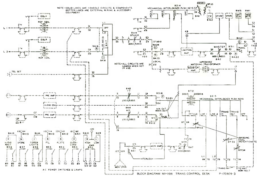
Block Diagram MI-II616 Transmitter Control Desk
