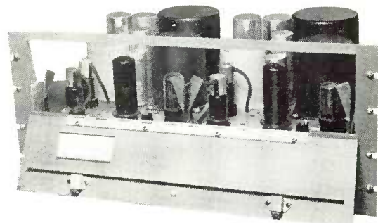
Panel open showing two BA-3A amplifiers
