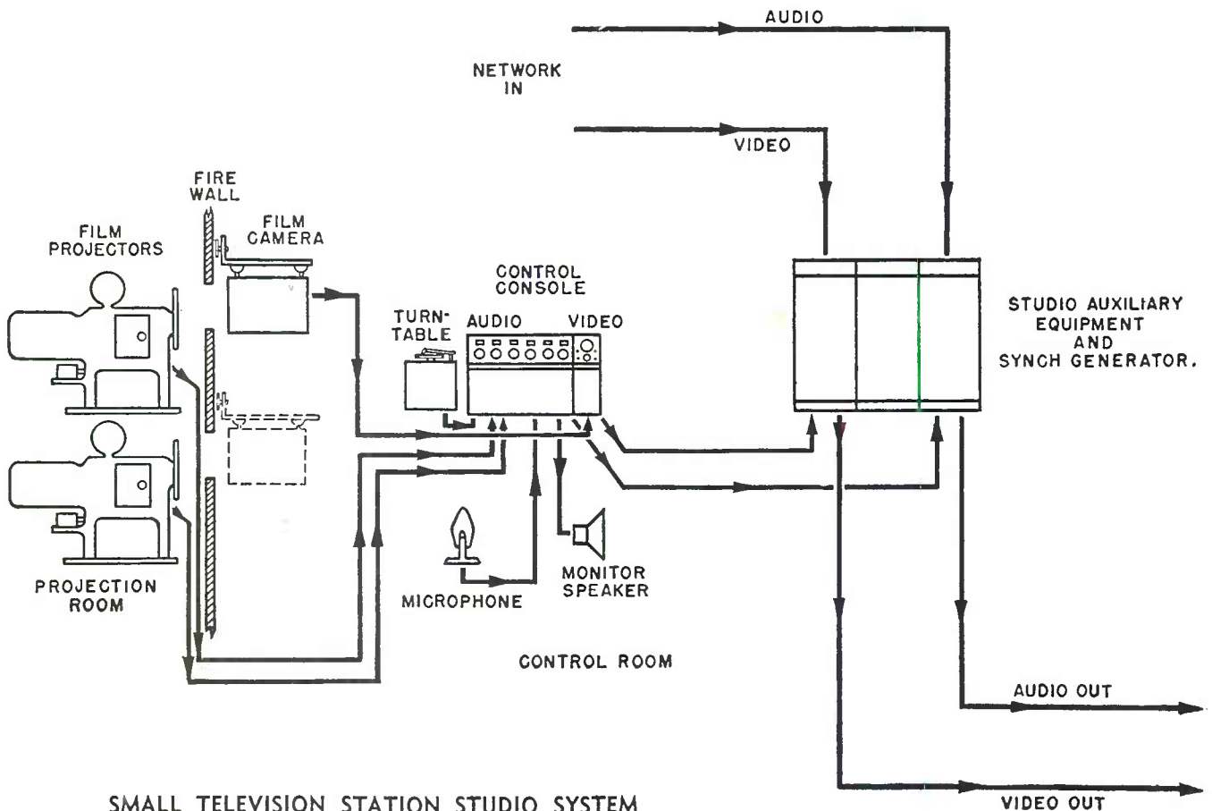
SMALL TELEVISION STATION STUDIO SYSTEM
