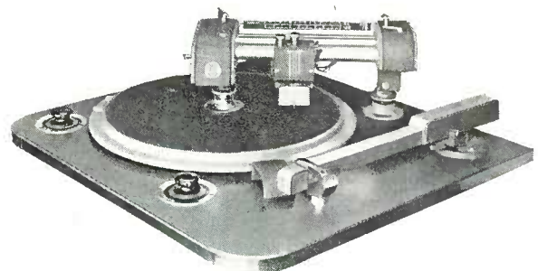
70-D Turntable with 72-D Recording Attachment in position
