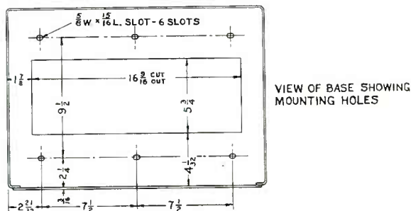
Outline Dimensions of 9-AX Cabinet Rack
