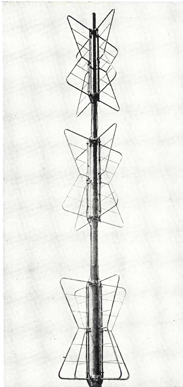
Three Section Super Turnstile. The center pole is self-supporting and may be mounted on top of a suitable building, mountain or a supporting tower similar to that used for standard band broadcasting antennas.
