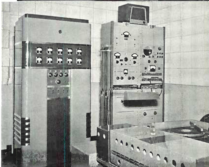
Control room at WMRN, Marion, Ohio, showing 250 watt transmitter, turntables, control console, and associated audio and test equipment.
