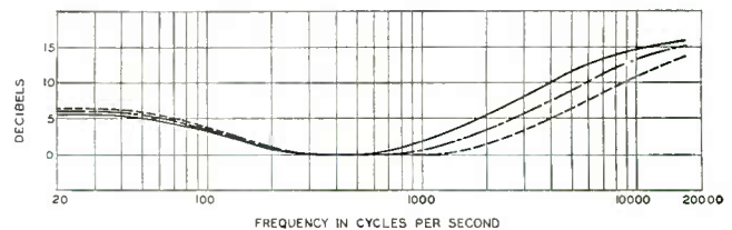
FREQUENCY RESPONSE CURVES OF A TYPICAL BA-5A AMPLIFIER WITH COMPENSATION
