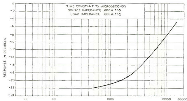
Frequency response of MI-4926-A
