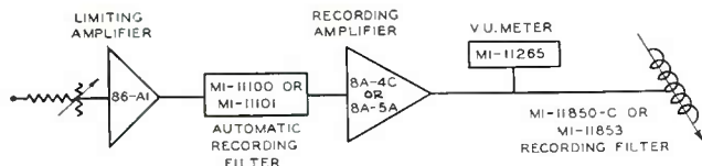
Fig. 2. This diagram illustrates a recording technique using the automatic recording filter only (or "flat").
