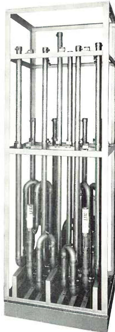
Triplexer with all covers removed to show system of tunable coaxial lines. Two output connectors are made near the bottom, as shown. The two input lines are at the rear and are not visible.
