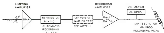
Fig. 3. This arrangement is included for recordists who choose to use both "automatic" and NAB orthacoustic compensation.
