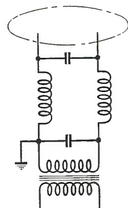
Isolation Circuit (Single Choke) with MI-7014 Isolation Transformer
