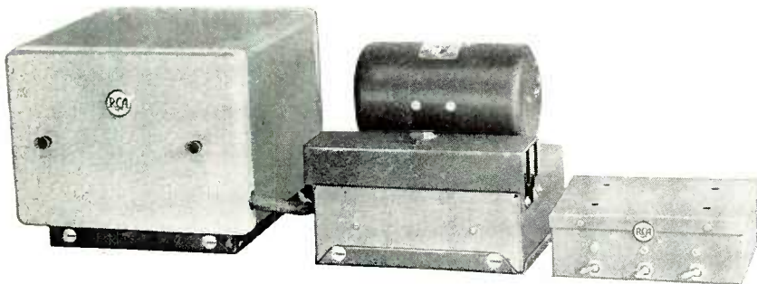
MI-7824—22-watt mobile UHF transmitter — is operated from 6-volt battery. Features: Crystal Control, automatic Modulation Control, minimum size and weight.
