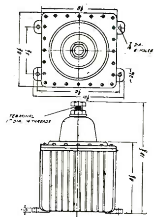
Casing 361 A
