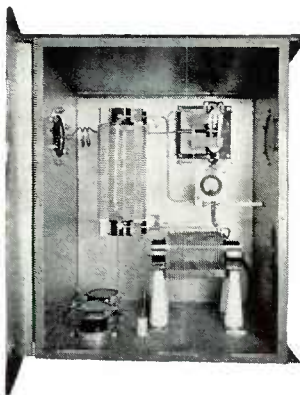
Line Terminating Unit MI-7485 enclosure. Open
