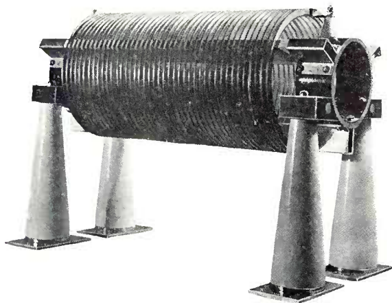
MI-7487 125 mh Inductor
