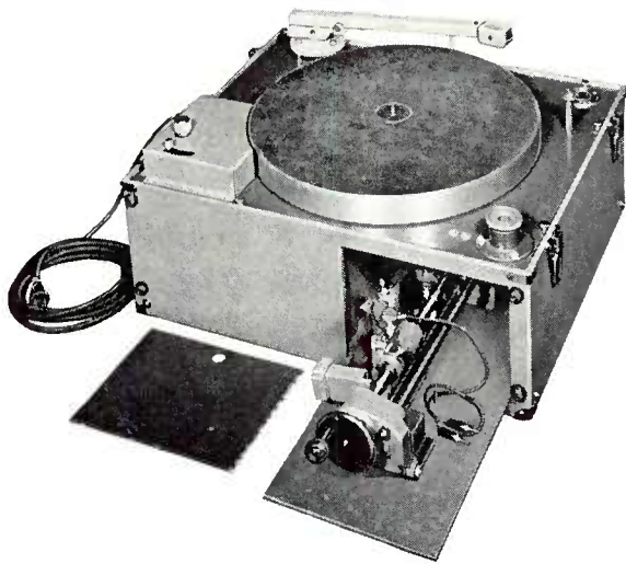
Showing method of mounting recording attachment while transporting unit.
