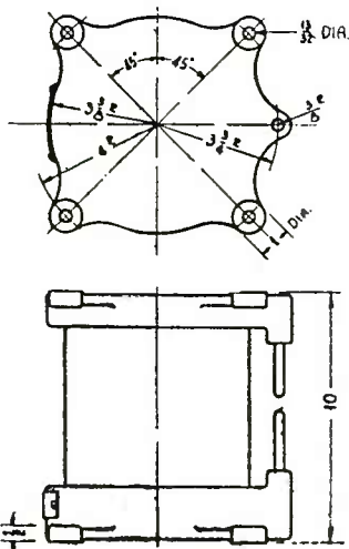
Casing 140
