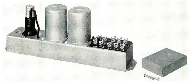
85-B Preamplifier with terminal board cover removed
