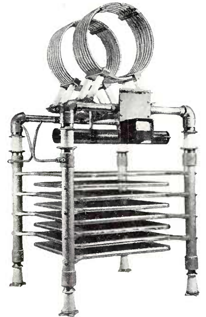
50 KW Line Terminating Unit Built for KWKH
