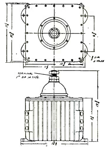
Casing 358
