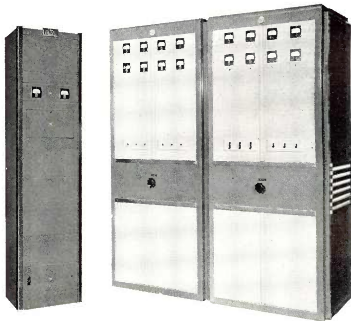
The FM-1-A Frequency Modulated Broadcast Transmitter is designed for high fidelity FM broadcasting and other special communication services in the 26 to 108 megacycle frequency range such as high fidelity television sound, facsimile broadcasting, educational broadcasting and similar UHF services, utilizing either FM or AM operation.
