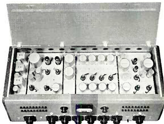
76-B2 with Top Raised
