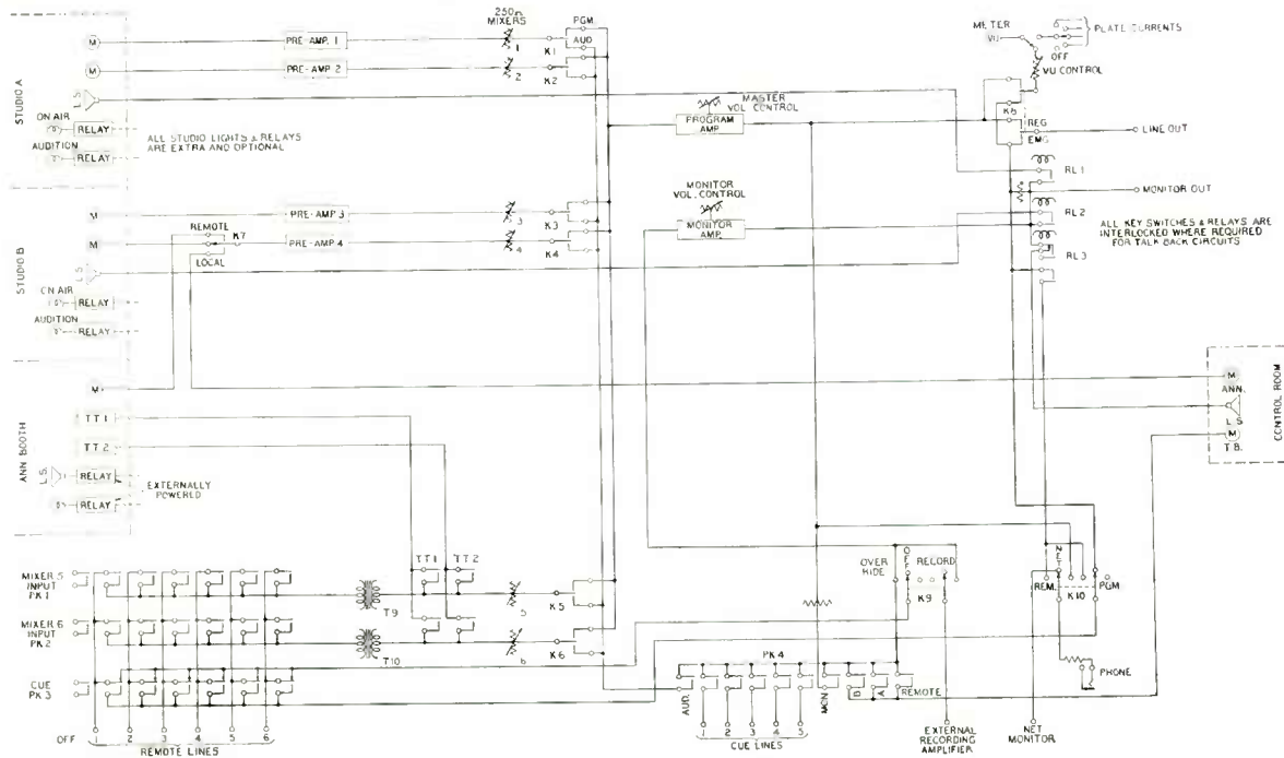
SIMPLIFIED BLOCK DIAGRAM OF 76B2 CONSOLE
