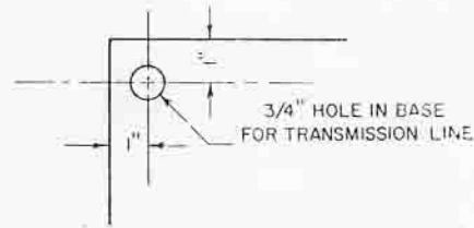
DETAIL I
