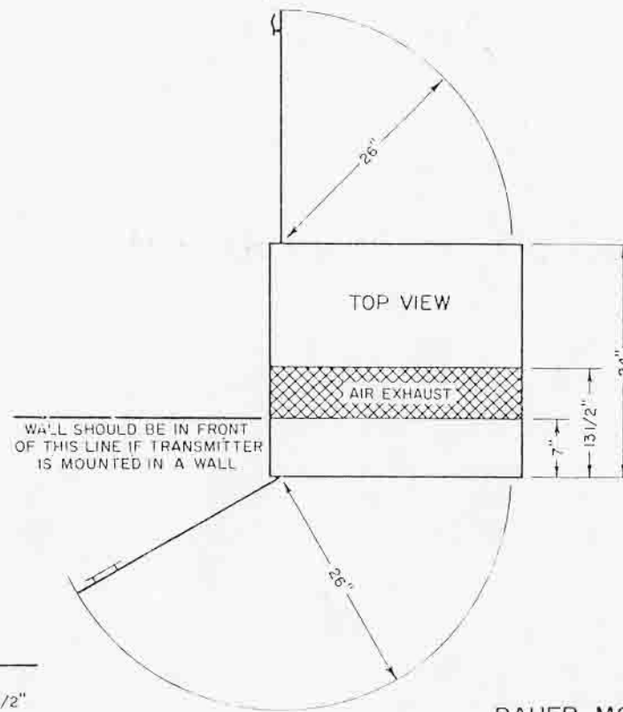
BAUER MODEL 707 AM BROADCAST TRANSMITTER
