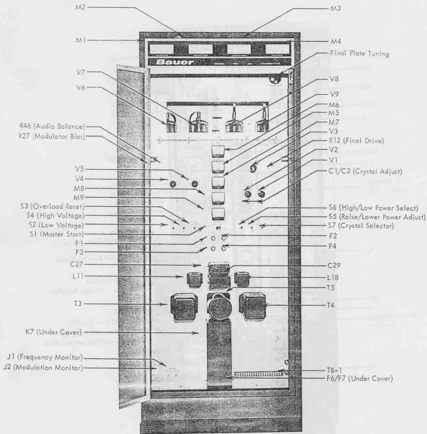
FRONT VIEW OF BAUER MODEL 707 BROADCAST TRANSMITTER
