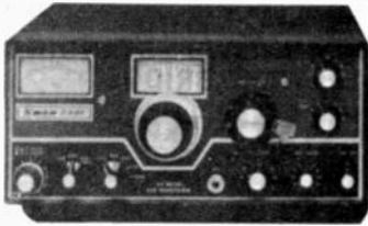
NEW SWAN 250C 6 METER SSB-CW-AM TRANSCEIVER
